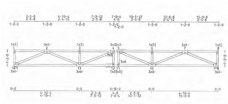
Figure 6.2. — Parallel chord truss design.
