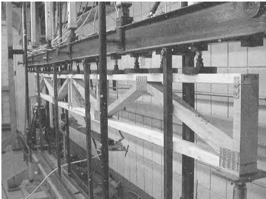
Figure 6.4. — Parallel chord truss testing setup.
