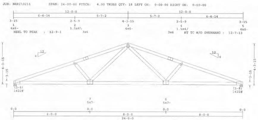
Figure 6.1. — Pitched chord truss design.
