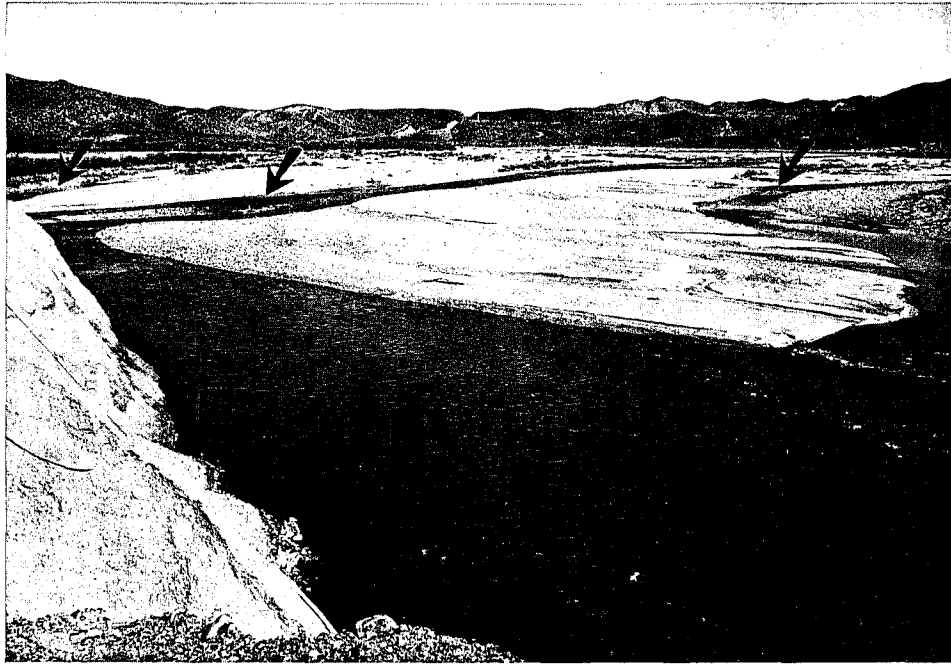
Figure 17.—Heavy sediment loads in this Salt River reach above Roosevelt Reservoir, Arizona, created a wide bed with shallow flow depth. Thus, stream competence (sediment-carrying capacity) was drastically reduced. To increase flow depth (and competence), the flow split into several channels (arrows). Flow in the foreground is from left to right.
