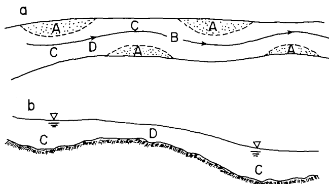
Figure 9.—(a) Schematic plan view of alternating bars (A) and thalweg (B) in a straight channel reach, and section view of the associated longitudinal profile (b) showing pool (C) and riffle formations (D). Riffles form at crossings of the thalweg between bends.
