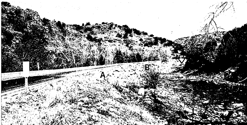
Figure 22. —(a) In mountain country, highway construction often infringes on streams. A relatively large meander bend (A) of Sycamore Creek, central Arizona (flowing from left to right), was cut off and the streambed relocated to the opposite side of the road (B). Thus streamlength was shortened, slope gradient steepened, and a nickpoint introduced at (D) that led to the development of a bedscarp in the volcanic bed rocks. This scarp advanced about 300 feet upstream (C) within approximately 25 years. At (D), the original meander bend connected with a short straight reach still used by the creek. (b) Closeup view of the 8-foot-deep bedscarp (arrow). Adjustment processes not only caused a bedscarp but also tried to reestablish the meander, endangering the road bed by undercutting. (c) Rock riprap bank protection was required between A and B to protect the road. Arrow signifies bedscarp location.
