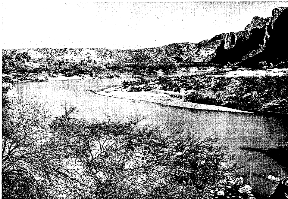
Figure 6.—Point bar in Salt River north of Phoenix, Ariz. Flow is from left to right in the foreground. Note the pointed downstream bar end.
