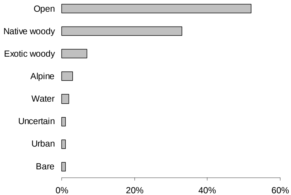
Fig. 1 Aggregated land cover classes of New Zealand (LCDBII)
