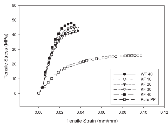
Figure 3 Stress–strain curves of various hybrid and nonhybrid composites.
