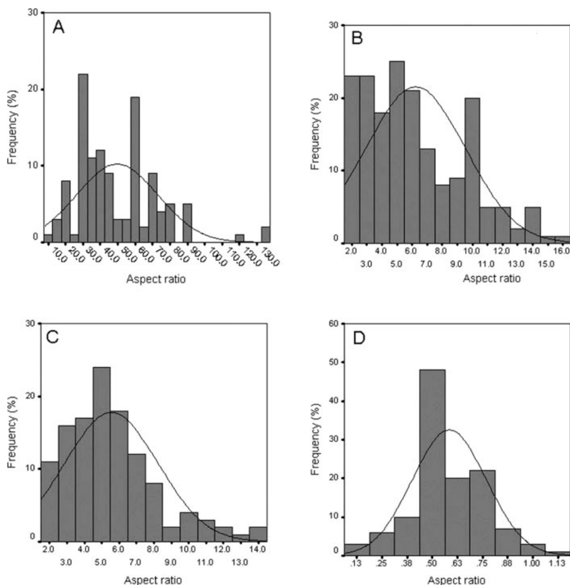
Figure 1 Frequency distributions of the aspect ratios of kenaf fibers and wood flour: (A) kenaf fiber before processing; (B) kenaf fiber after processing; (C) wood flour before processing; and (D) wood flour after processing.
