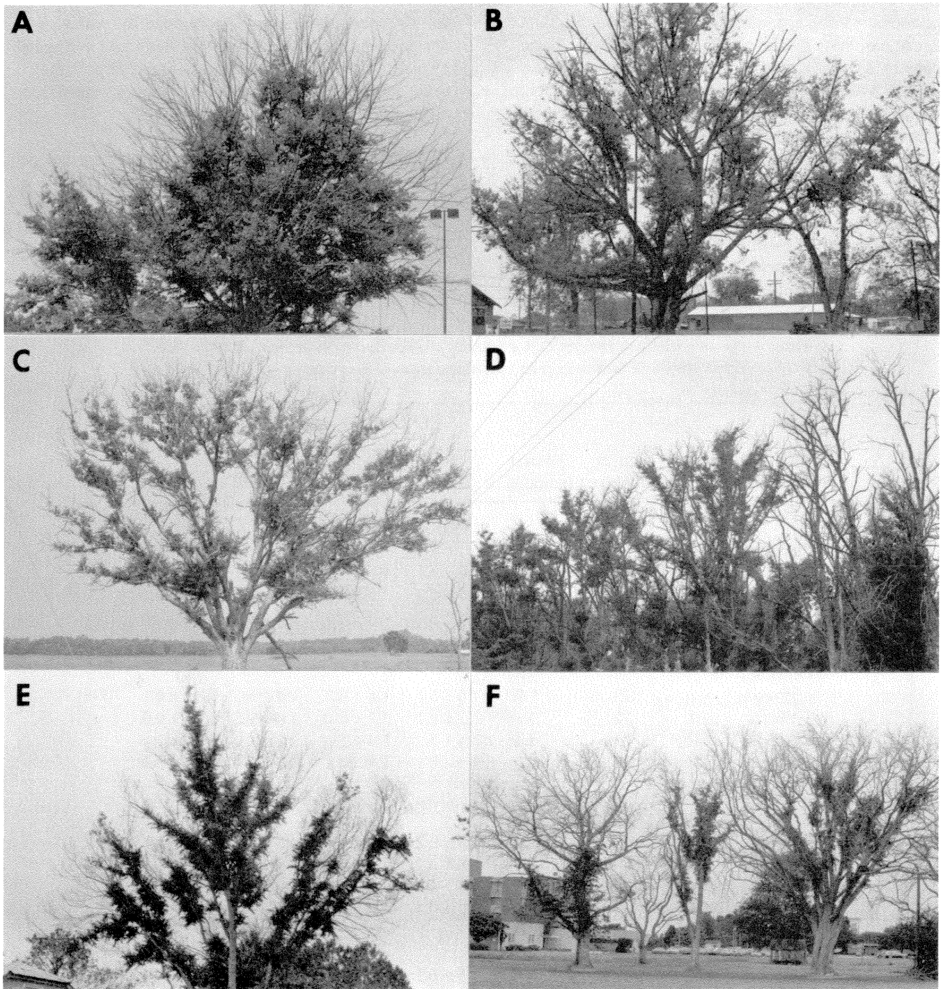
Figure 2—Symptoms of sugarberry dieback and decline observed in southern Louisiana. (A) Twig and branches with bare ends following defoliation, (B) breakage of branches following defoliation, (C) epicormic sprouts and suckers along the main branches and trunk of a tree in an open field, (D) dieback and epicormic branching of sugarberry trees in a woodland setting, (E) twig dieback and epicormic branching of a sugarberry tree in a residential yard, and (F) water sprouts arising along large branches and trunks of large trees.
