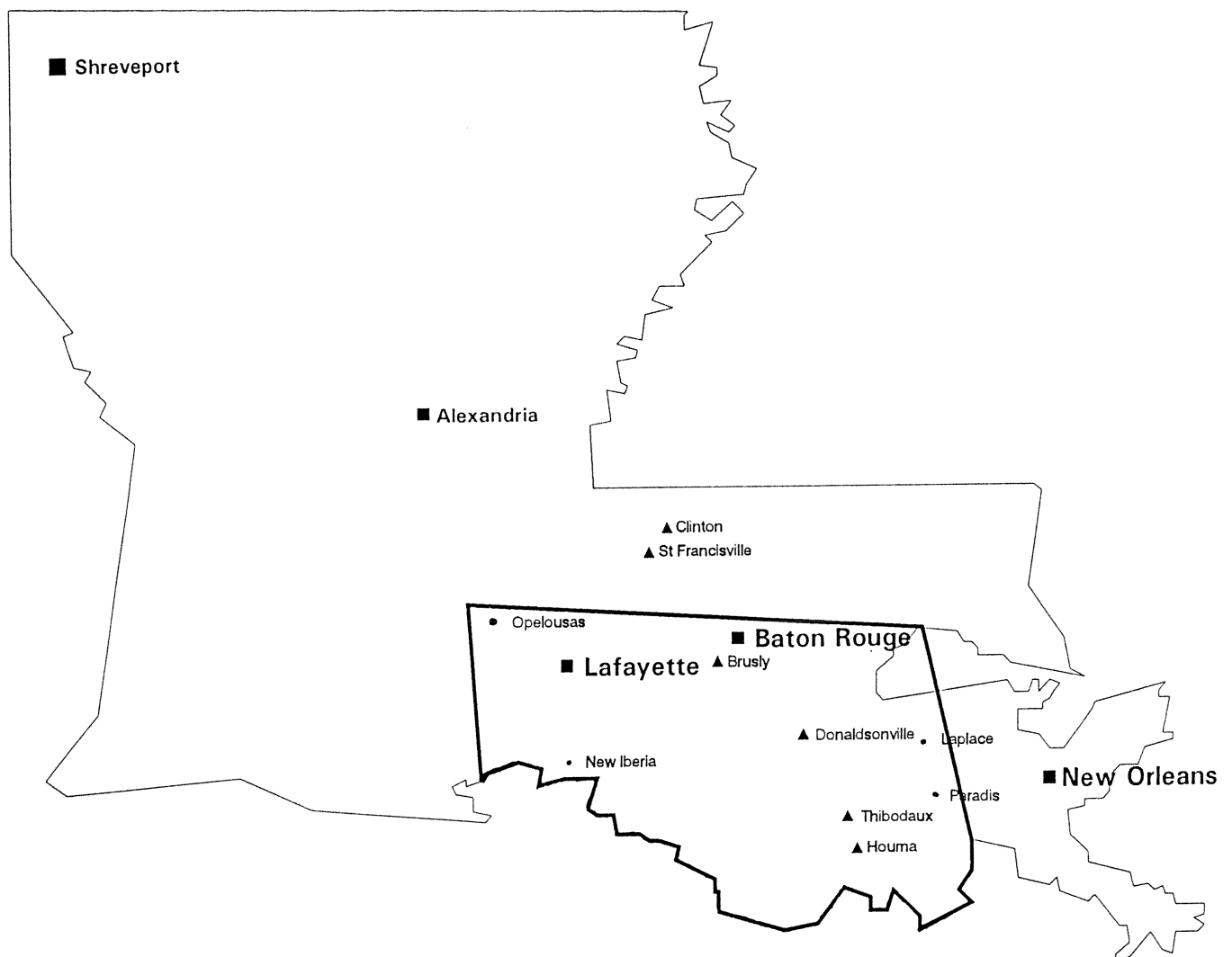
Figure 1—Area in southern Louisiana affected by sugarberry decline during and after the 1988-89 dieback episode.
