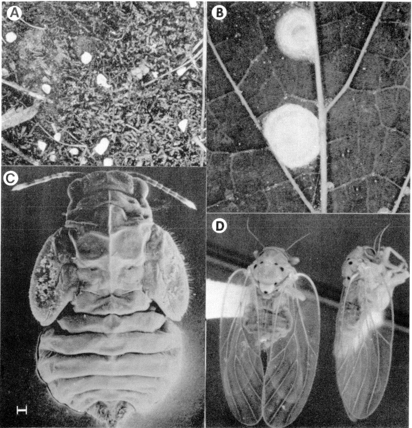
Figure 4—Observed life stages of psyllid, Tetragonocephala flava . (A) White tests (coverings) resting on leaves in litter on the forest floor; (B) closeup of nymph tests (on the underside of sugarberry leaf); (C) scanning electron micrograph of nymph, scale bar = 0.1 \mu M, \times 41 magnification; and (D) adults of psyllid.
