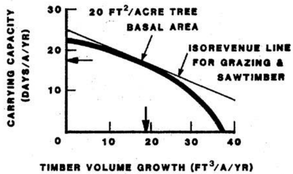
Figure B --Optimum thinning intensity when considering grazing and current sawtimber prices.
