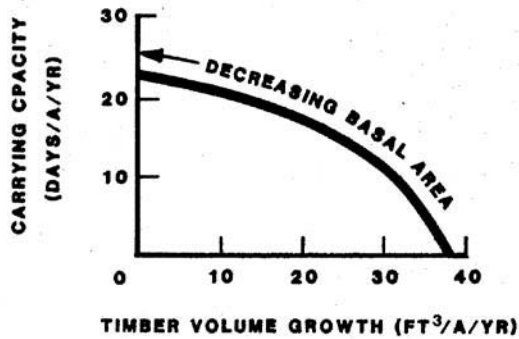
Figure A.--Production possibilities frontier for livestock grazing and wood growth.
