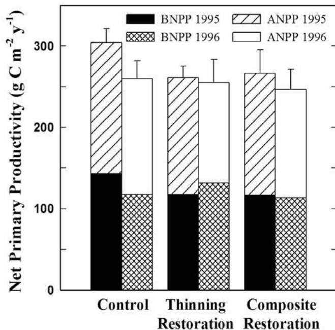
Figure 9. Total net primary production (NPP) in untreated control, thinning restoration, and composite restoration treatments. Bars depict means \pm 1 SE ( n = 5 plots). There were no significant differences among treatments in aboveground NPP (ANPP), belowground NPP (BNPP), or total NPP for individual years or repeated-measures ANOVA ( P > 0.10 ). From Kaye and others (2005).
