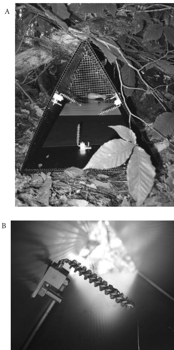
Figure 6.8. Triangular marten cubby (with track plate) installed on the ground, showing (A) the placement of gun brushes serving as hair collection devices, and (B) a close-up of a gun brush mounted on a mechanical lug (with fisher hair). Photos by P. MacKay.
