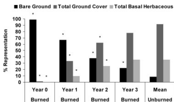
Figure 2. Percentage bare ground, total ground cover, and total basal herbaceous cover on burned and unburned hillslopes immediately following fire and 1, 2, and 3 years after fire. An asterisk above the burned value indicates significant differences ( P < 0.05 ) in burned and unburned values for the respective cover type and year
