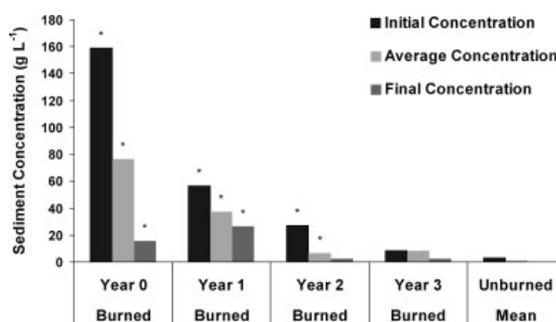
Figure 5. Initial, average, and final sediment concentrations measured on burned and unburned hillslopes during overland flow simulations at inflow rate 15 l min -1 . Means presented here only depict concentrations for plots that generated runoff. An asterisk above burned value indicates significant differences ( P < 0.05 ) in burned and mean unburned values for the respective year
