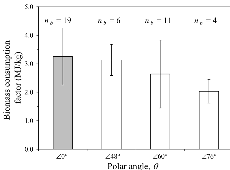
Figure 10. Mean ratio of FIRE to total mass loss categorized by polar angle. Radiative measurements at 48^\circ , 60^\circ , and 76^\circ were taken with the TVS-8500. Radiative measurements at the zenith were taken with the AGEMA-550 and were corrected by the ratio of FIRE_{AGEMA} to FIRE_{TVS} determined during the collocated sensor-to-sensor cross calibration.
