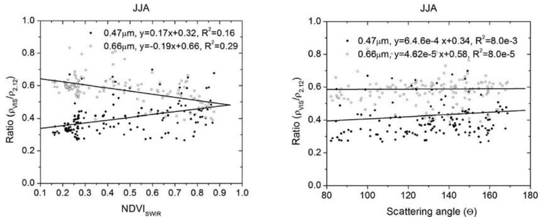
Figure 6. Scatterplot of the reflectance ratios (VIS/SWIR) versus the (left) NDVISWIR and (right) scattering angle.
