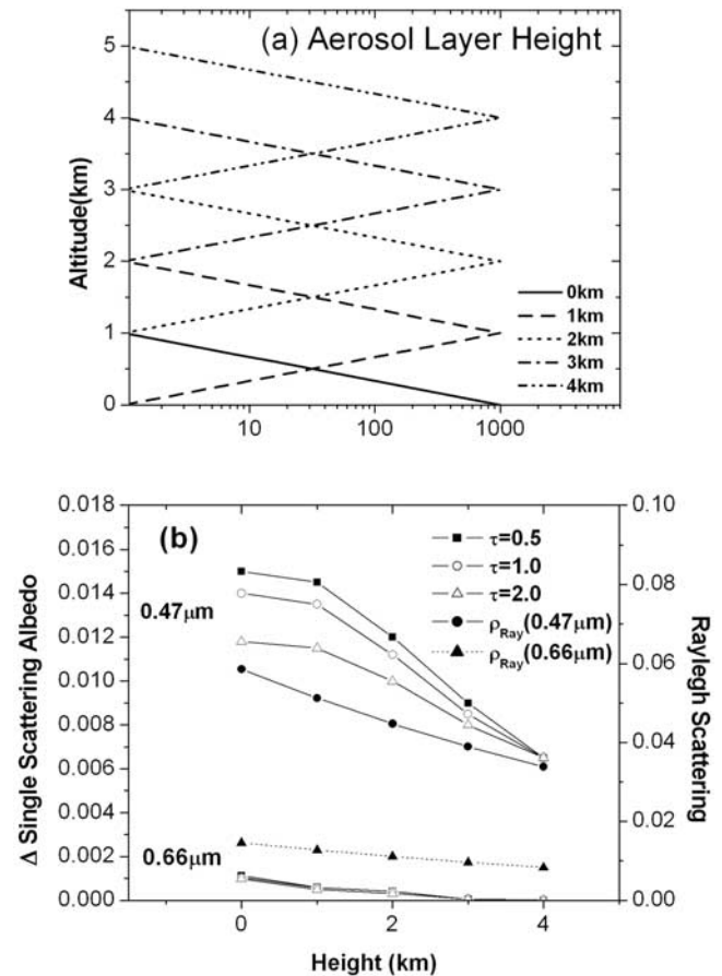
Figure 8. (a) Five assumed vertical distributions of absorbing aerosol layers (AAL). (b) Dependence of the errors in SSA ( \Delta\omega_0 ) at 0.47 \mu\text{m} and 0.66 \mu\text{m} and Rayleigh scattering, as a function of height, for three AOT values.
