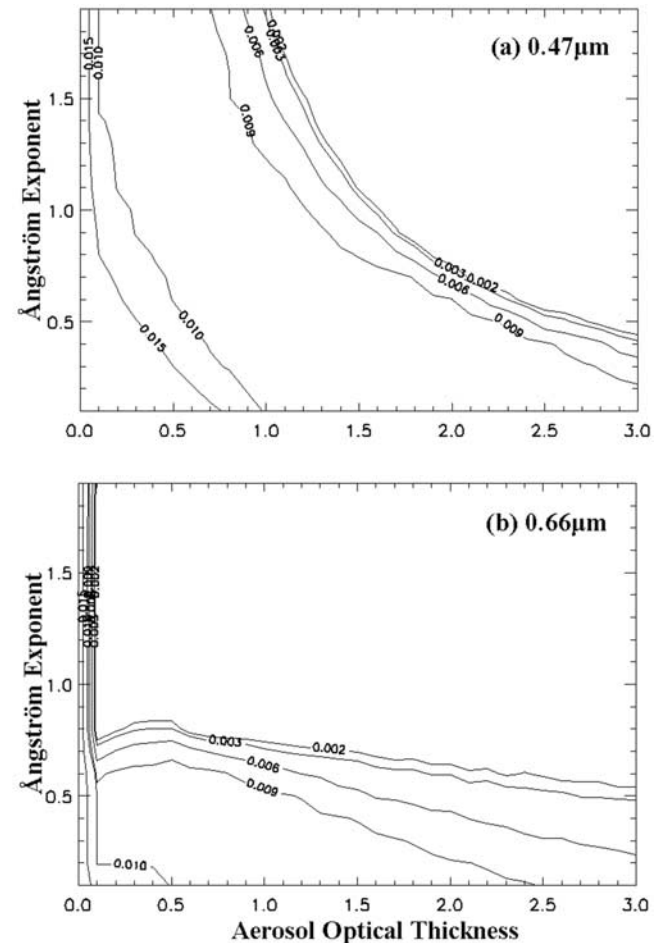
Figure 6. Errors in SSA ( \Delta\omega_0 ) due to a 10% change in the Ångström exponent at (a) 0.47 \mu\text{m} and (b) 0.66 \mu\text{m} channels.
