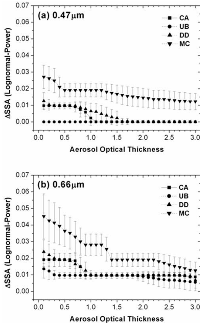
Figure 4. Differences in SSA ( \Delta\omega_0 ) at (a) 0.47 \mu\text{m} and (b) 0.66 \mu\text{m} between the lognormal and Junge power law size distributions. The Ångström exponents, as a Junge distribution parameter ( \nu ) for each aerosol model, are 1.42 (CA), 1.43(UB), 0.17(DD), and 0.08(MC), respectively [Hess et al. , 1998].
