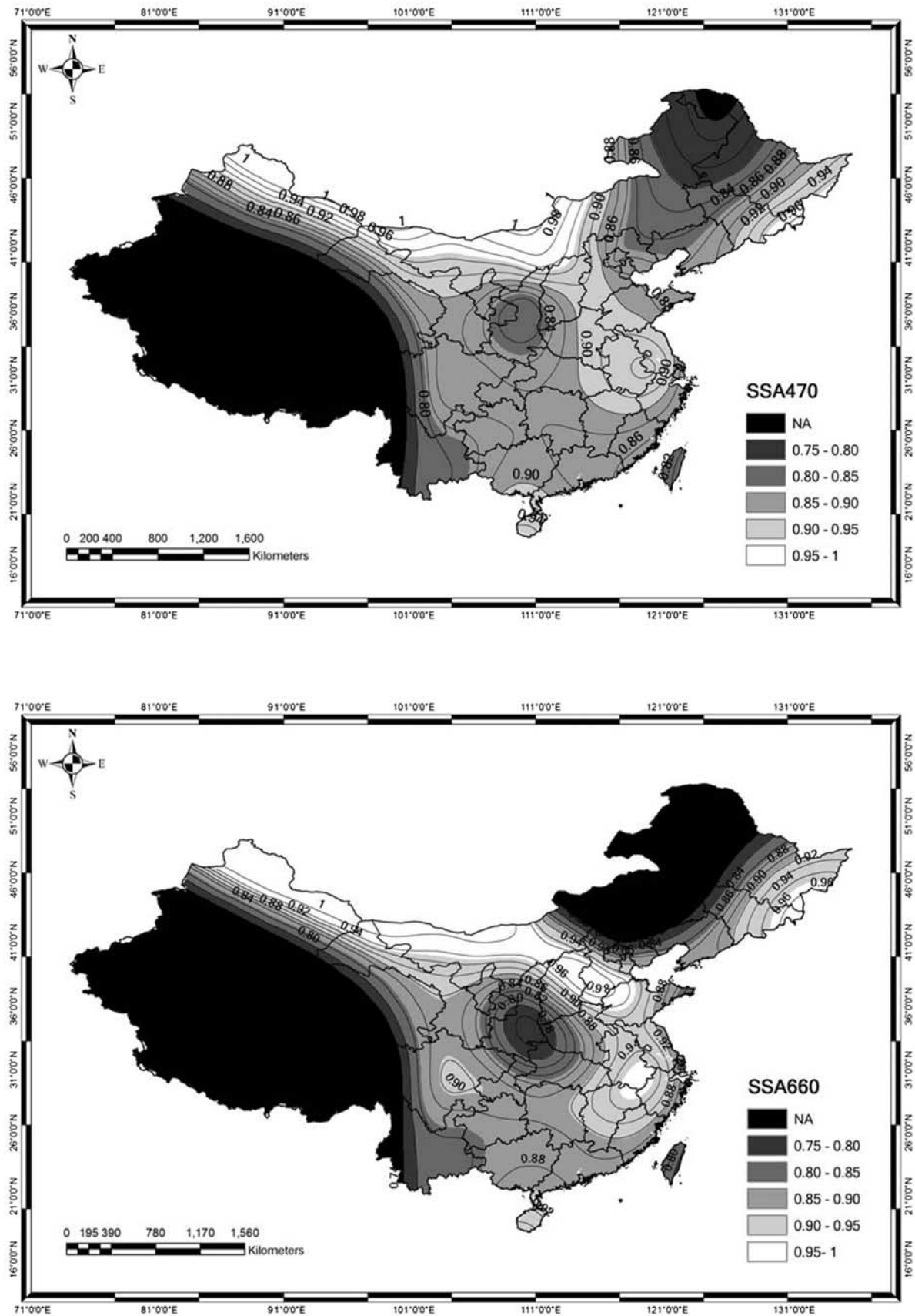
Figure 13. Spatial distribution of retrieved SSA at 0.47 \mu\text{m} and at 0.66 \mu\text{m} over the study area.
