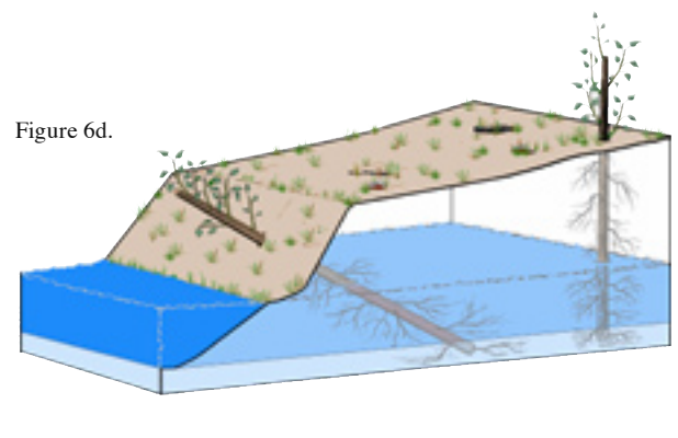
Figures 6a, 6b, 6c, and 6d—Streambank bioengineering uses dormant non-rooted hardwood cuttings for a variety of treatments: brush mattress (6a), wattle (6b), vertical bundle (6c), and pole plants (6d).—Illustrations by Steve Morrison, reprinted from Riparian Zone Reforestation: Field Requirements and Nursery Opportunities by J. Chris Hoag and Thomas D. Landis (2001), Native Plants Journal 2 (1): 30–35. Used with permission from Native Plants Journal, Inc.
