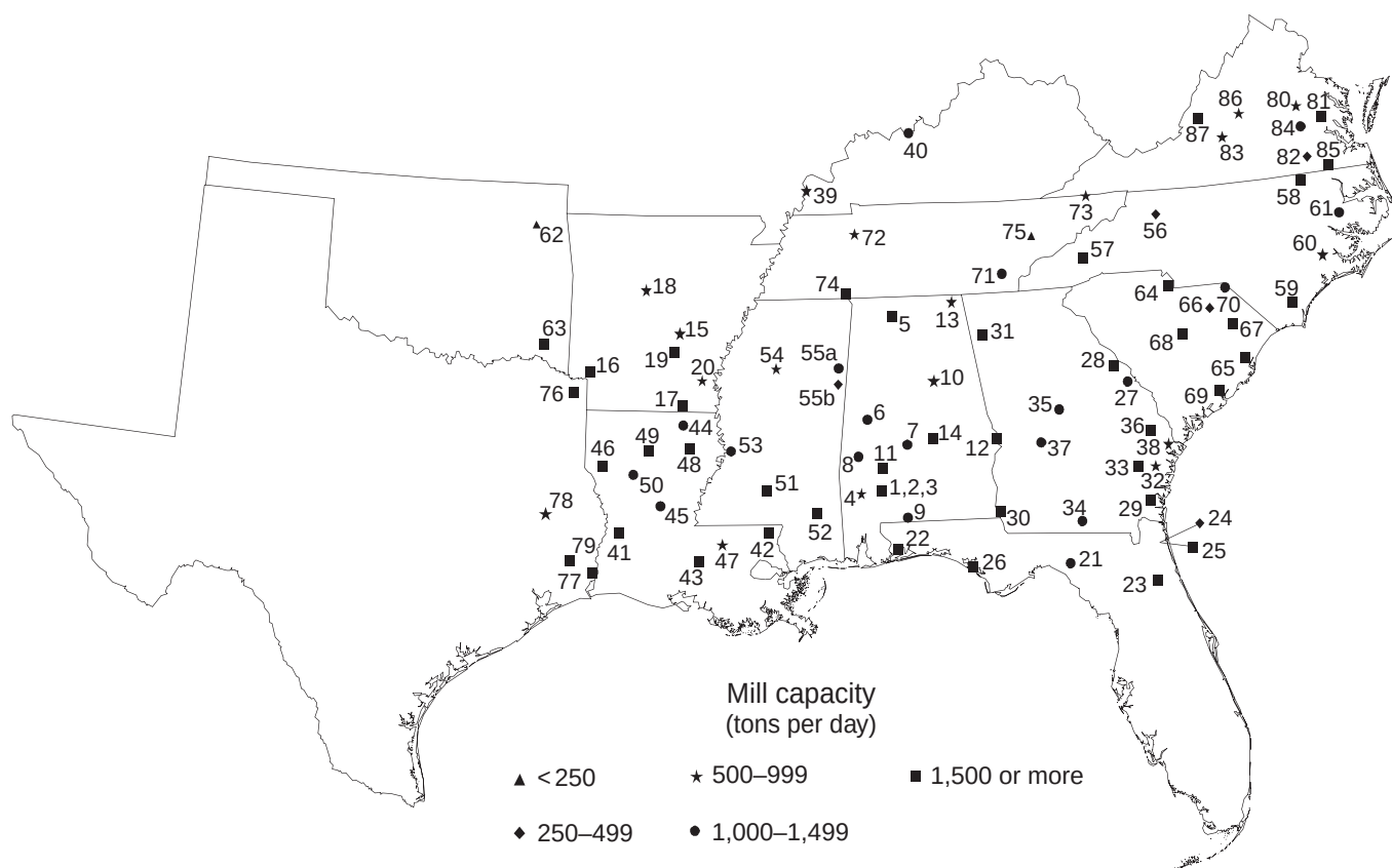
Figure 7—Capacity of southern pulpmills operating and drawing wood from the 13 Southern States, 2007. Numerals are coded on Table A.22.
