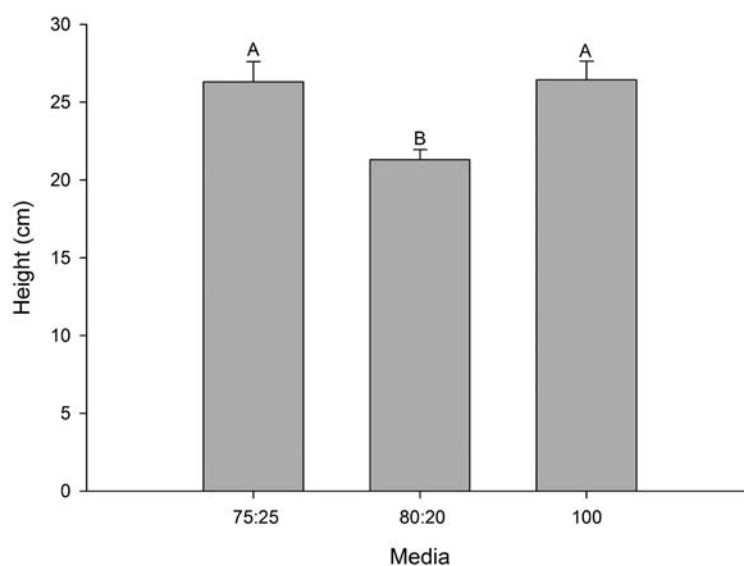
Figure 3. Height of western larch seedlings grown for 105 days in three media mixes (75:25 = 75% peat, 25% fine screened Douglas-fir bark by volume; 80:20 = 80% peat, 20% fresh Douglas-fir sawdust by volume; 100 = 100% peat). Different letters indicate significant differences at \alpha = 0.05 .
