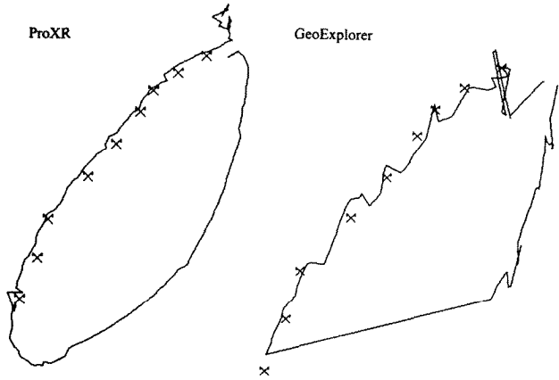
Figure 3. Photograph and map of heavy canopy test conditions with example plots of GPS-based skidder paths in that test condition. Data were collected at the low travel speed
