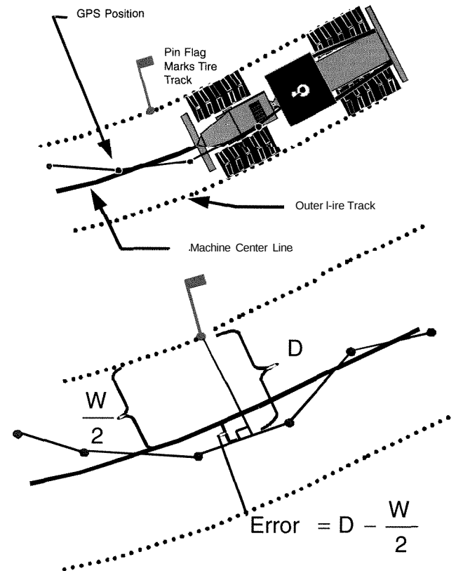
Figure 4. Graphical representation of procedure used to determine GPS position error.
