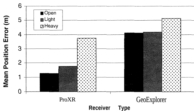
Figure 5. Mean GPS position errors for different receiver types and canopy conditions
