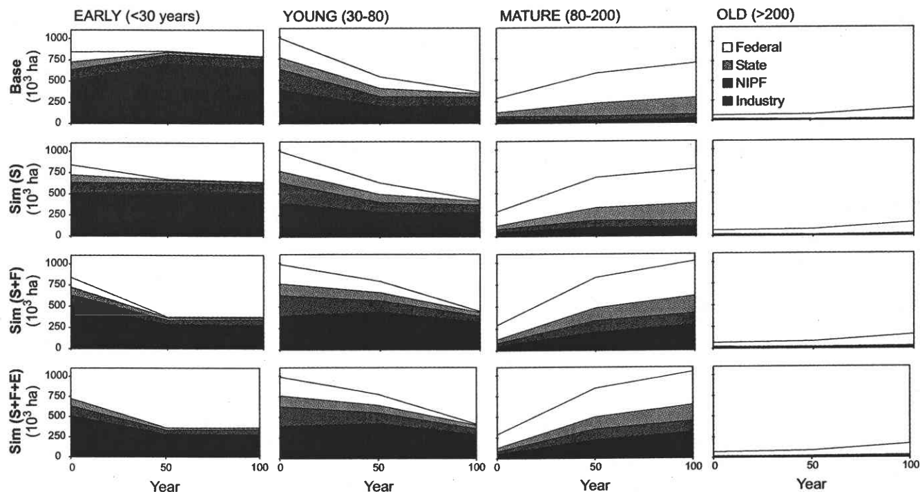
Fig. 4. Forest inventory by ownership group and age-class throughout the 100-year LAMPS policy simulations.
