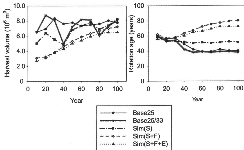
Fig. 2. Industrial harvest volumes and rotation ages throughout the 100-year LAMPS policy simulations.
