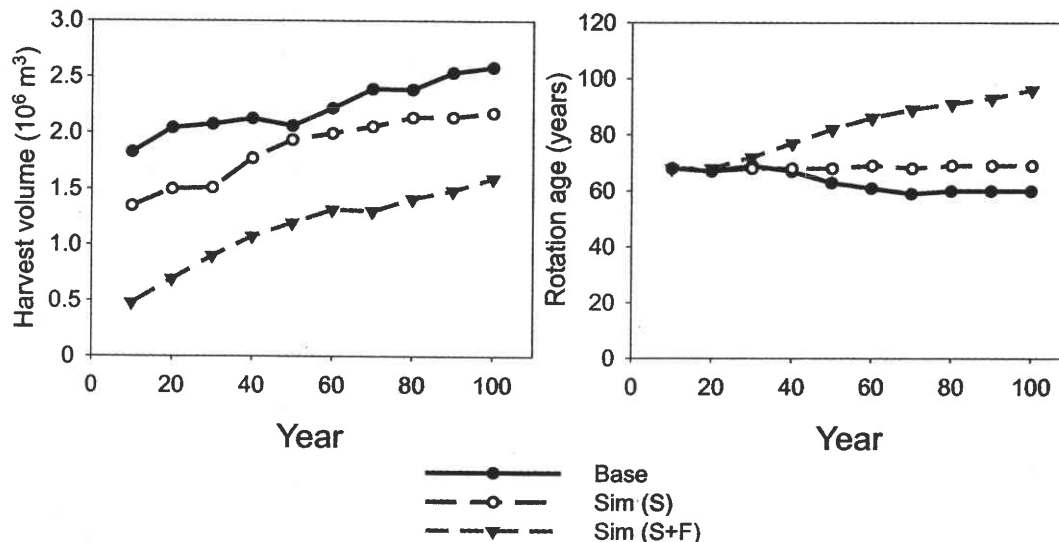
Fig. 3. Nonindustrial harvest volumes and rotation ages throughout the 100-year LAMPS policy simulations.
