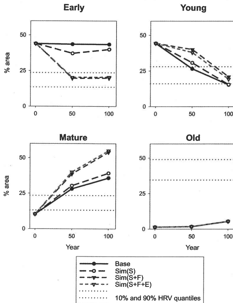
Fig. 5. Relative area in each age-class throughout the 100-year LAMPS simulations. Dotted lines represent the estimated historical range of variability (HRV) established from the Landscape Age-class Demographic Simulator (Wimberly 2002).
