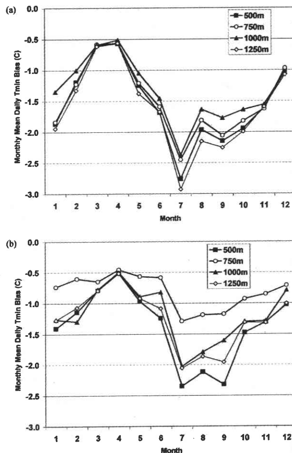
FIG. 9. PRISM bias (predicted - observed) of daily minimum temperature for stations (a) SGO and (b) MMO at four different inversion-height parameterizations ranging from 500 to 1250 m, averaged for each month in 2003.
