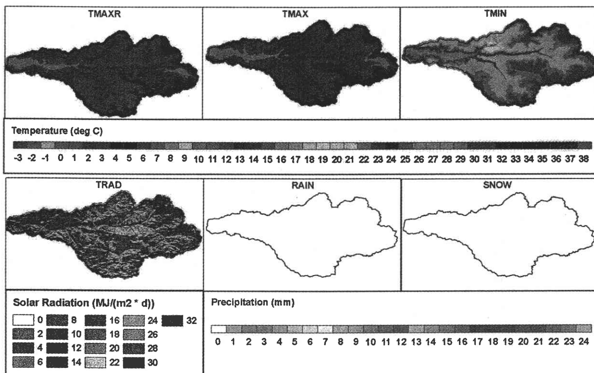
FIG. 12. As in Fig. 10, but for 29 Jul 2003.
