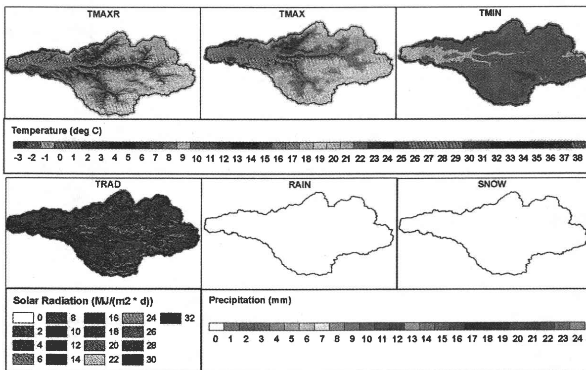
FIG. 13. As in Fig. 10, but for 4 Oct 2003.
