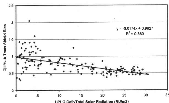
FIG. 7. Relationship between ratio of Gill to HJA shield daily maximum temperature bias [(\text{Gill} - \text{aspirated})/(\text{HJA} - \text{aspirated})] and daily total solar radiation observed at UPLMET for 7 Jul–31 Dec 2003.
