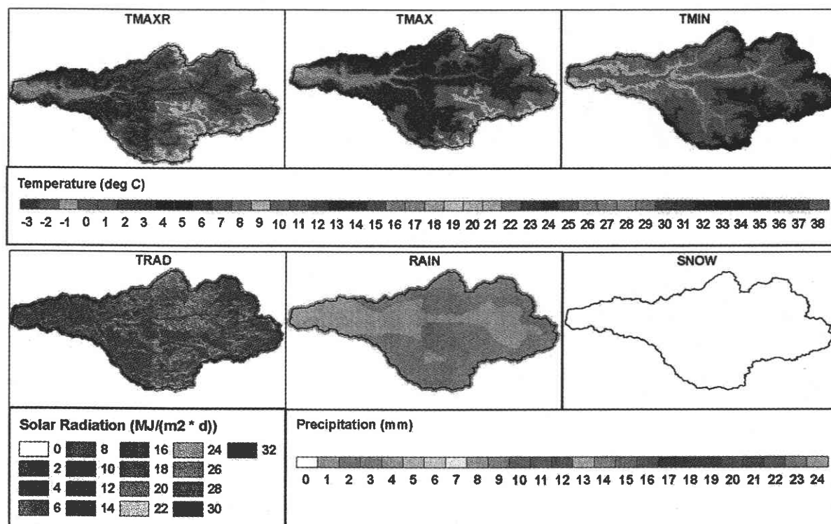
FIG. 11. As in Fig. 10, but for 19 Jun 2003.
