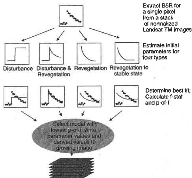
Fig. 2. A conceptual flow of the competing models approach. For each pixel in the image, band 5 reflectance (B5R) is extracted for all 19 years (dates shown in Table 1). Four separate hypothesized models (described in Fig. 3) are then fit to this data, first through an initial estimate of fitting parameters, and then through non-linear iterative curve-fitting. After each of four models is fit to the data, the model with the best fit is selected as describing the pixel, and its descriptive parameter values added to a growing summary image.
