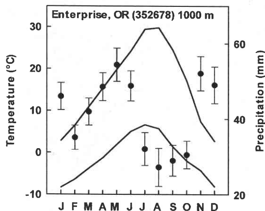
Fig. 1. Climatic features near the Fire and Fire Surrogate fuel reduction study area in northeastern Oregon. Pattern of mean monthly maximum temperature and mean monthly minimum temperature (left axis and solid lines), with the pattern of mean monthly precipitation (right axis, dots with standard error bars) for the period of 1969–2004 at Enterprise, OR.
