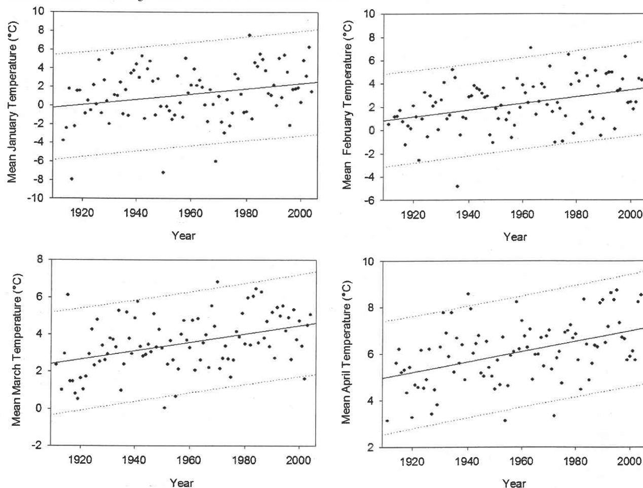
Fig. 2. Winter temperature trends in southeastern Alaska during the 20th century based on simple linear regression models of Ketchikan–Annette combined records. Light dotted lines are 95% confidence intervals.
