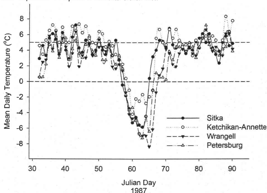
Fig. 4. The 1987 thaw–freeze event based on mean daily temperatures from four weather records. After a prolonged thaw, temperatures dropped approximately 10 °C in 4 days and remained below freezing for 7–10 days, depending on the weather record. Growing (5 °C) and freezing (0 °C) reference temperatures are depicted as horizontal broken lines.
