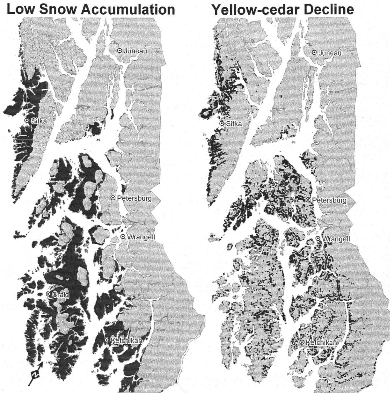
Fig. 8. Comparison of areas of low snow accumulation (left map, solid areas) and the occurrence of cedar decline (right map, solid areas) across southeastern Alaska. Snow map based on PRISM model estimates of snow accumulation categorized into low, moderate, high, and very high zones; only the low zone is shown on map (D. Albert, The Nature Conservancy, Juneau, Alaska, unpublished data). The cedar decline map is based on aerial survey data (Wittwer 2004).
