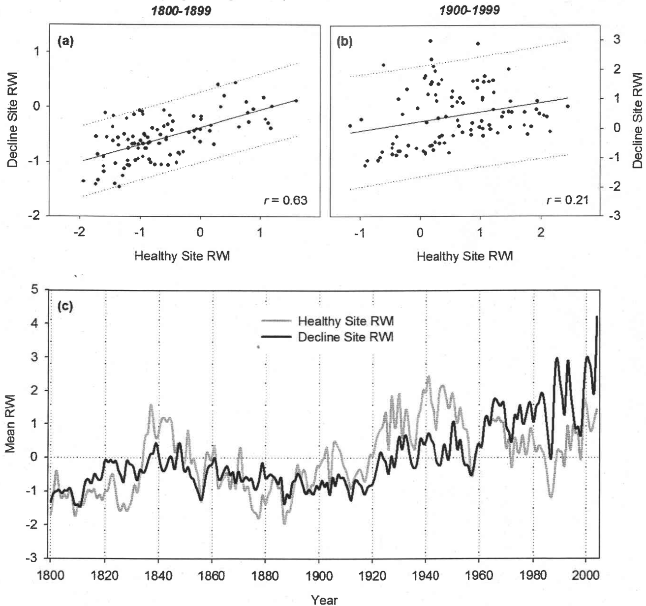
Fig. 6. Statistical and qualitative comparisons of cedar growth chronologies (ring width indices, RWI) between paired sites in the Poison Cove watershed indicating that a common growth signal during the 19th century was decoupled during the 20th century. Analysis is based on a linear model partitioned by century, providing two regressions: (a) 1800–1899 and (b) 1900–1999. Regressions are plotted with 95% confidence intervals. (c) Chronologies plotted in parallel from 1800 to 2004.
