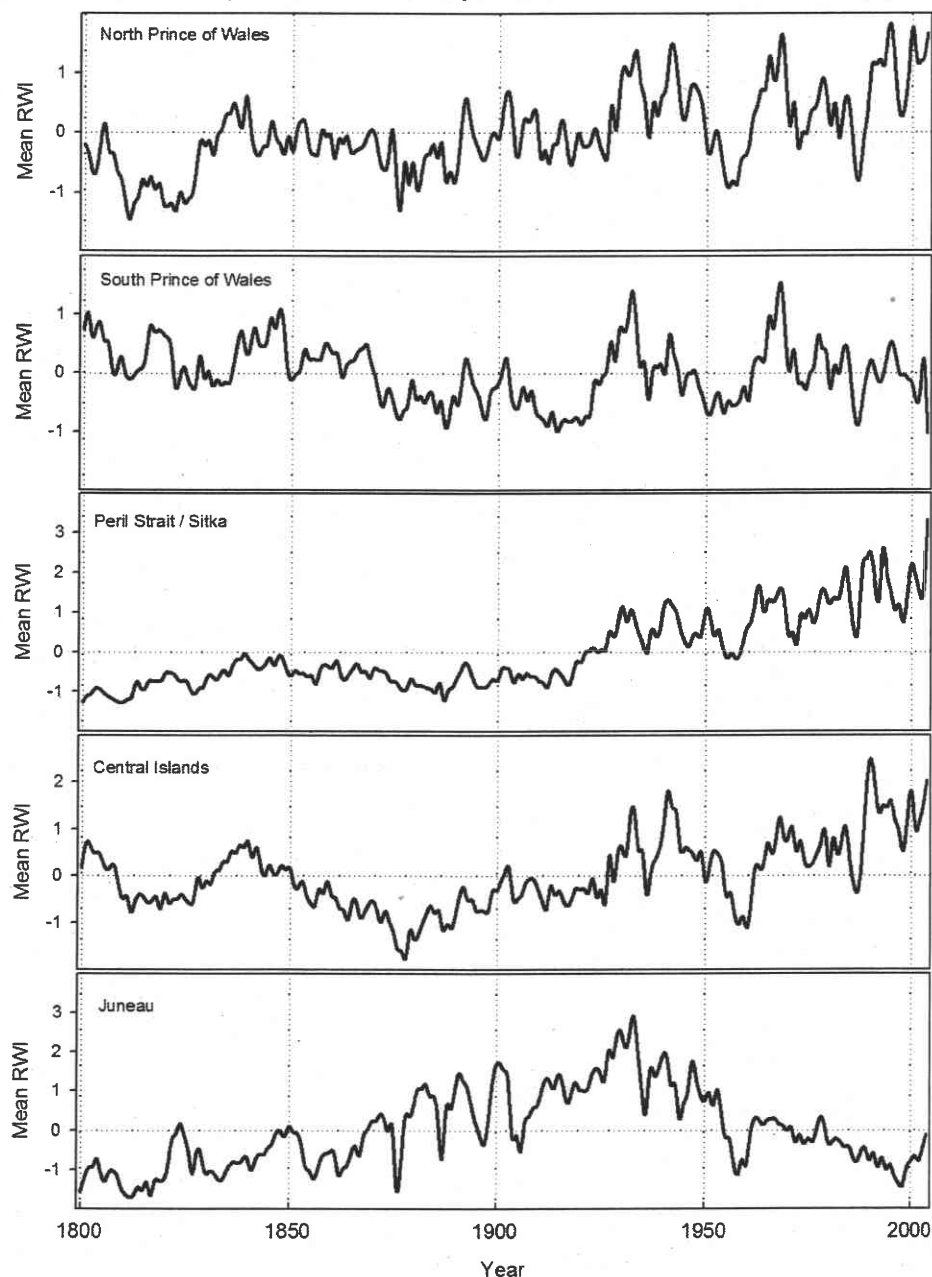
Fig. 5. Comparison of 1800–2004 standardized growth chronologies (ring width indices, RWI) for four region-aggregated declining cedar populations and one healthy cedar population (Juneau). Increasing overall growth in declining populations during the 20th century may be attributable to competitive release caused by decline-related mortality in the stand.
