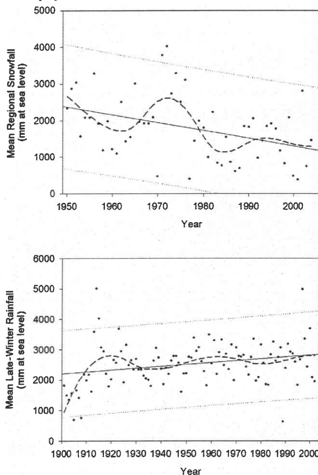
Fig. 3. Regional trends in mean winter snowfall (October–April) and mean late-winter rainfall (January–April) in southeastern Alaska based on existing weather records for the 20th century. Solid lines are linear regression fits with 95% confidence intervals (light dotted lines). Broken lines are cubic spline fits used for illustrative purposes.
