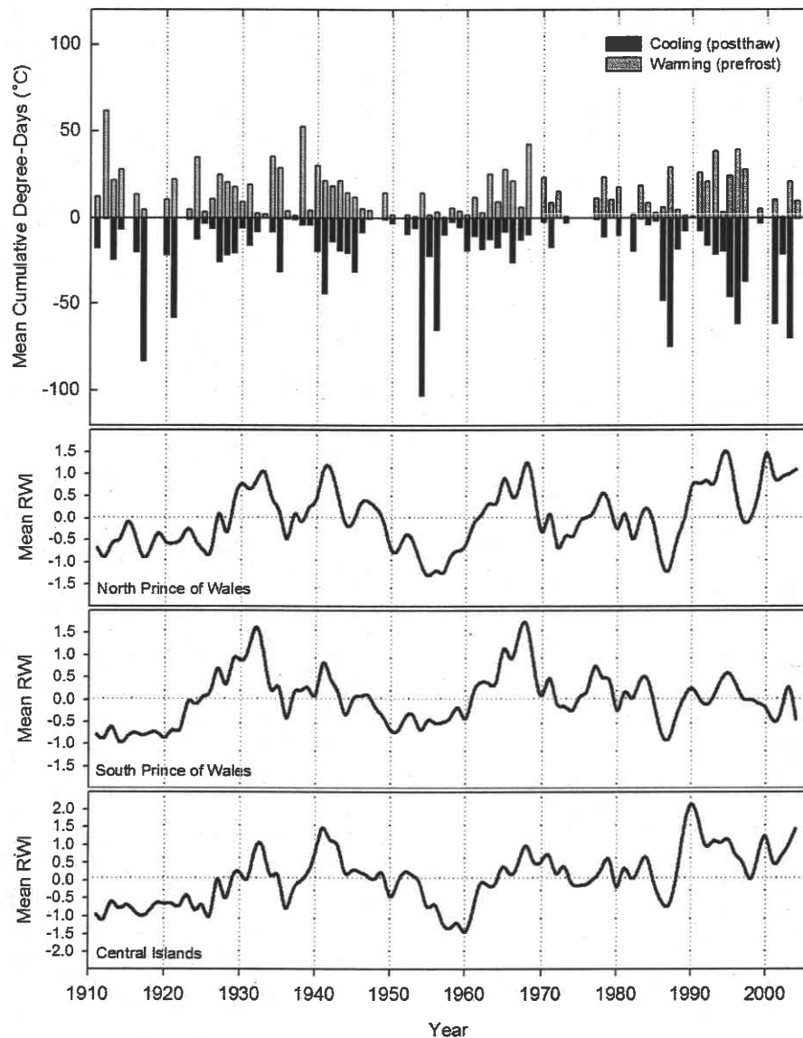
Fig. 7. Comparison of thaw-freeze magnitude and growth chronologies (ring width indices, RWI) for declining yellow-cedar populations in southeastern Alaska. Mean cumulative growing degree-days (GDD) prior to frost are plotted as shaded bars, and mean cumulative cooling degree-days (CDD) after the thaw are plotted as solid bars. CDD are given negative values in this figure for illustrative purposes only. Standardized cedar chronologies are plotted in parallel with thaw-freeze records from 1910 to 2004.
