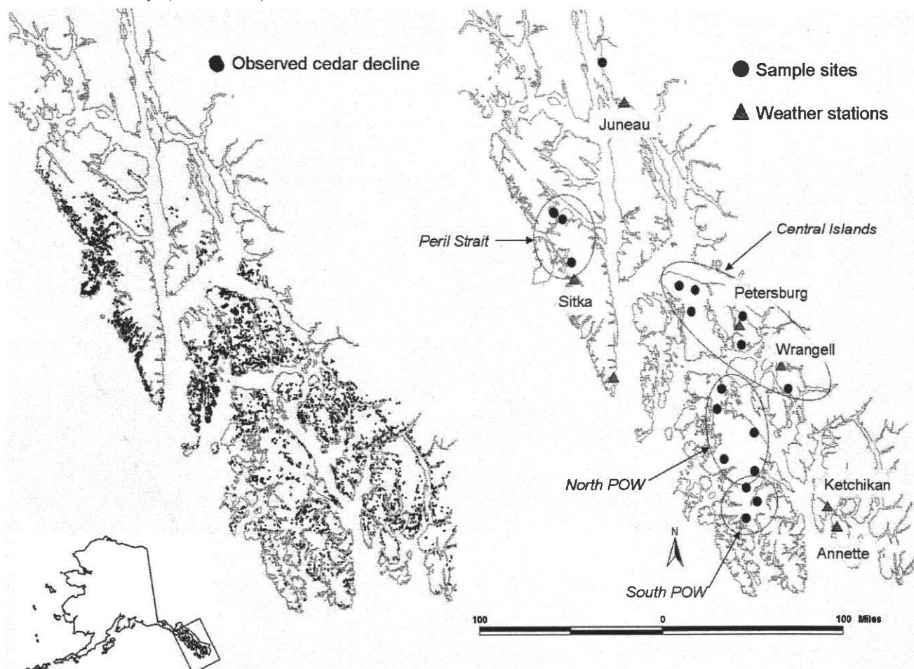
Fig. 1. Maps of observed cedar decline, sample sites, weather stations, and sampling provinces in southeastern Alaska. Cedar decline map based on aerial surveys (Wittwer 2004). All weather stations meet First Order standards and are located near sea level.
