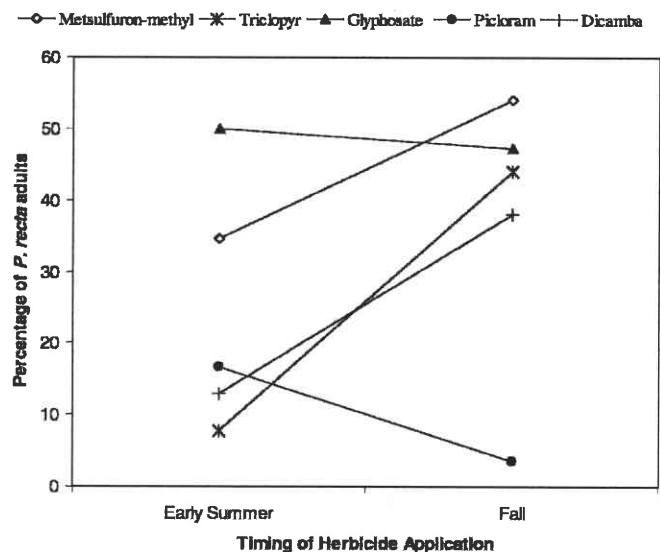
Figure 3. Interactions between timing of herbicide application and herbicide type on the proportion of living sulfur cinquefoil individuals that were adults (reproductively active) in 2005. Herbicides were applied in 2002 in May (early summer) and October (fall).
