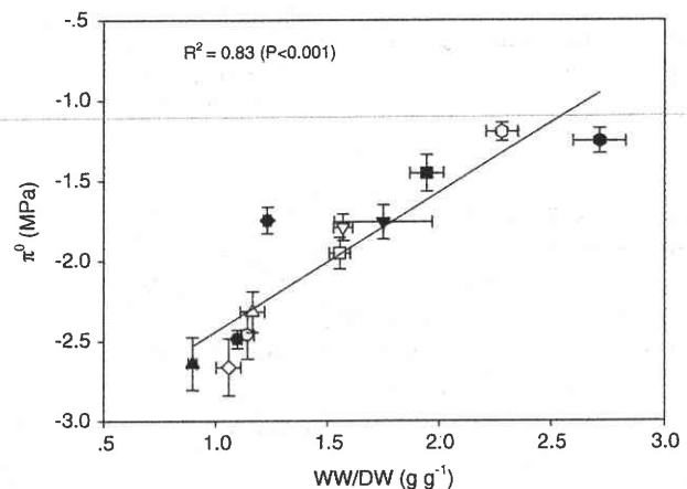
Fig. 3 Relationship between turgor loss point ( \pi^0 ) and leaf water content per unit leaf dry mass at full turgor ( WM/DW ). Open hexagon Savanna species of Aegiphila , filled hexagons forest species of Aegiphila ; other symbols are the same as in Fig. 1. Error bars show \pm 1 SE ( n = 5–6 )
