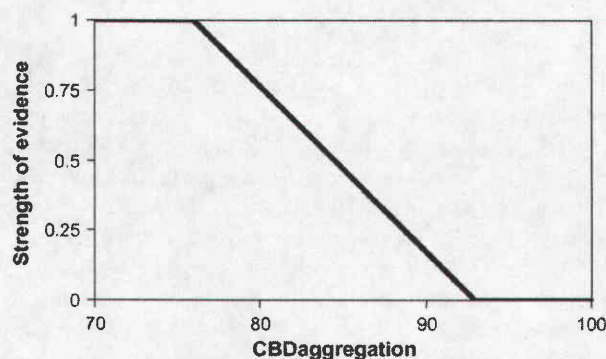
Fig. 4. The fuzzy membership function used to evaluate strength of evidence for the proposition of low canopy bulk density. The proposition is fully satisfied when the observed value of CBDaggregation \leq 76 , and there is no evidence for the proposition if CBDaggregation \geq 93 (Table 2). Observed values of CBDaggregation that fall within the open interval (76, 93) evaluate to partial support for the proposition, based on linear interpolation between 76 and 93.
