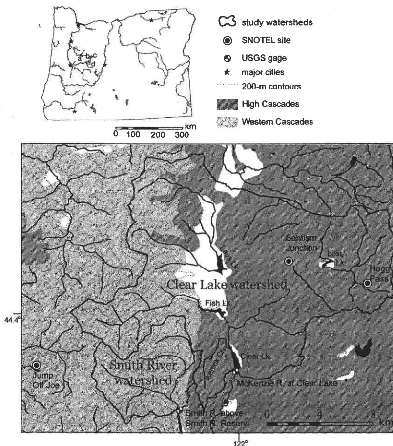
Figure 1. Map showing the study watersheds relative to their location in Oregon and to Cascades topography and geology. On the Oregon map, the letter 'a' next to a gauge symbol indicates the position of the stream gauge for South Santiam River below Cascadia, 'b' indicates Smith River above Smith River Reservoir, 'c' indicates McKenzie River at Clear Lake, and 'd' indicates McKenzie River at McKenzie Bridge
