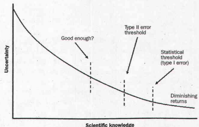
Figure 8. The relationship between the level of scientific knowledge of a system and the uncertainty about the results of applying conservation or management actions to that system.
