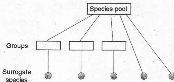
Figure 1. The hierarchical relation between the species pool of interest, species groups, and surrogate species. Surrogate species may be used either to represent the species pool as a whole or to represent the subsets of that pool designated by species groups, or the groups themselves may be used as distillations of the larger species pool.
