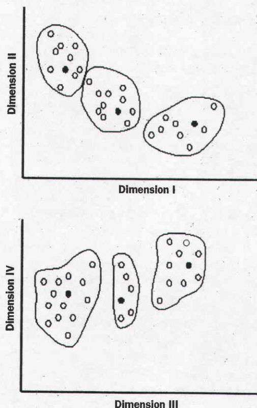
Figure 2. Hypothetical example of how a single set of species (circles) might be arrayed in a multidimensional space (e.g., principal component analysis) when different criteria (variables) are used to characterize the species. Solid circles indicate potential surrogate species for each group of species.
