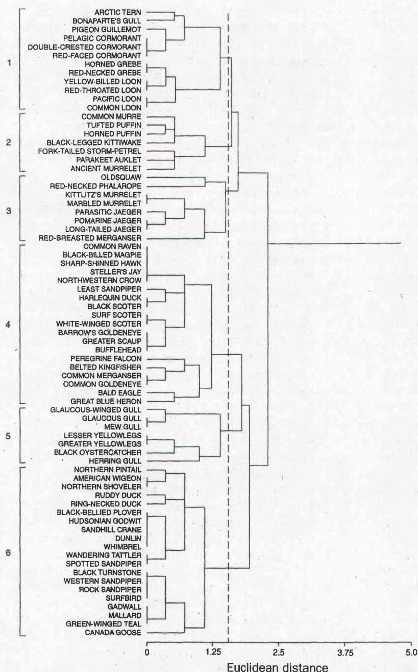
Figure 7. A hierarchical cluster diagram of 73 seabird species occurring in Prince William Sound, Alaska, grouped by similarities in seasonal residency, breeding aggregation, nest-site location, prey type, foraging method, and feeding zone. The vertical line represents a similarity threshold for determining species clusters, within which a representative species could be selected as a surrogate. Using different levels of Euclidean distance similarity would yield different clusters, and correspondingly different surrogates. Reprinted with permission from Wiens and colleagues (1996).
