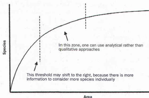
Figure 5. With growing knowledge about the species and system of interest, the surrogate zone may shift to the right on the species-area function curve because more species can be considered individually. More information also enables one to use quantitative rather than qualitative approaches to identify surrogate species or groups within the surrogate zone.
