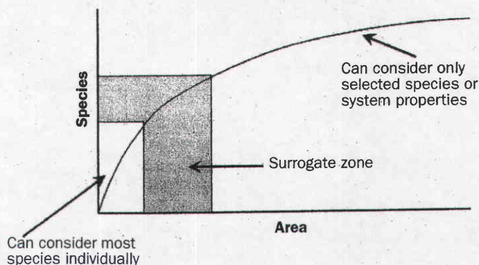
Figure 3. The species-area relationship. When the number of species or the size of the area is small, individual species can be considered and surrogate approaches may be unnecessary. When the size of the area or number of species is very large, surrogate species or groups may not adequately represent the variety of taxa or habitats present and such approaches are not useful. In between is the “surrogate zone,” where surrogate species or groups can be used effectively to reduce the dimensionality of the system.
