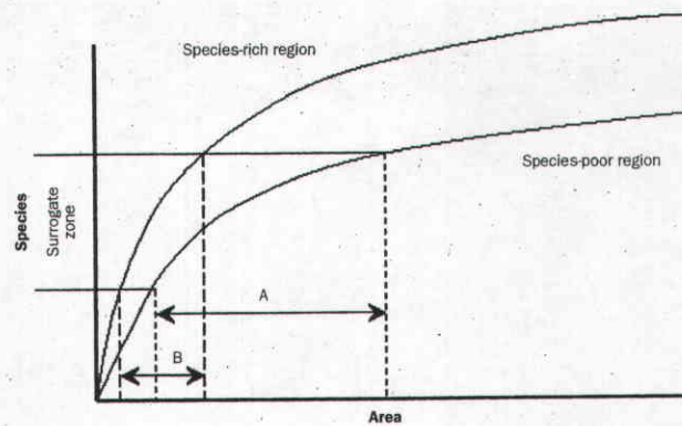
Figure 4. In a species-poor region the surrogate zone is shifted toward larger areas (A) compared with a species-rich region (B) because the utility of surrogate species or groups is determined more by the number of species to be considered than by area per se.
