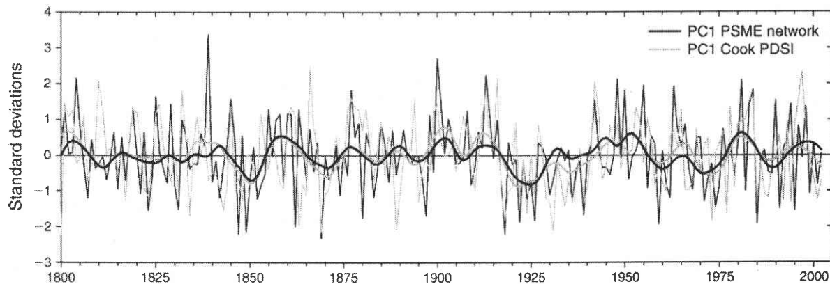
FIG. 7. Douglas-fir ("PSME") network PC1 time series and PC1 of regional reconstructed ("Cook") PDSI. PCA comparison of the 1800–2002 common signal from this study and the common signal from six PDSI (Palmer drought severity index) grid point reconstructions over the same region is shown. Bold lines indicate 21-yr lowess-smoothed time series (PSME, black; PDSI, gray).
