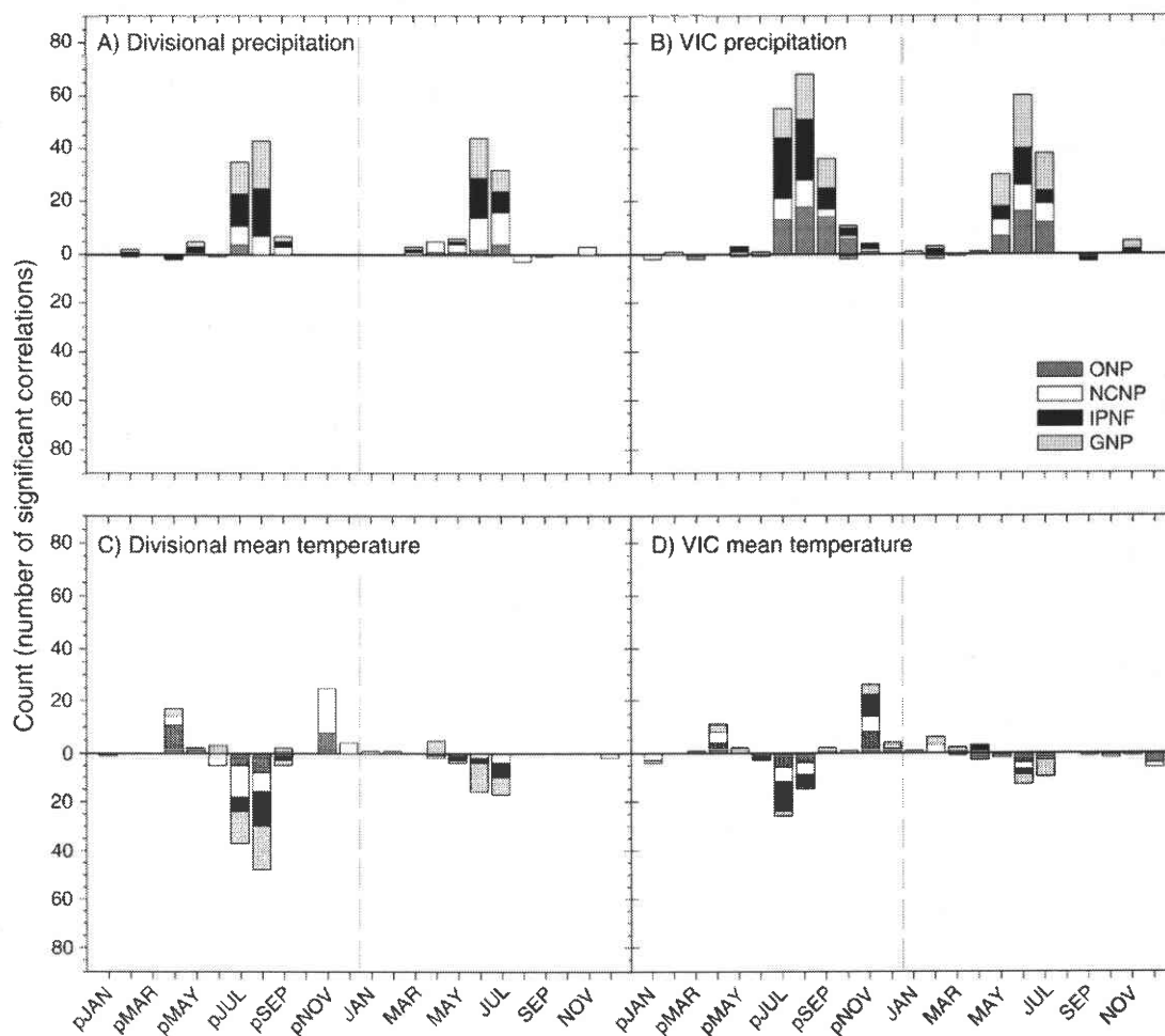
FIG. 3. Monthly divisional (left-hand panels) and variable infiltration capacity (VIC; right-hand panels) hydrological models for (A, B) precipitation and (C, D) mean temperature relationships with growth. Bars indicate the number of significant ( P < 0.01 ) correlations between lag-1 (e.g., pJAN) or year-of-growth (e.g., JAN) precipitation and tree-ring time series from all watersheds. In this and all subsequent correlation plots, positive counts are above the line, and negative counts are below. Counts have been weighted such that the different numbers of sample chronologies in Olympic National Park (ONP), North Cascades National Park (NCNP), Idaho Panhandle National Forest (IPNF), and Glacier National Park (GNP) have the potential to contribute equally to the total count and area in each bar. The maximum number of significant correlations is therefore 144, not 124, so that the area in the bars is directly comparable.
