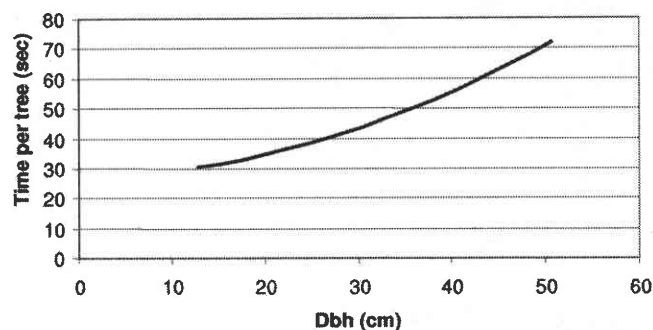
Figure 7. Stroke-boom delimber productivity processing ponderosa pine (1.4 pieces from each stem).
