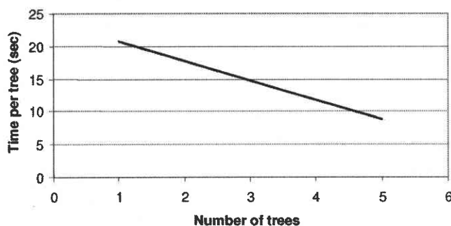
Figure 5. Feller-buncher productivity in a fuel reduction thinning.
