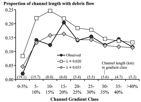
Fig. 10. Predicted and observed proportions of total channel length within the Mapleton study site, divided by gradient class, traversed by debris flows. Predictions were made with two values of \lambda (rate parameter for the exponential distribution of debris-flow travel lengths, Eq. (18)), for which a \lambda value of 0.035 best matches the observations.
