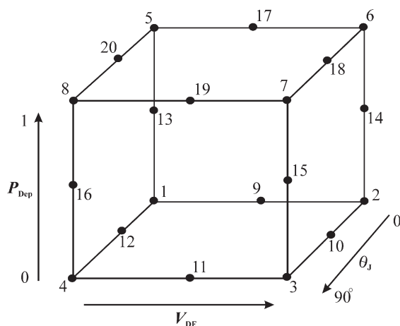
Fig. 1. A 20-node, 3-dimensional serendipity brick for estimating p_J , the probability that a debris flow continues through a tributary junction. Values of depositional probability P_{\text{Dep}} in the receiving channel, tributary junction-angle \theta_J , and debris-flow-volume index V_{\text{DF}} determine position within the brick. Values of p_J are determined at all points within the brick by the values set at the 20 nodes indicated on the surface.
