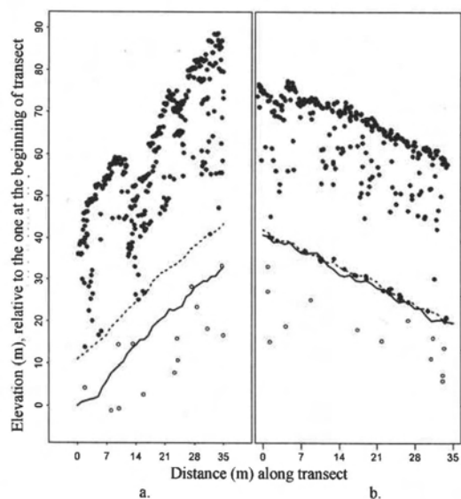
Figure 5. Plot profiles of 1 m depth depicting laser returns either maintained (dots) or filtered out (hollow circles) during data preprocessing, and surveyed (solid lines) and LiDAR-derived (dashed lines) ground surfaces.
