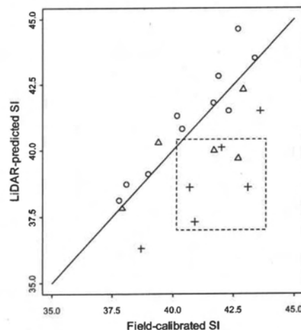
Figure 6. Plot Site Index values computed using the tallest trees surveyed in the field and their LiDAR-derived equivalent. Symbols indicate plot membership in classes of fidelity for the ground surface extracted from the laser data.
