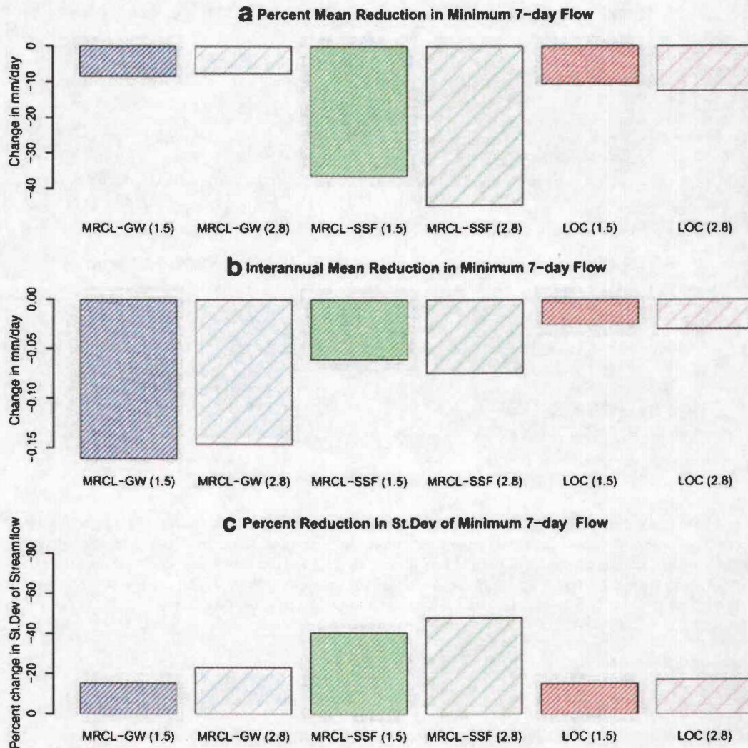
Fig. 10 RHESys modeled change in mean minimum 7-day streamflow for 1.5°C (warm 1) and 2.8°C (warm 2) temperature increase scenarios. Comparisons are made between LOC, MRCL modeled with deeper groundwater included, and hypothetical scenario of MRCL modeled with only shallow subsurface flow system. Results shown as a percent reduction in flow, b actual reduction in flow (normalized by drainage area), and c as percent reduction in year-to-year standard deviation
