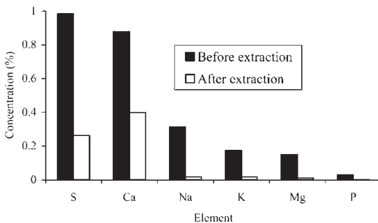
Figure 4. Mineral content determined by inductively coupled plasma (ICP) analysis of wood flour from saltcedar before and after a 4-h Soxhlet extraction with water.
