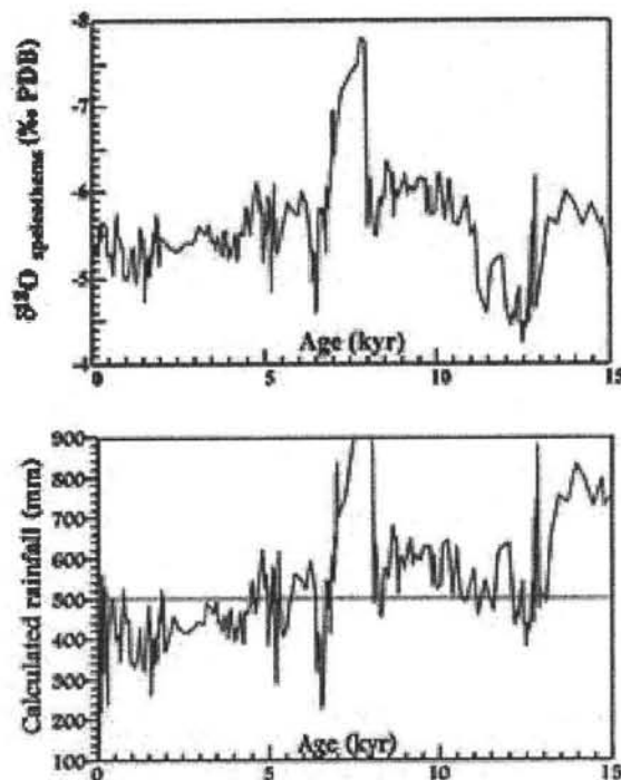
Figure 5. Paleo-climatic records according to the isotopic values in cave deposits in Israel (after Bar-Matthews et al. , 2003). The lower graph of the calculated rainfall is based on the isotopic record of \delta^{18}\text{O} .
