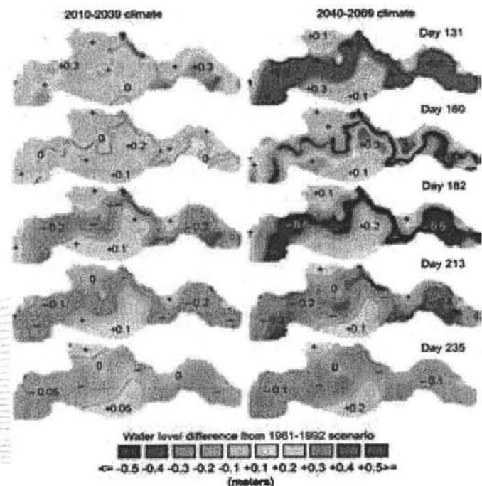
Figure 12. Water level differences (measured as head in layer 2 of the unconfined aquifer) between a) future (2010-2039) and present climate, and b) future (2040-2069) and present climate under pumping conditions. Maps by time step in days 131 to 235. Positive contours are shown at 0.1 m interval. The zero contour is a dashed line. Negative contours are not shown. Darkest blue colors indicate values < -0.5 m (along rivers only). At day 101 (not shown), difference map has values within 0.1 m of zero (from Scibek et al., 2007)
