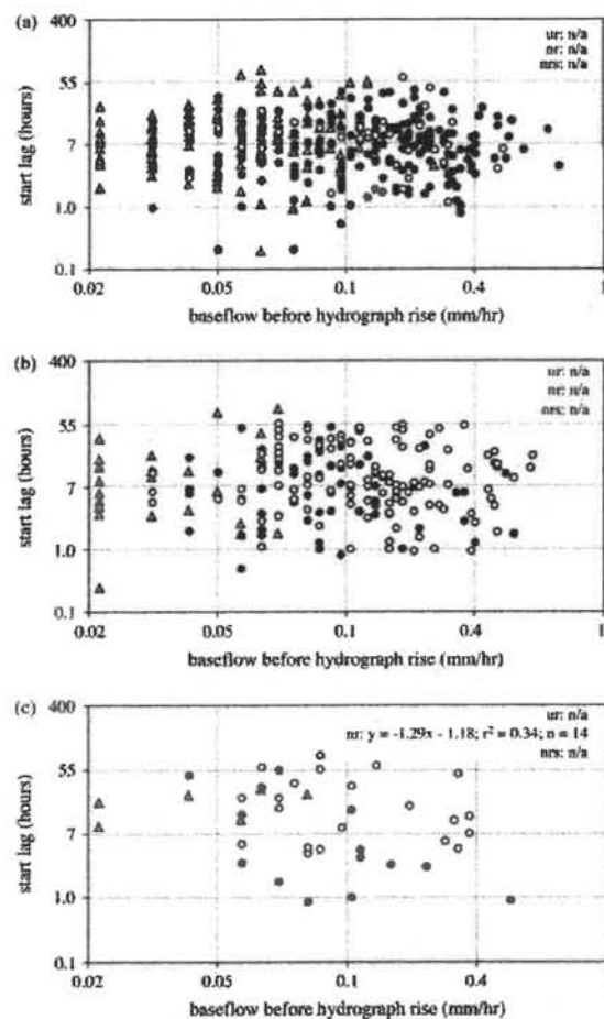
Figure 9. Relationships between baseflow before hydrograph rise ( \text{mm h}^{-1} ) and start lag (h) for three event types in three watersheds: rain events on unsaturated soil ('ur', gray triangles), rain events on near-saturated soils ('nr', solid circles), and rain-on-snow events on near-saturated soil ('nrs', open circles), from (a) Watershed 9, 1969-1992; (b) Watershed 2, 1964-1992; and (c) Watershed 8, 1985-1992. Data were log-transformed for analysis and plotting
