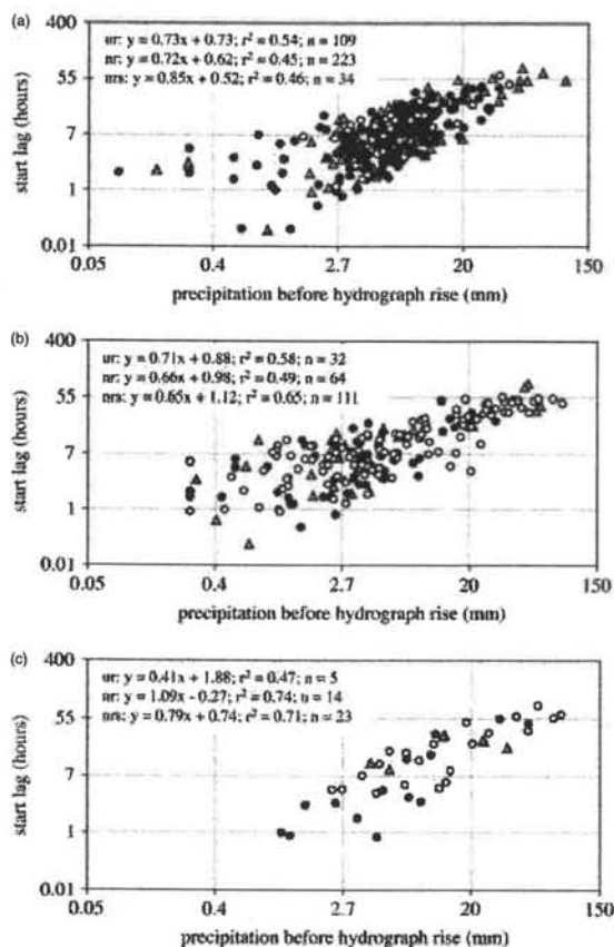
Figure 8. Relationships between precipitation before hydrograph rise (mm) and start lag (h) for three event types in three watersheds: rain events on unsaturated soil ('ur', gray triangles), rain events on near-saturated soils ('nr', solid circles), and rain-on-snow events on near-saturated soil ('nrs', open circles), from (a) Watershed 9, 1969-1992; (b) Watershed 2, 1964-1992; and (c) Watershed 8, 1985-1992. Data were log-transformed for analysis and plotting
