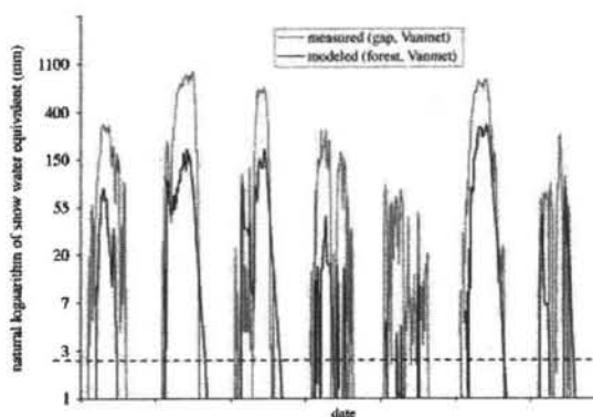
Figure 4. Measured and modelled snow water equivalents. Snow water equivalent was measured at a canopy gap containing the VanMet station (1100 m elevation; see Figure 1) and modelled for the HRU containing VanMet, but assuming that the area was forested. Patterns of measured and modelled snow demonstrate the order-of-magnitude differences in snow between canopy gaps (grey line, measured) and under forest (black line, modelled) and the ephemeral nature of snowpacks even at high elevation in some years. A snow water equivalent of 2.5 mm was used to define 'on snow' conditions (horizontal dashed line)
