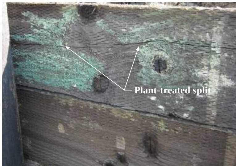
Figure 4-58. New ACZA treated back wall planks properly seasoned prior to treatment
