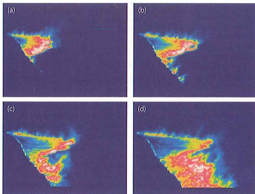
FIG. 4. Infrared image sequence covering the ignition of the experimental burn. Peak temperatures measured were (a) 796°, (b) 774°, (c) 760°, and (d) 834°C.
