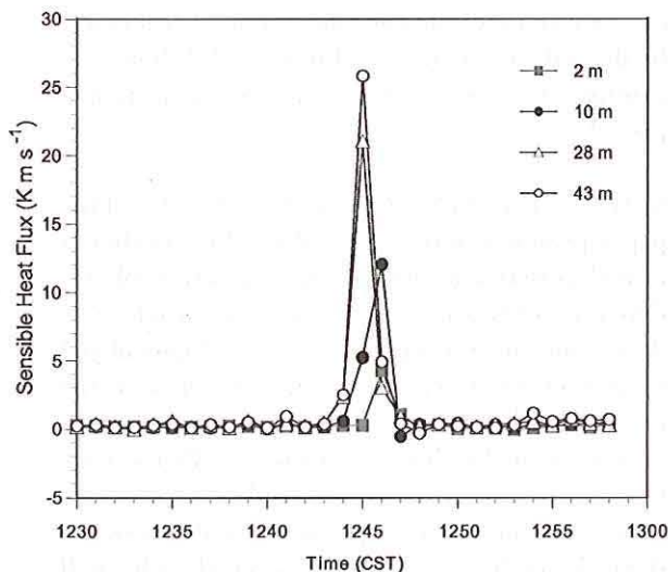
FIG. 9. Sensible heat fluxes calculated for each level of the main tower.
