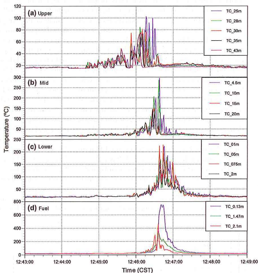
FIG. 6. Thermocouple measurements of temperature at different levels on the main tower, (a) the upper levels, (b) the midlevels, (c) the low levels, and (d) the fuel temperatures measured away from the tower.
