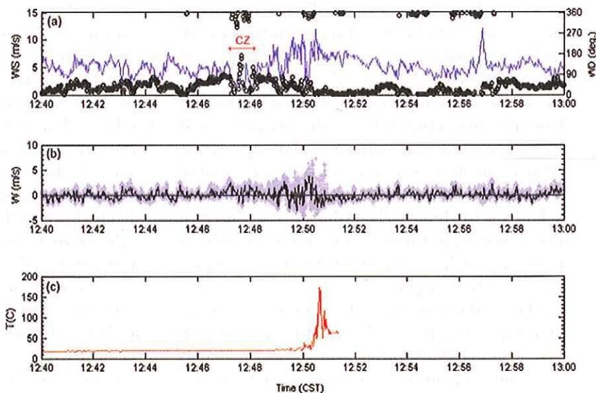
FIG. 10. Time series of 1-s average data from the 2-m sonic anemometer on the south tower. (a) Wind speed is indicated by the blue line and wind direction by black circles. (b) The vertical velocity, w , where blue crosses are the instantaneous 20-Hz tilt-corrected values and the solid black line is 1-s data. (c) Fine-wire thermocouple temperature ( T ). (a) The convergence zone is indicated by CZ.
