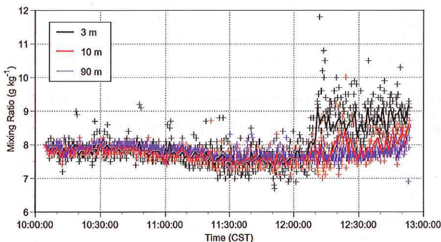
FIG. 8. Water vapor mixing ratio obtained from tethered system downwind of the burn unit during black lining operations. Solid lines are 1-min-averaged values and crosses are 10-s instantaneous values.
