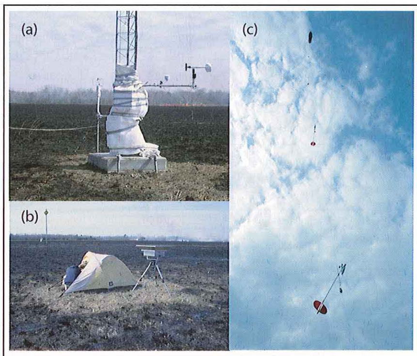
FIG. 2. Photographs of main tower base (a) after burn showing protection around sonic anemometer and tower, (b) mini sodar (Remtech, Inc., PAO) after burn, and (c) tethered sonde system deployed in tower mode with five sondes.
