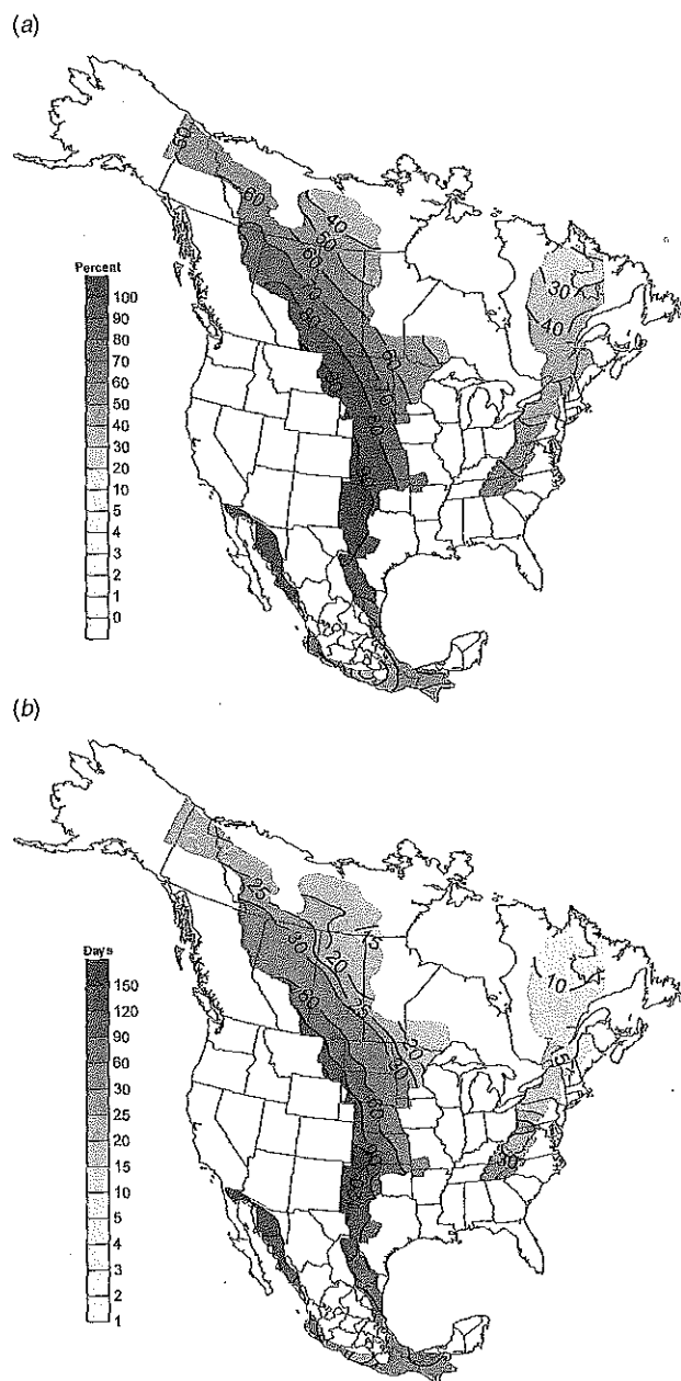
Fig. 9. Haines Index mid variant: (a) frequency (as percentage of days p summer season) that the index is \geq 4 , and (b) the maximum consecutive number of days in summer during 1961–2000 with index values \geq 4 at 0000 UTC. Locations outside the mid variant region are shown in white.
