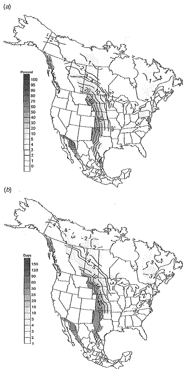
Fig. 11. As in Fig. 8 except for values of the Haines Index mid variant equal to 6.
