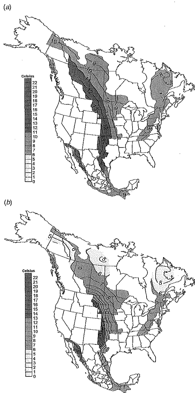
Fig. 7. Summer (June, July, August) (a) mean environmental lapse rate (850-hPa temperature minus 700-hPa temperature) in ^{\circ}\text{C} , (b) 850-hPa dewpoint depression ( ^{\circ}\text{C} ) during 1961–2000 for the mid variant of the Haines Index. Shading refers to the categorical values for the stability (A) and humidity (B) components, with light shading, medium shading, and dark shading representing categorical values of 1, 2, and 3, respectively. Locations outside the mid variant region are in white.
