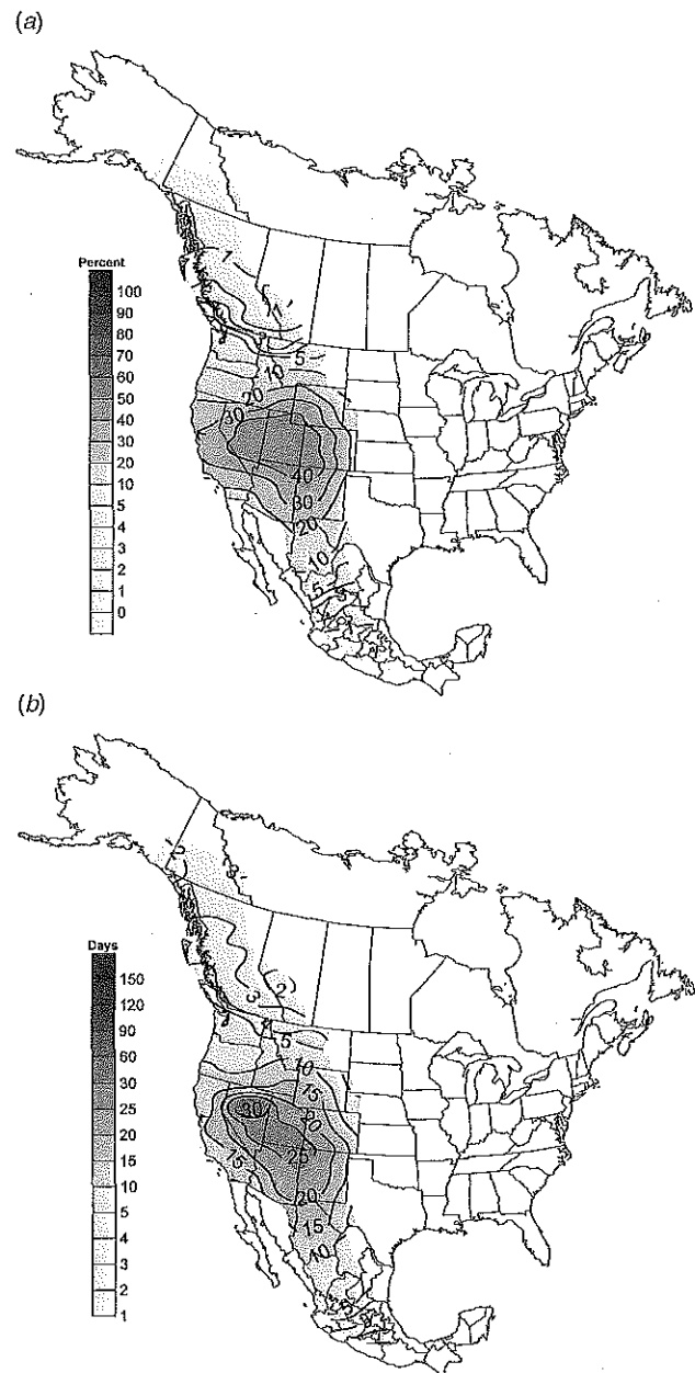
Fig. 15. As for Fig. 13 except for values of the Haines Index high variant \geq 5 .
