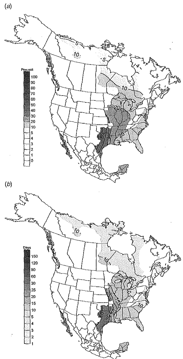
Fig. 5. As in Fig. 3 except for values of the Haines Index low variant \geq 5 .
