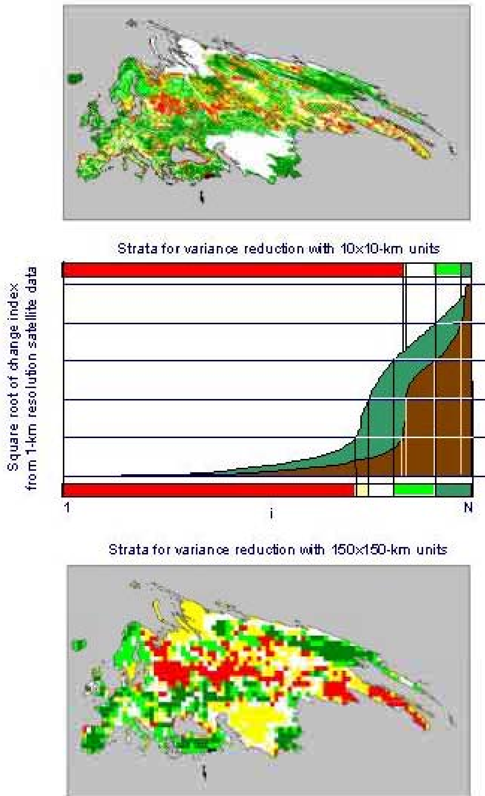
Figure 5: Stratification based on Neyman allocation for 150x150-km and 10x10-km Sample Units
