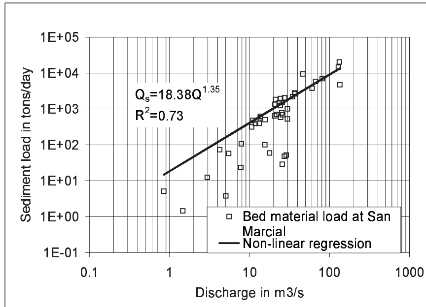
Figure A.2: Bed material data measured at the San Marcial gage from 1990 to 1997. The rating curve fitted to the data is indicated.
