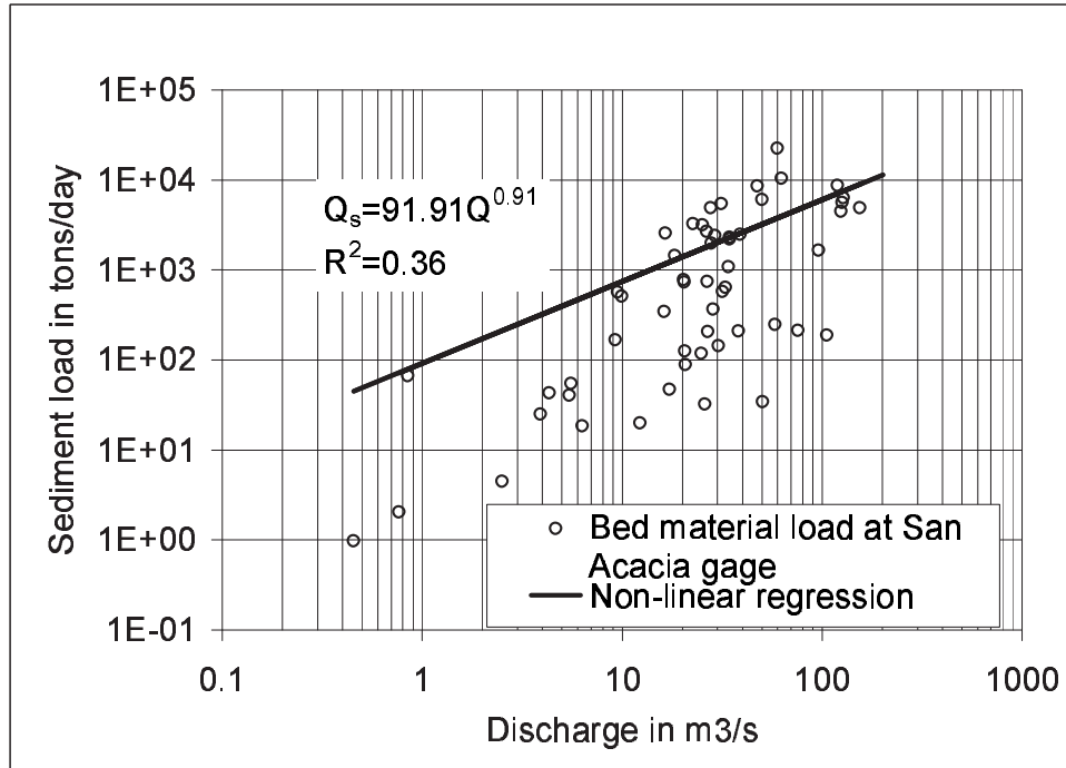
Figure A.1: Bed material data measured at the San Acacia gage from 1990 to 1997. The rating curve fitted to the data is indicated.
