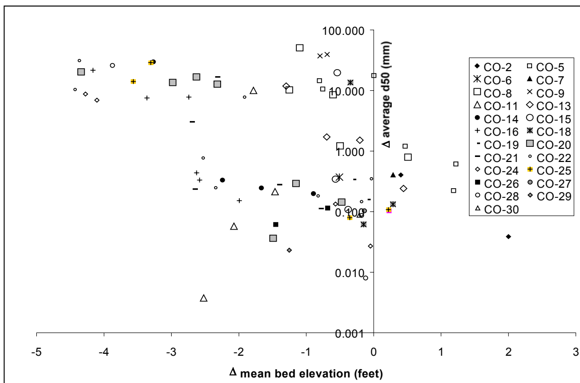
Fig. 3.19. Change in mean bed elevation versus change in median bed material size with respect to the 1971 data.
