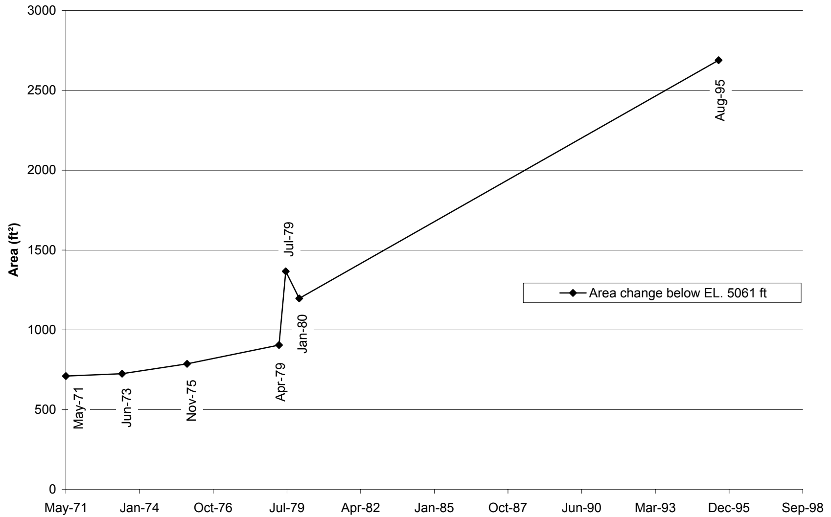
Fig. E-55. Change in cross section area with time at cross section CO-28.
