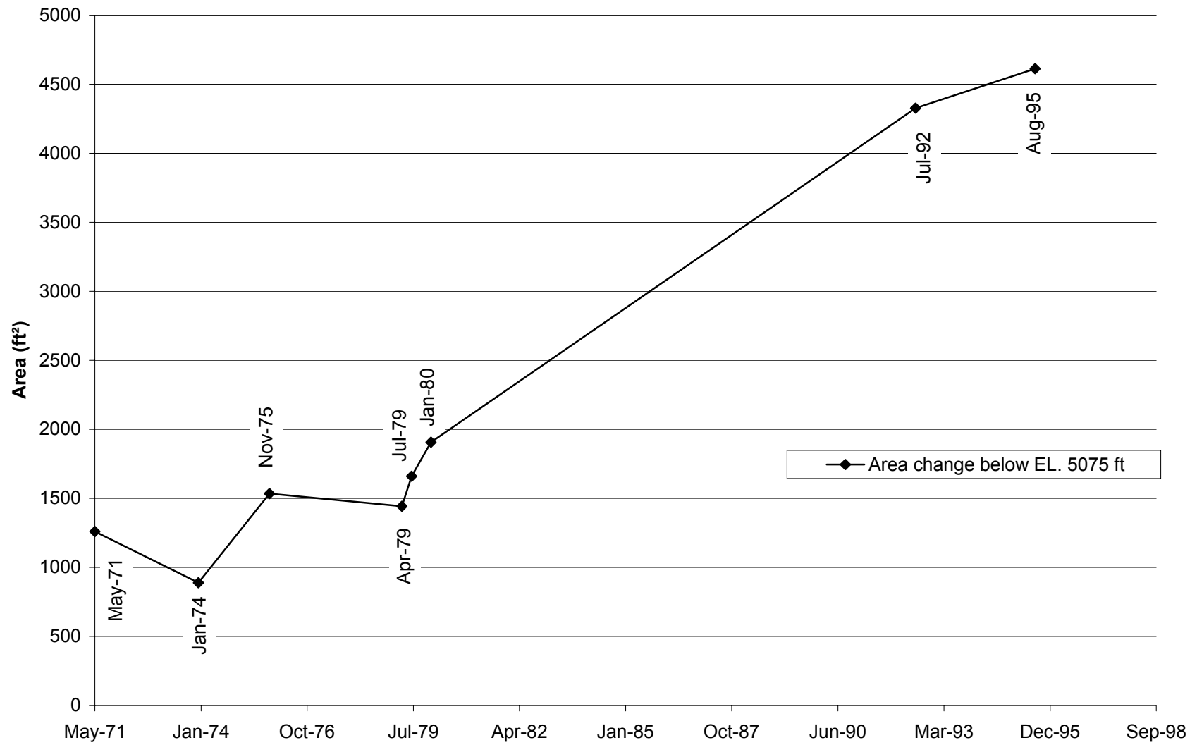
Fig. E-52. Change in cross section area with time at cross section CO-25.
