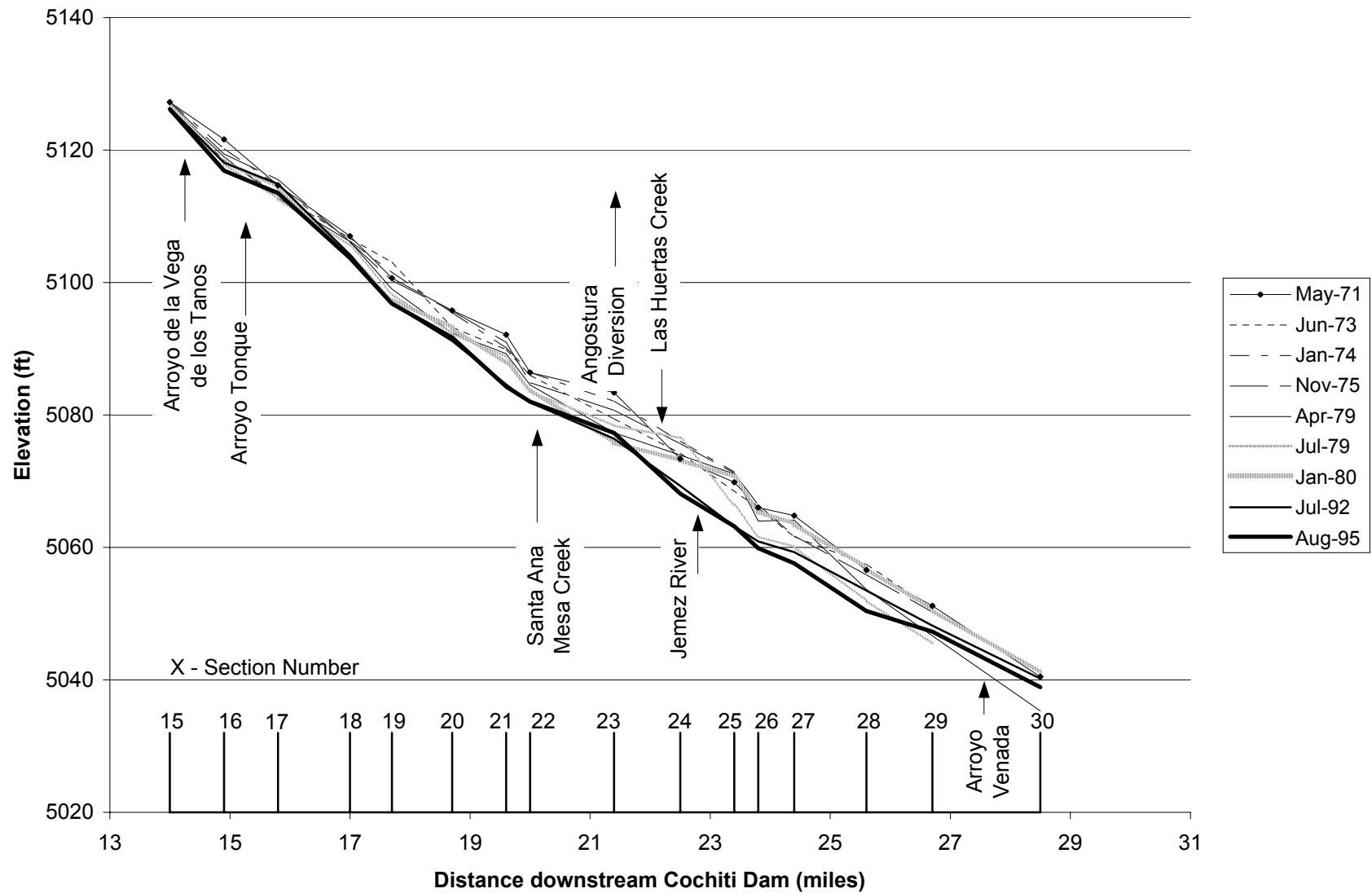
Fig. 3.8. Thalweg profile from cross section CO-15 to cross section CO-17
