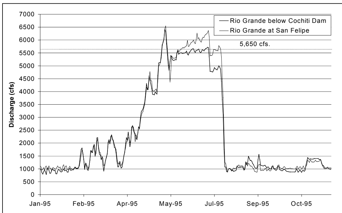
Fig. 3.6. 1995 flow hydrograph of Rio Grande below Cochiti Dam and Rio Grande at San Felipe gaging stations.
