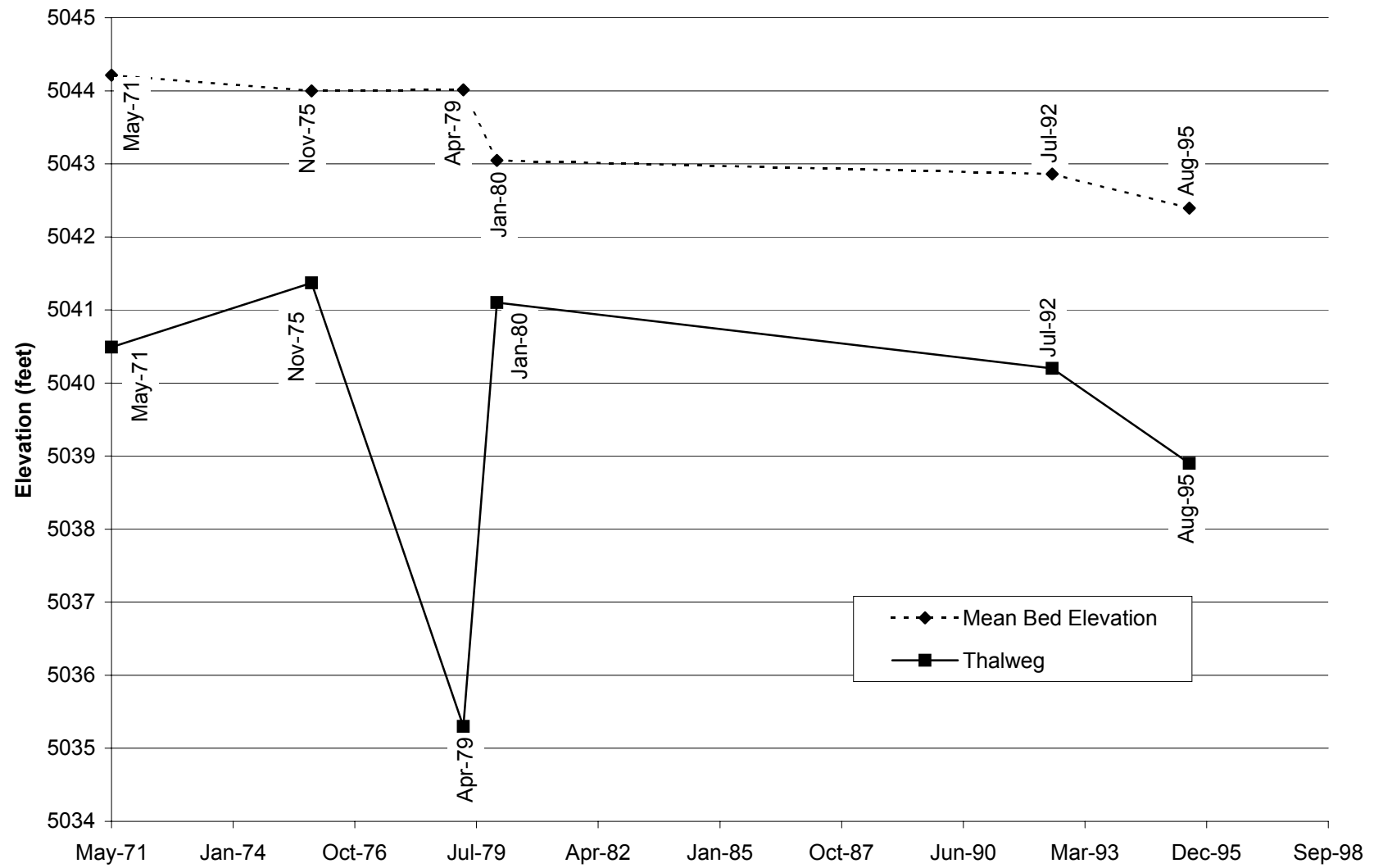
Fig. E-28. Change in thalweg elevation and mean bed elevation with time at cross section CO-30.
