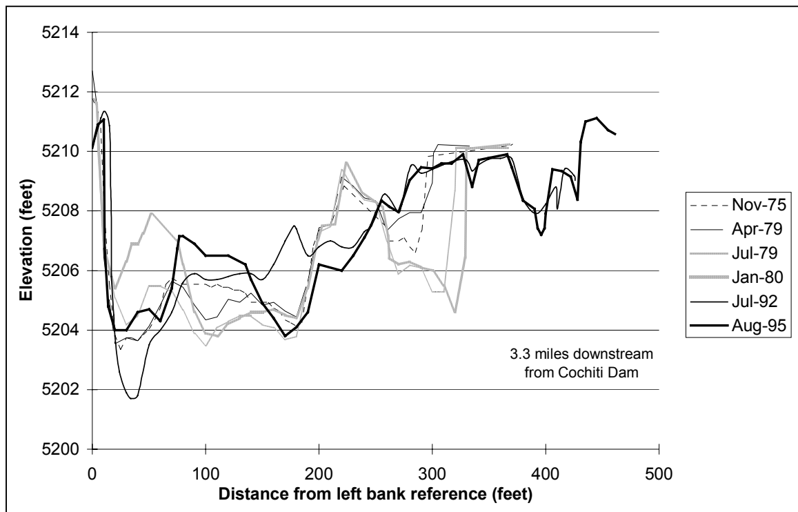
Figure 4.2. Cross section CO-3.
