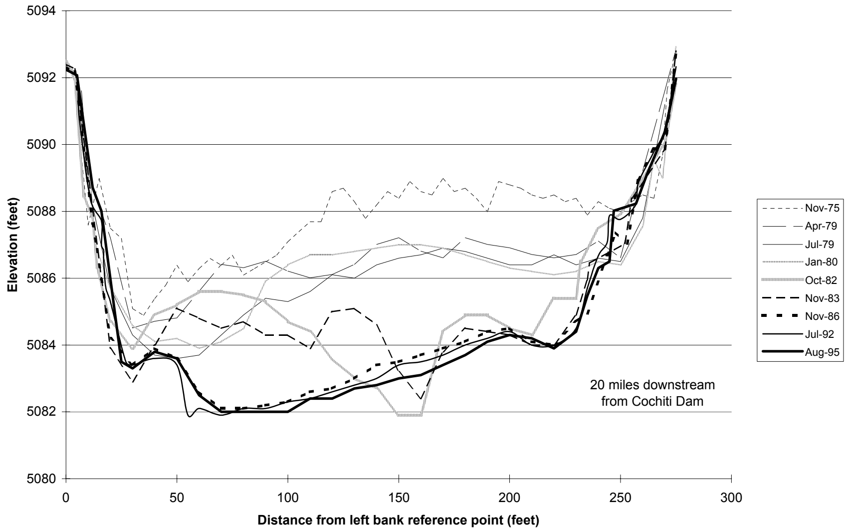
Fig.D-13. Cross Section CO-22.
