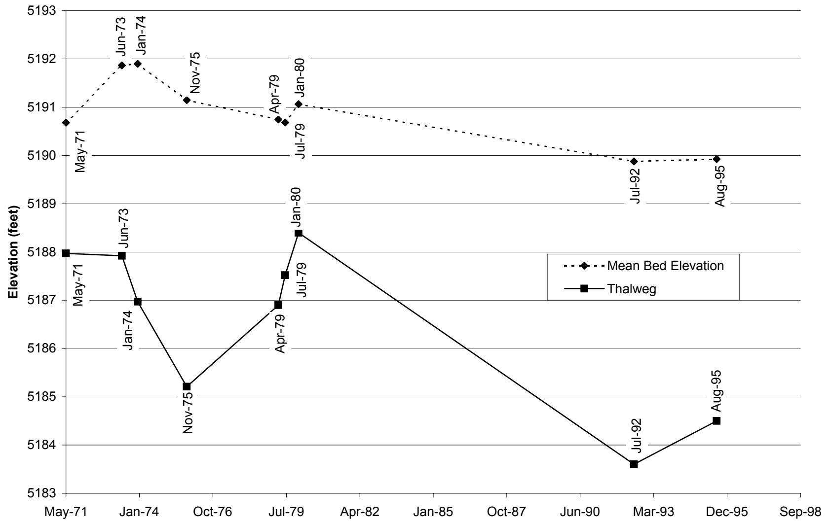
Fig. E-4. Change in thalweg elevation and mean bed elevation with time at cross section CO-5.
