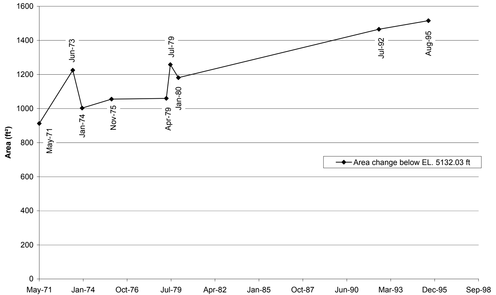
Fig. E-42. Change in cross section area with time at cross section CO-15.
