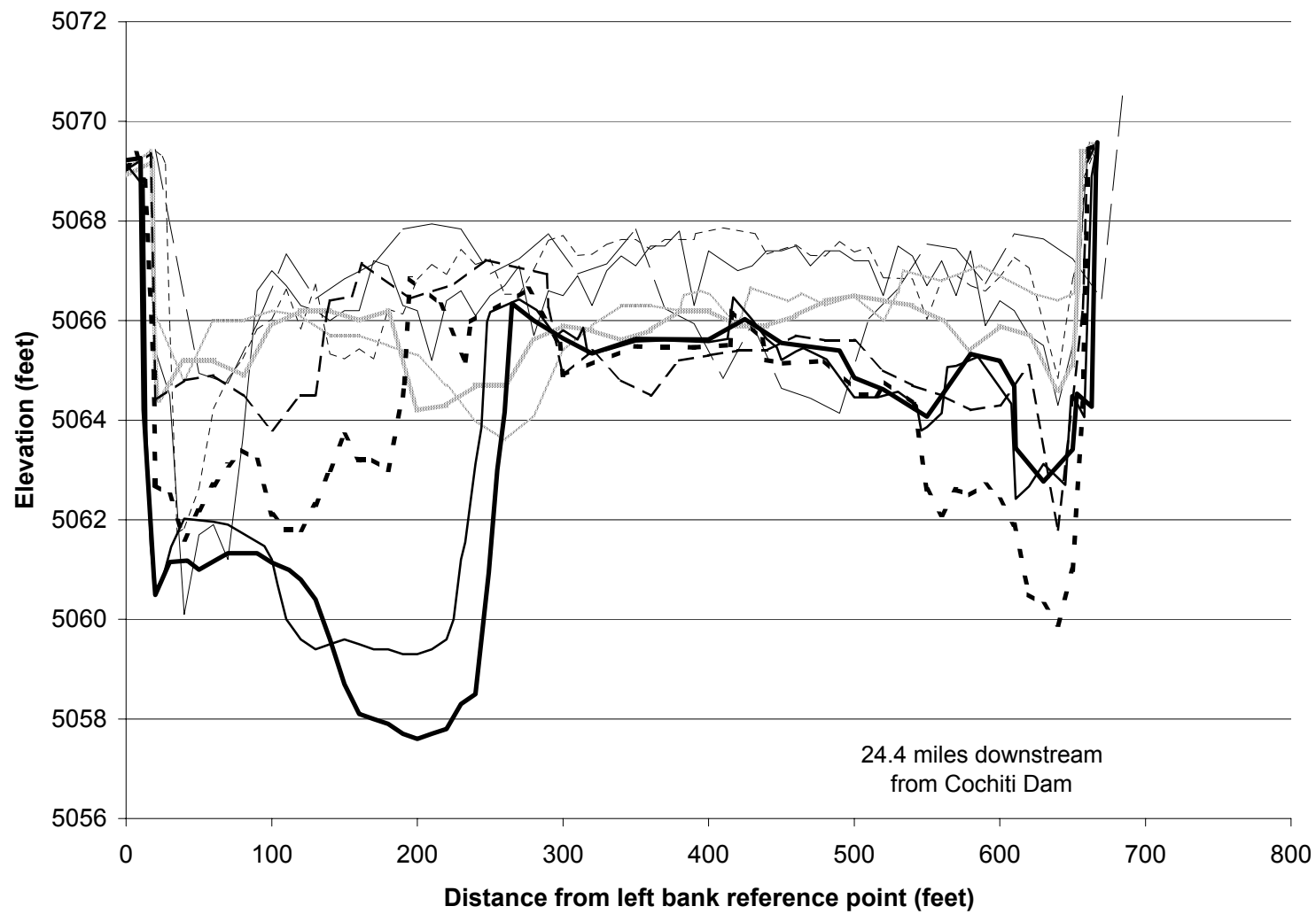
Fig.D-17. Cross Section CO-27.
