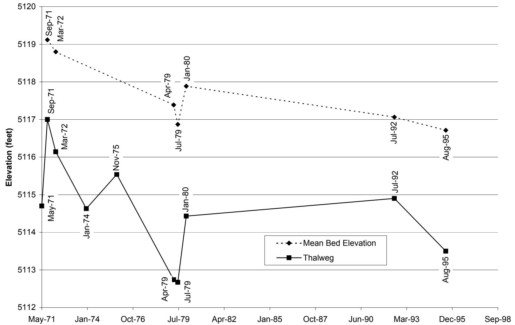
Fig. E-15. Change in thalweg elevation and mean bed elevation with time at cross section CO-17.
