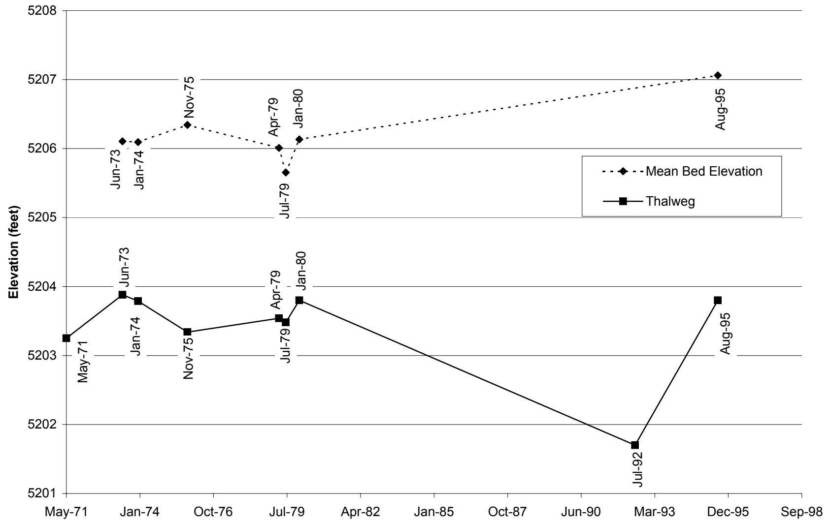
Fig. E-2. Change in thalweg elevation and mean bed elevation with time at cross section CO-3.
