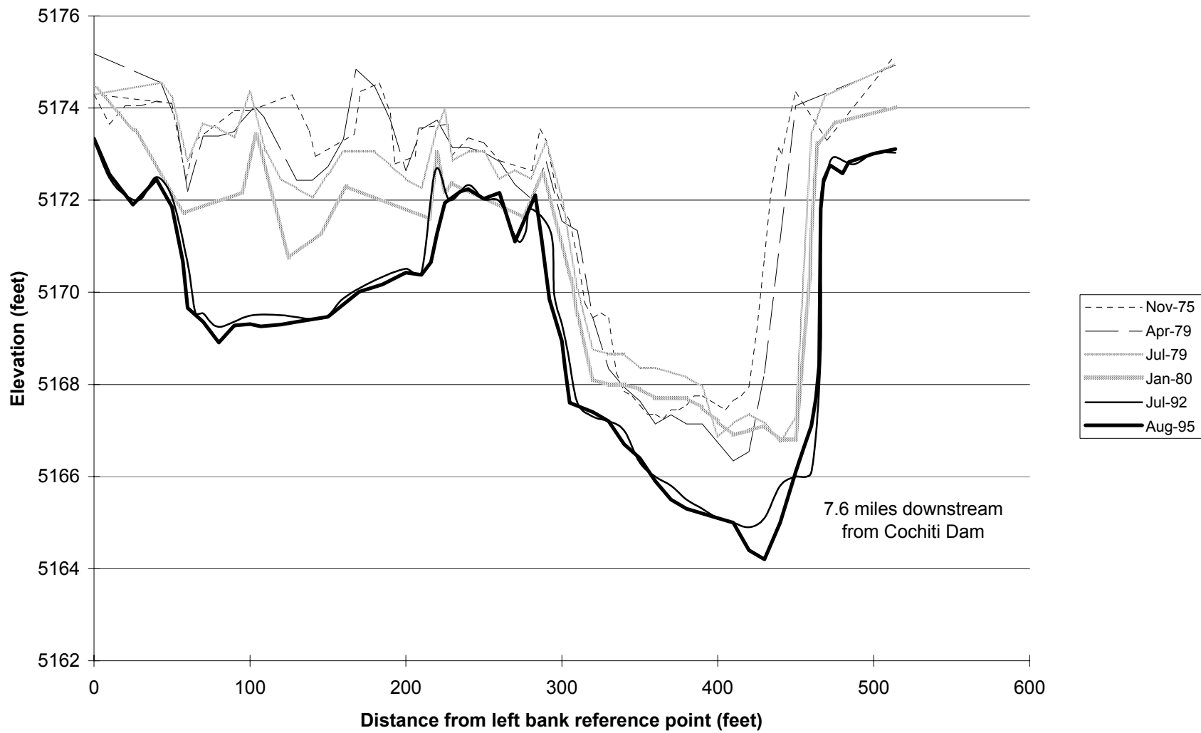
Fig.D-5. Cross Section CO-8.
