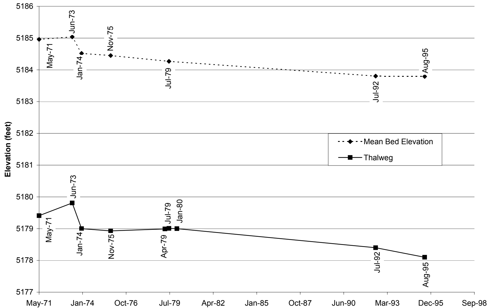
Fig. E-5. Change in thalweg elevation and mean bed elevation with time at cross section CO-6.
