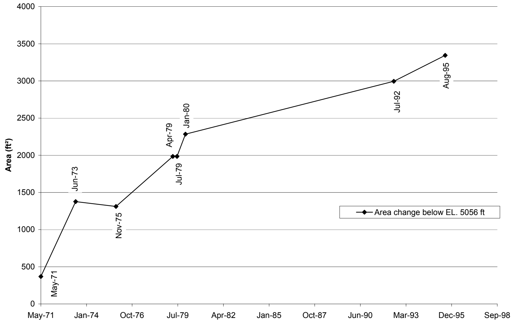
Fig. E-56. Change in cross section area with time at cross section CO-29.
