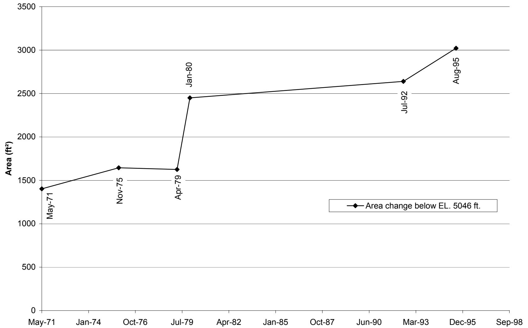
Fig. E-57. Change in cross section area with time at cross section CO-30.
