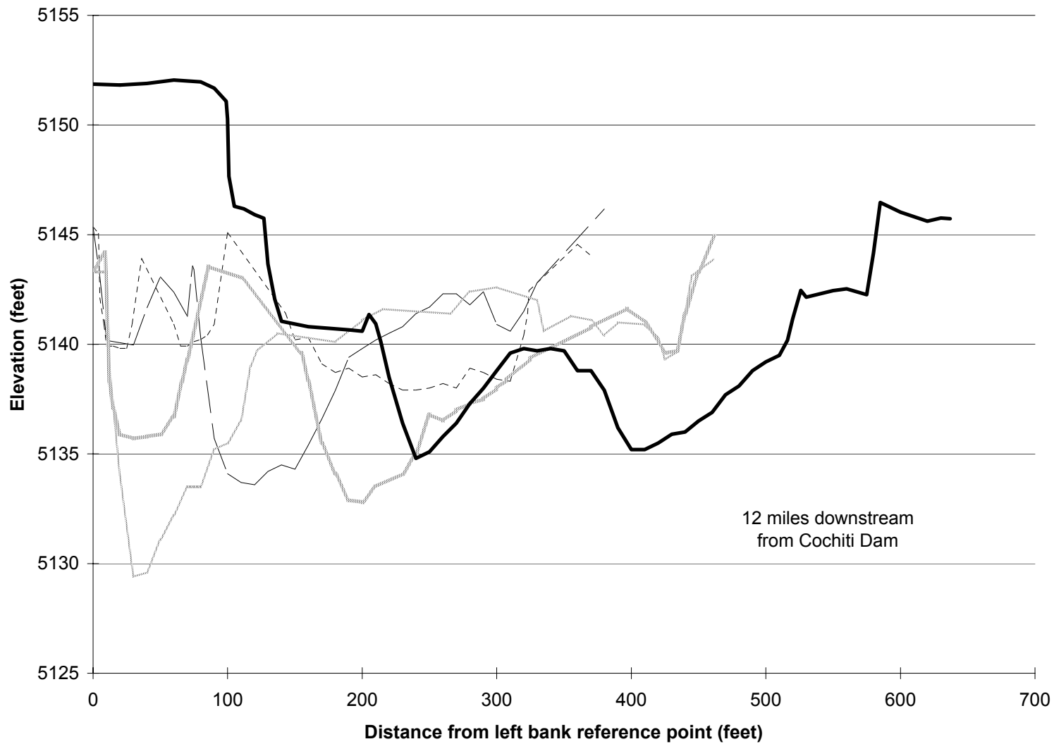
Fig.D-8. Cross Section CO-13.
