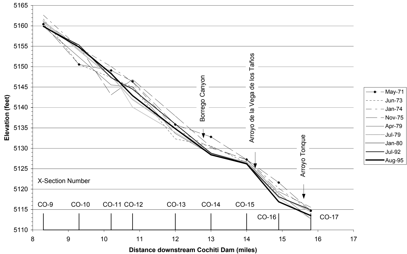
Fig. 3.10. Thalweg profile from cross section CO-9 to cross section CO-17
