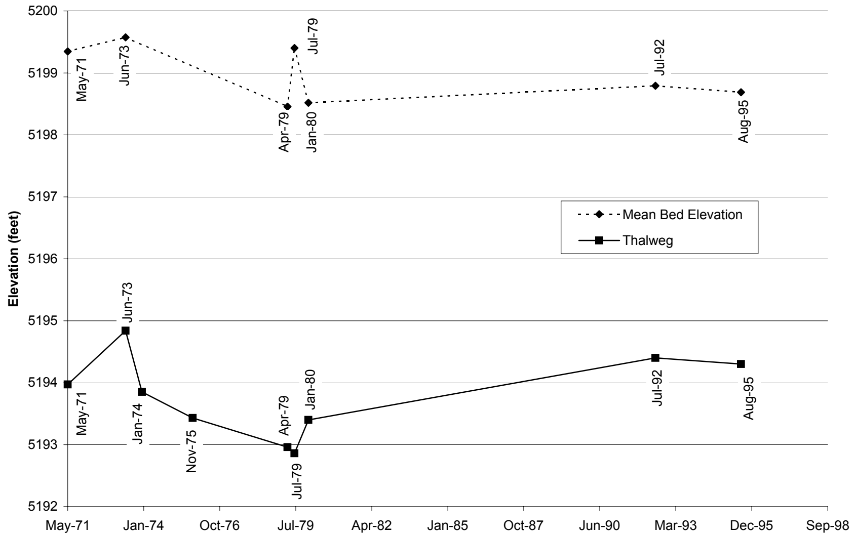
Fig. E-3. Change in thalweg elevation and mean bed elevation with time at cross section CO-4.
