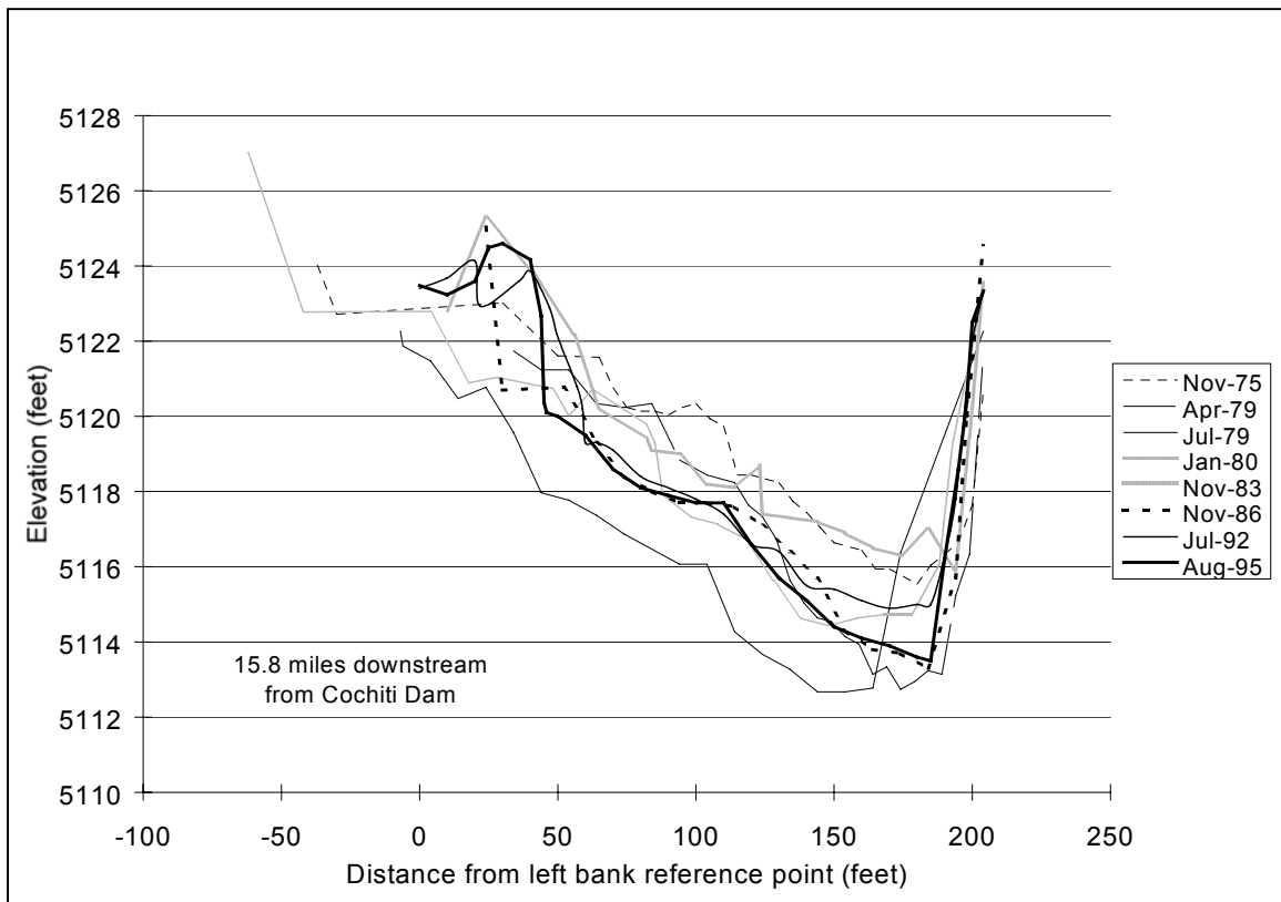
Fig. 4.7. Cross section CO-17.
