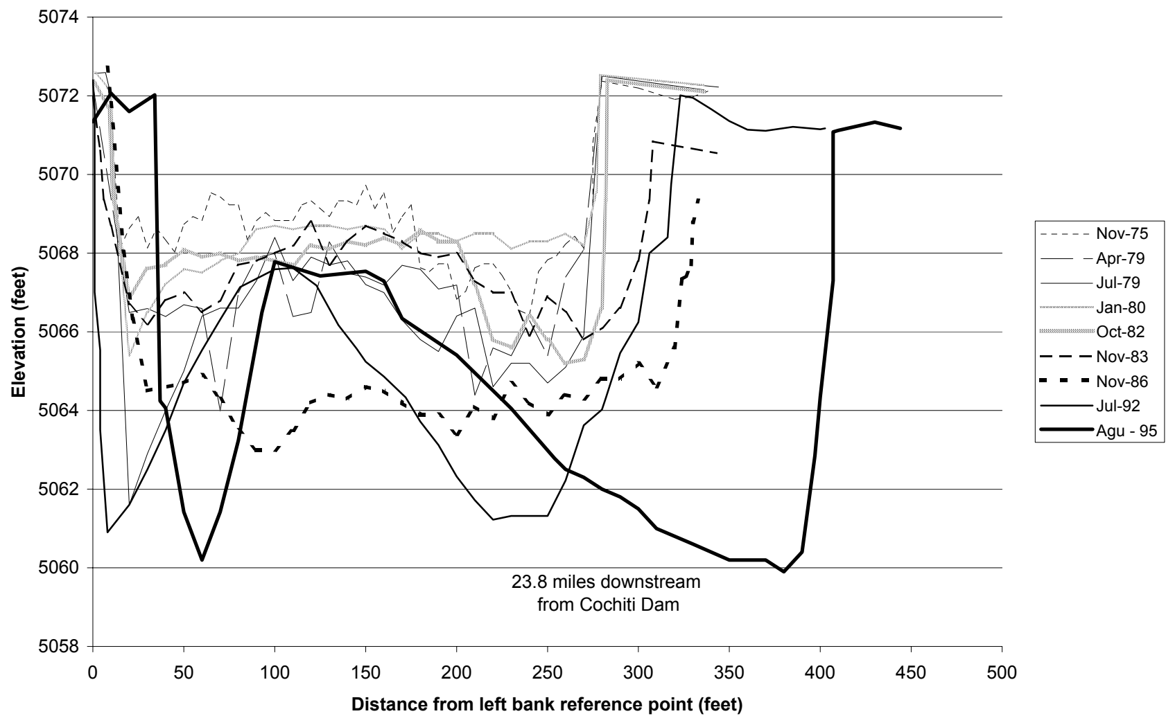
Fig.D-16. Cross Section CO-26
