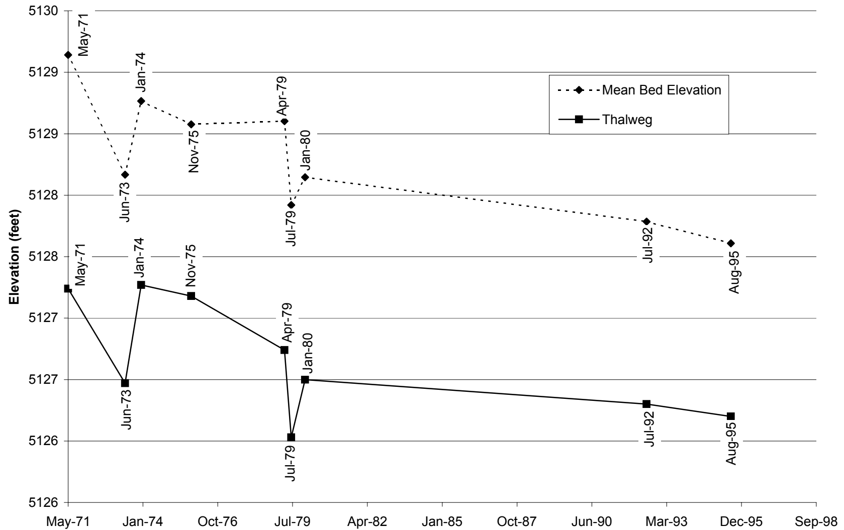
Fig. E-13. Change in thalweg elevation and mean bed elevation with time at cross section CO-15.
