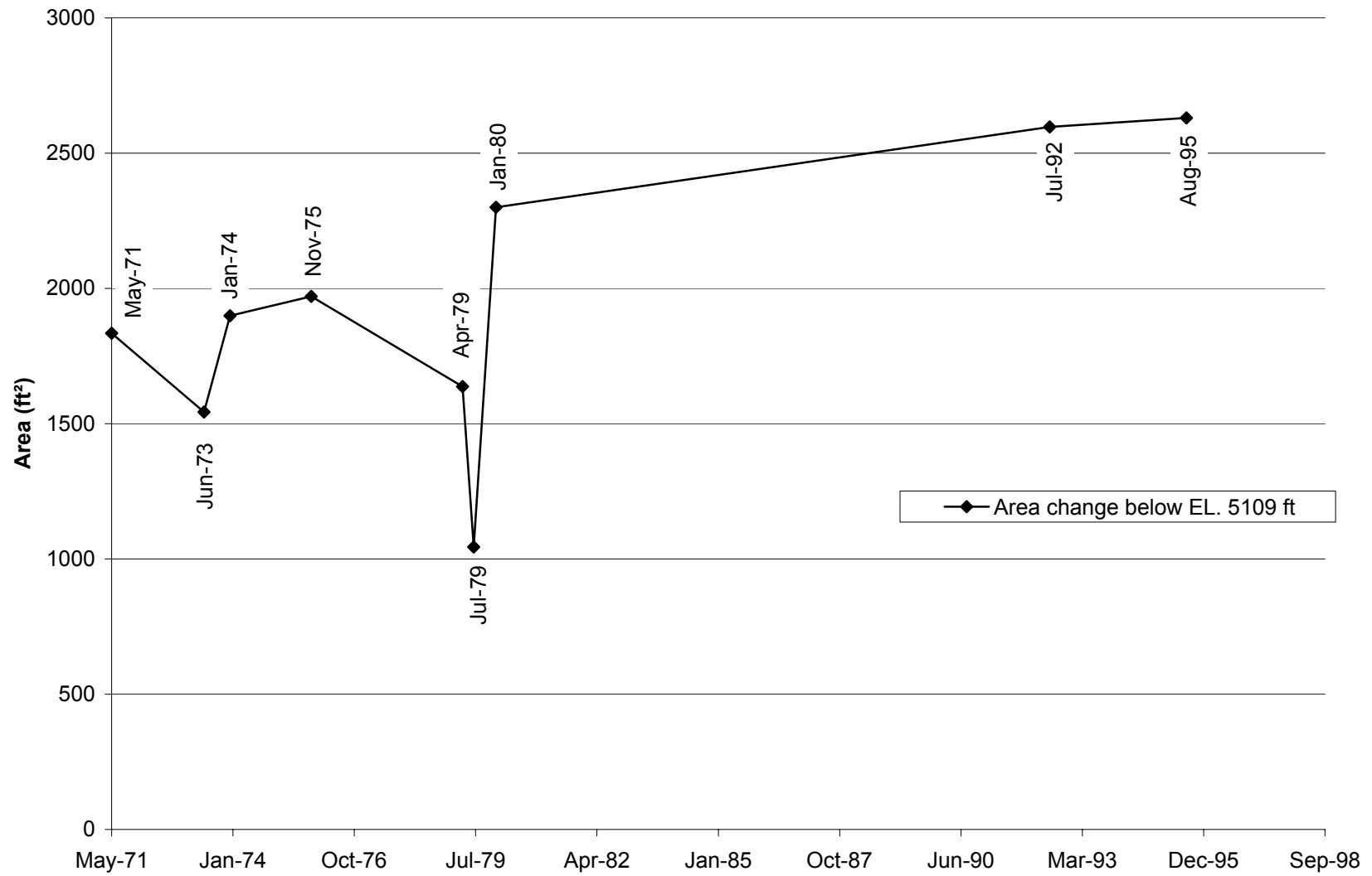
Fig. E-46. Change in cross section area with time at cross section CO-19.
