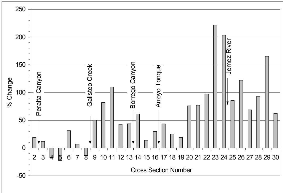
Fig. 3.15. Pre-dam to Post-dam change in cross sectional area.
