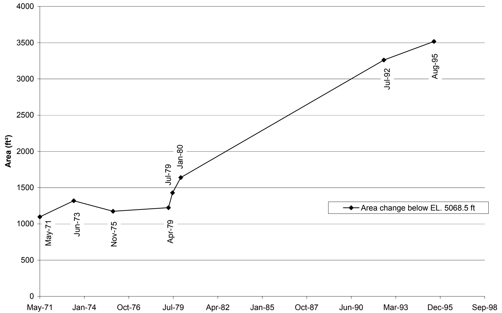
Fig. E-54. Change in cross section area with time at cross section CO-27.
