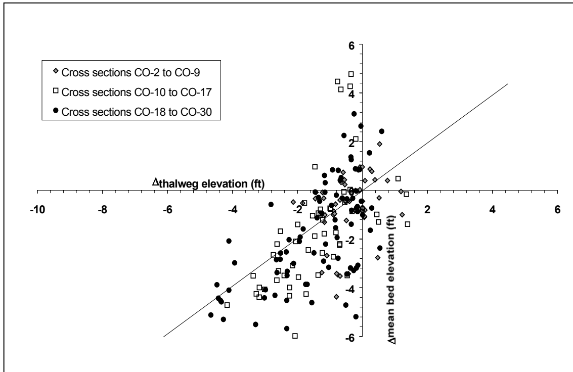
Fig. 3.14. Change referenced to 1971 in mean bed elevation against change referenced to 1971 in thalweg elevation.
