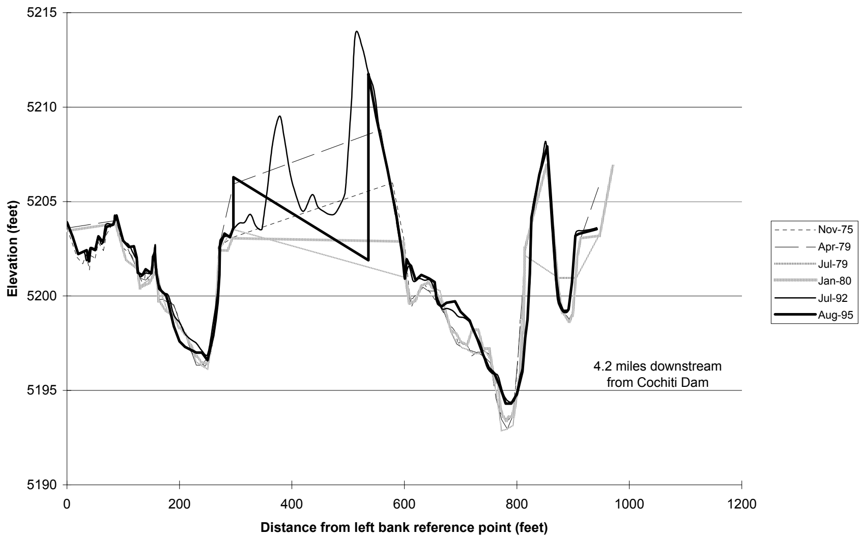
Fig.D-2. Cross Section CO-4.
