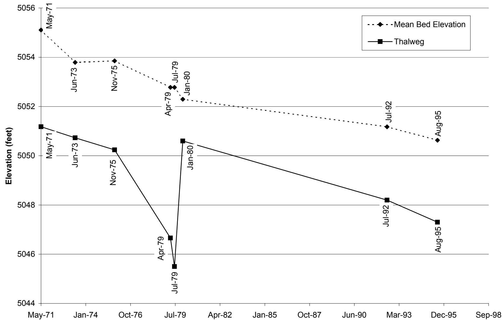
Fig. E-27. Change in thalweg elevation and mean bed elevation with time at cross section CO-29.
