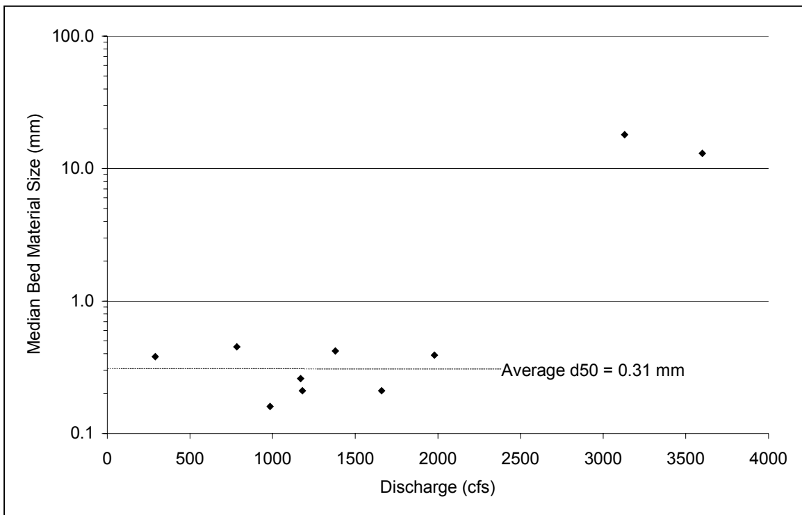
Fig. 3.23. Median bed material size versus discharge at Rio Grande at San Felipe gaging station from 1970 to 1974.
