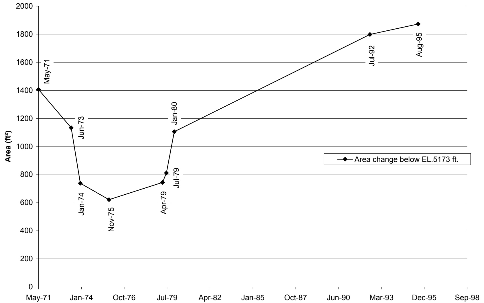
Fig. E-35. Change in cross section area with time at cross section CO-8.
