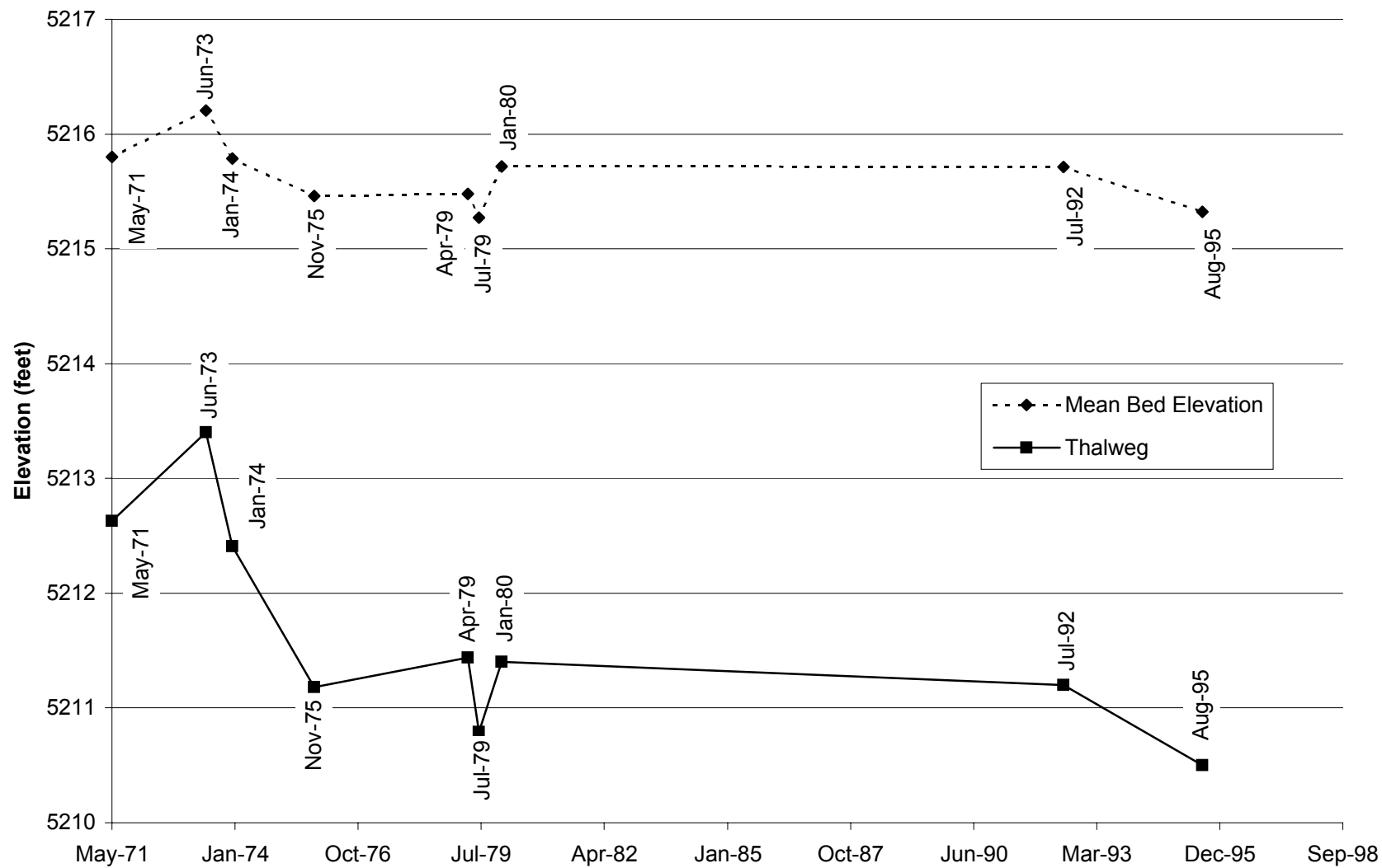
Fig. E-1. Change in thalweg elevation and mean bed elevation with time at cross section CO-2.
