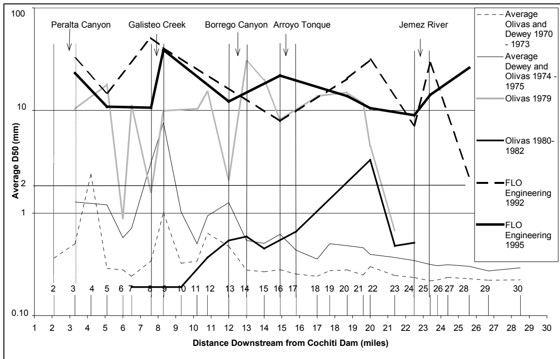
Fig. 3.16. Median bed material size downstream Cochiti Dam from 1970 to 1995.
