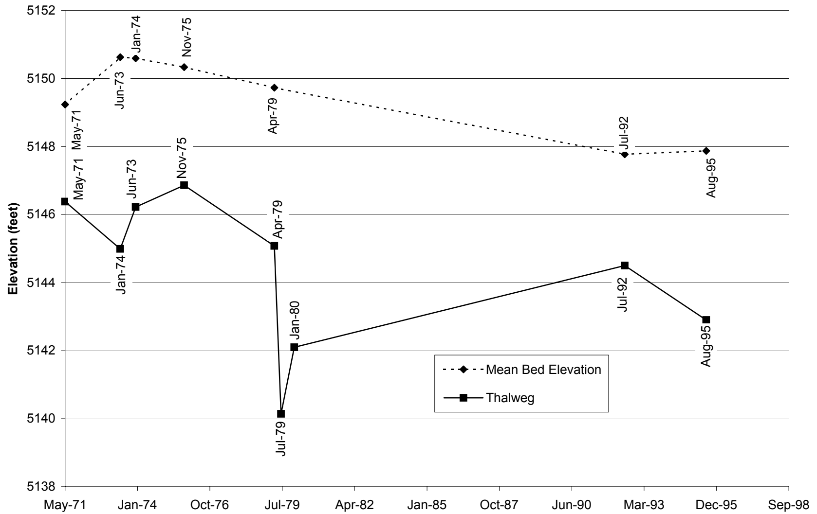
Fig. E-10. Change in thalweg elevation and mean bed elevation with time at cross section CO-12.
