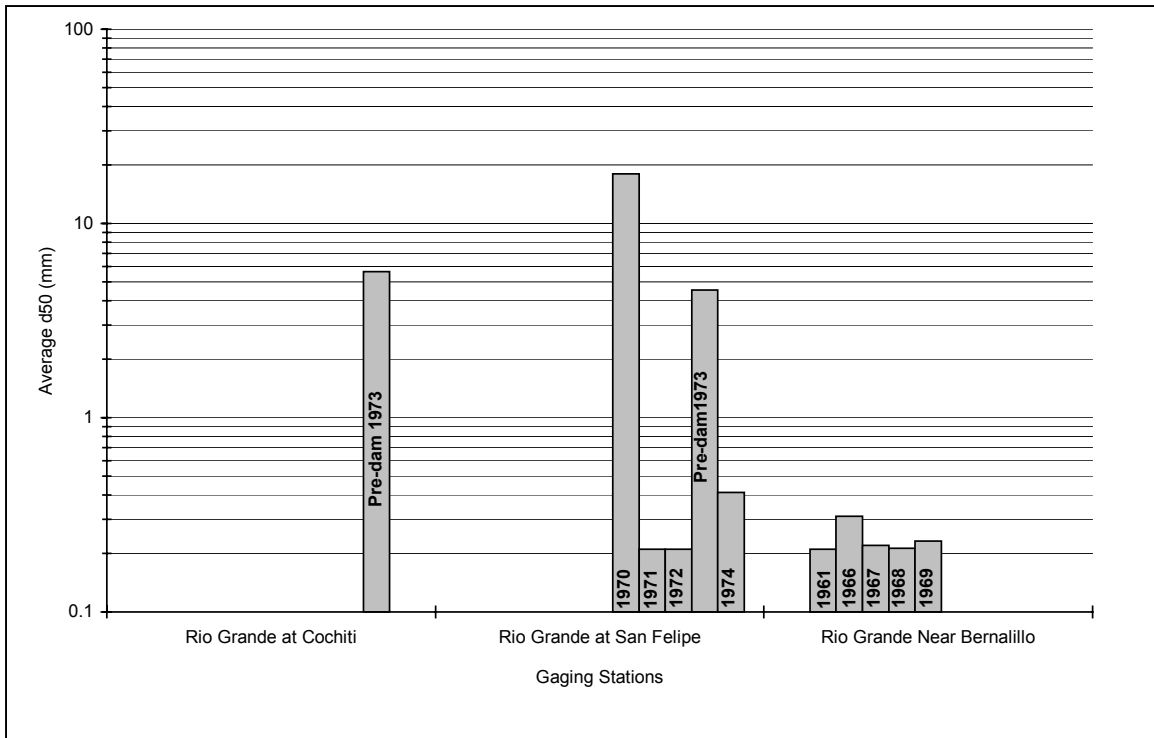
Fig. 3.22. Median bed material size at USGS gaging stations from 1961 to 1973.
