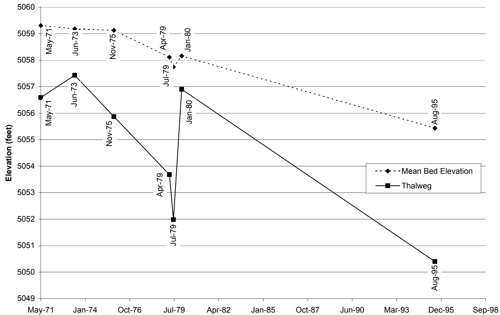
Fig. E-26. Change in thalweg elevation and mean bed elevation with time at cross section CO-28.
