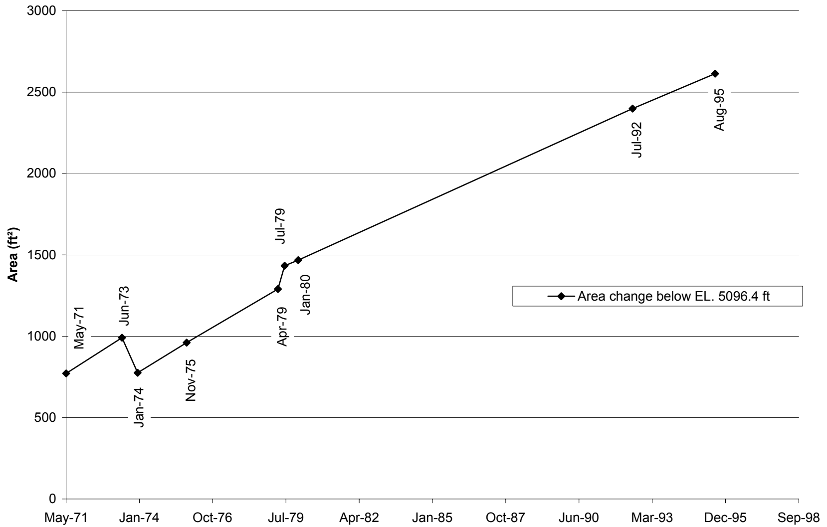
Fig. E-48. Change in cross section area with time at cross section CO-21.
