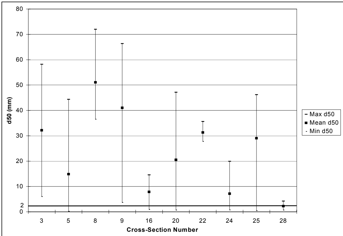
Fig. 3.20. 1992 median bed material size data.
