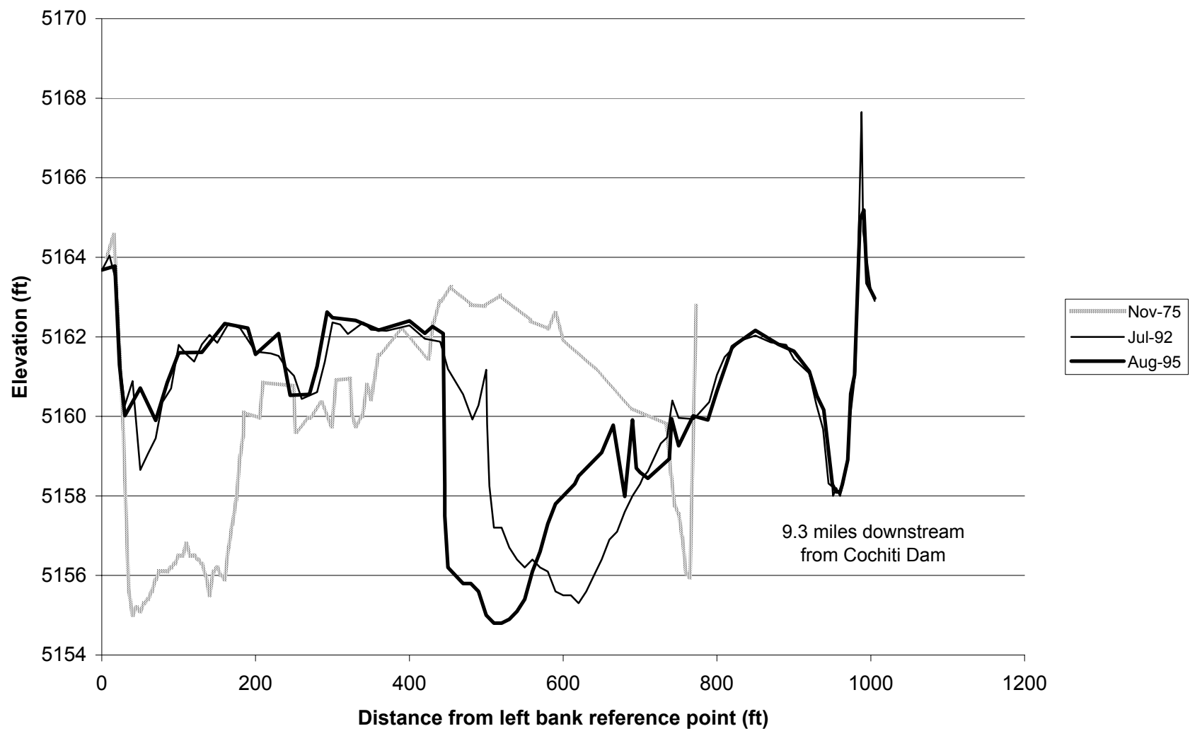
Fig.D-6. Cross Section CO-10.
