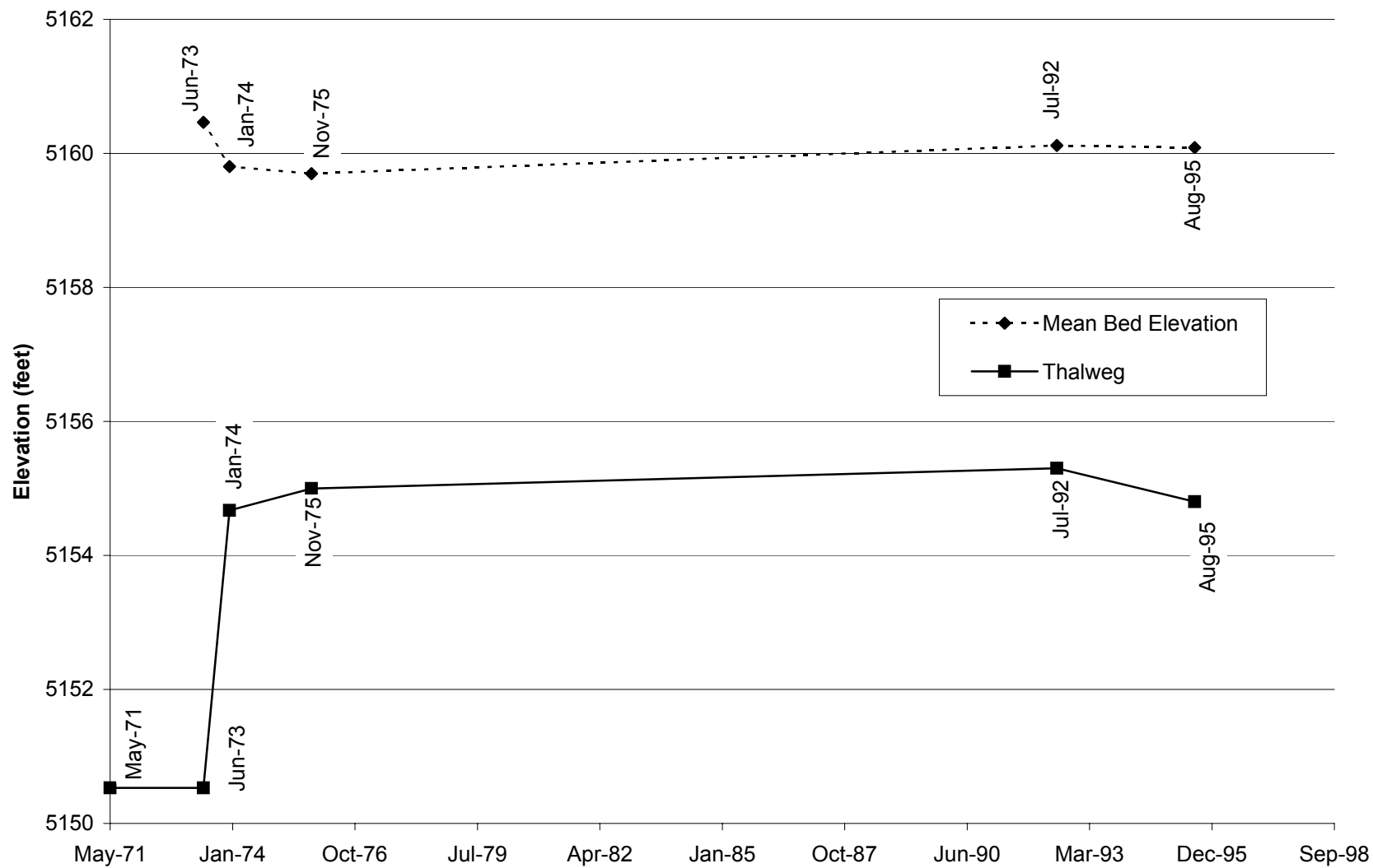
Fig. E-9. Change in thalweg elevation and mean bed elevation with time at cross section CO-10.
