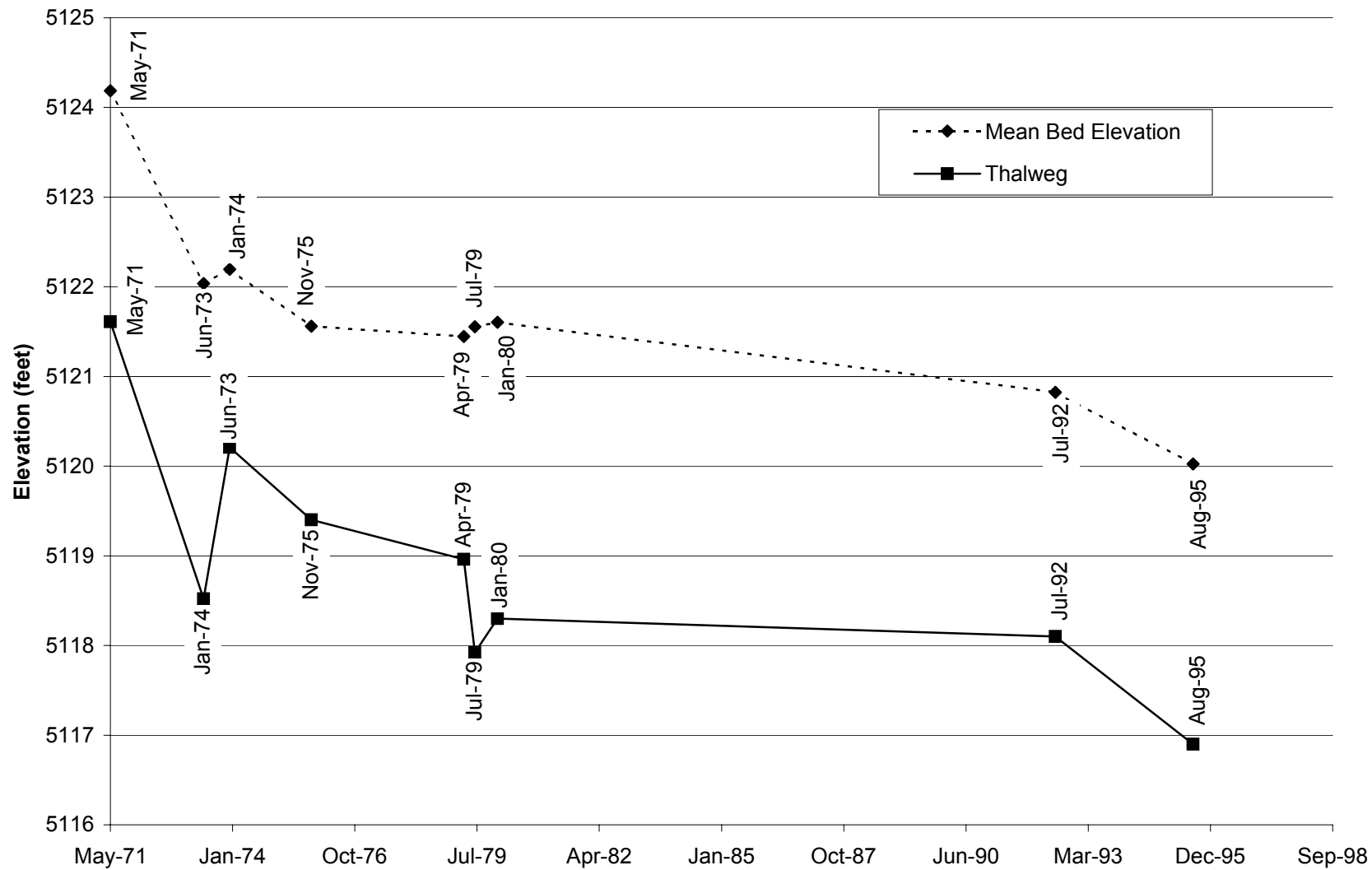
Fig. E-14. Change in thalweg elevation and mean bed elevation with time at cross section CO-16.
