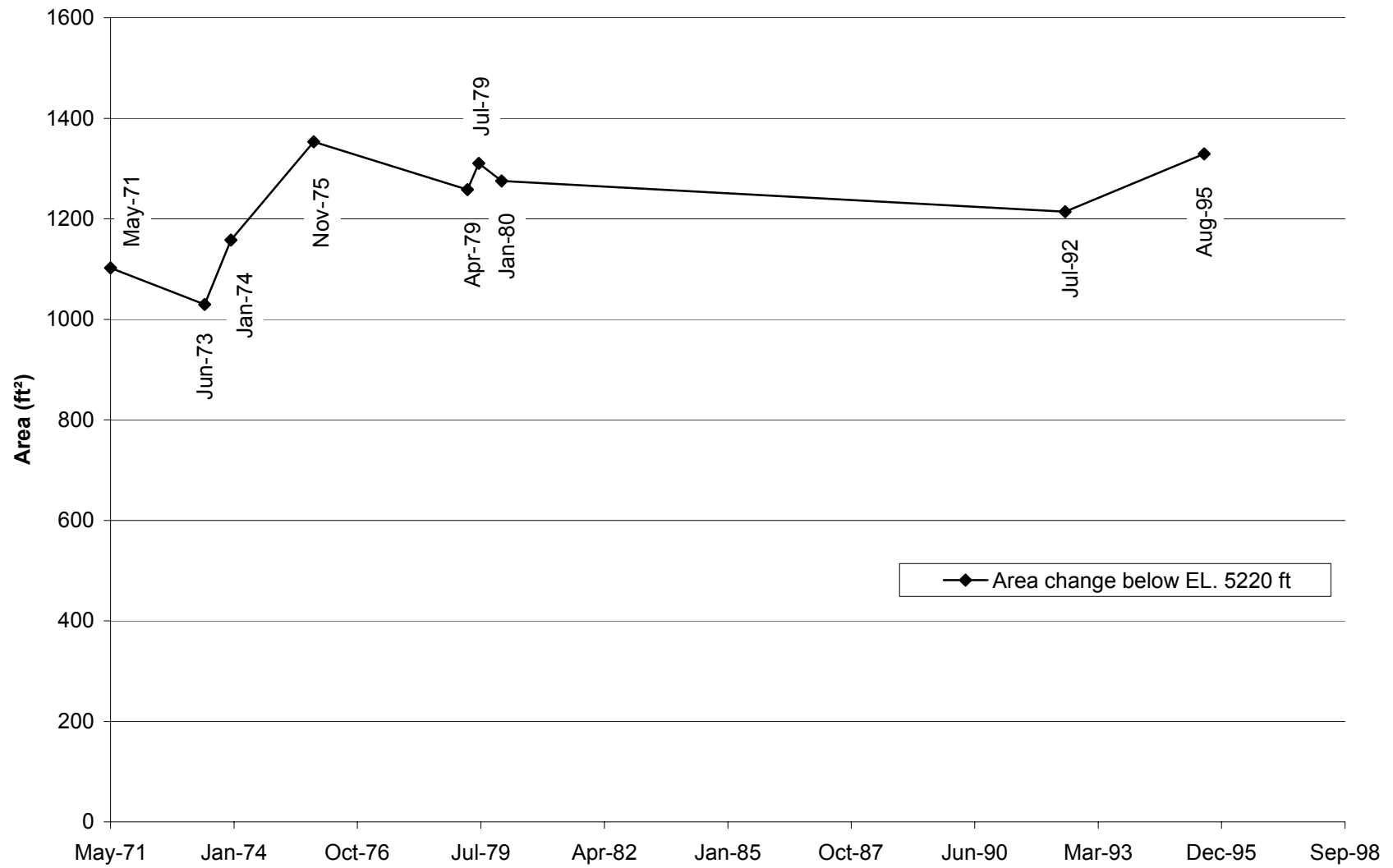
Fig.E-29. Change in cross section area with time at cross section CO-2.
