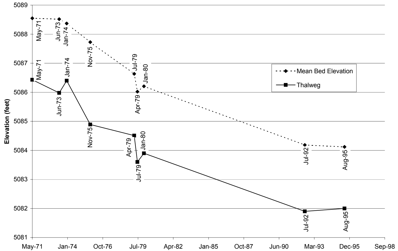
Fig. E-20. Change in thalweg elevation and mean bed elevation with time at cross section CO-22.
