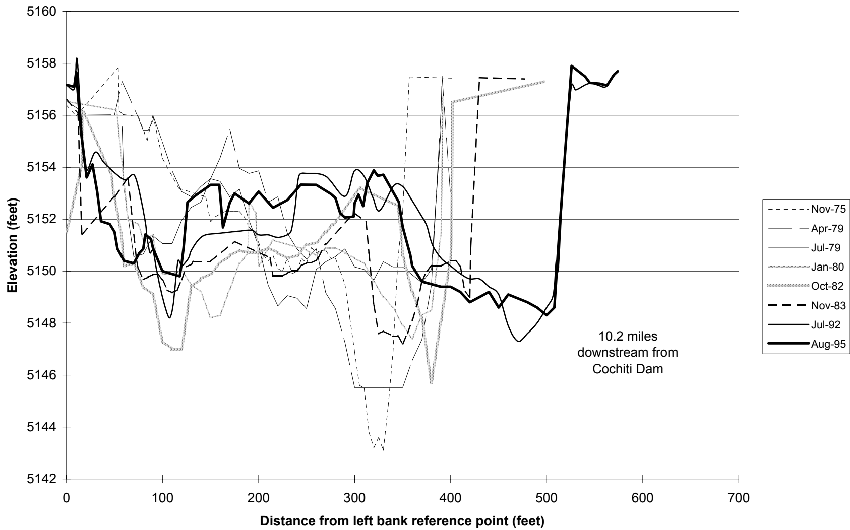
Fig.D-7. Cross Section CO-11.
