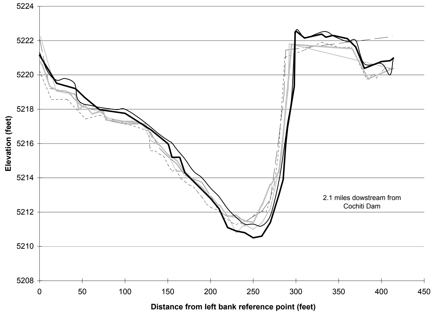
Fig. D-1. Cross Section CO-2.
