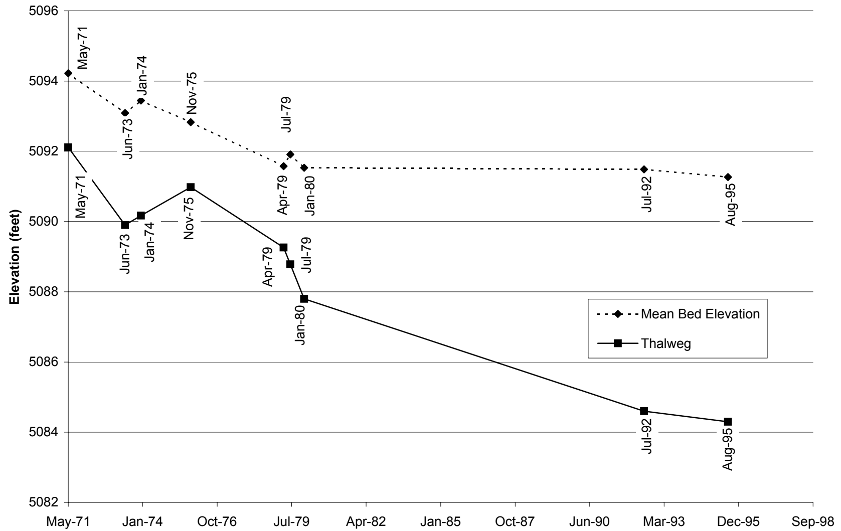
Fig. E-19. Change in thalweg elevation and mean bed elevation with time at cross section CO-21.
