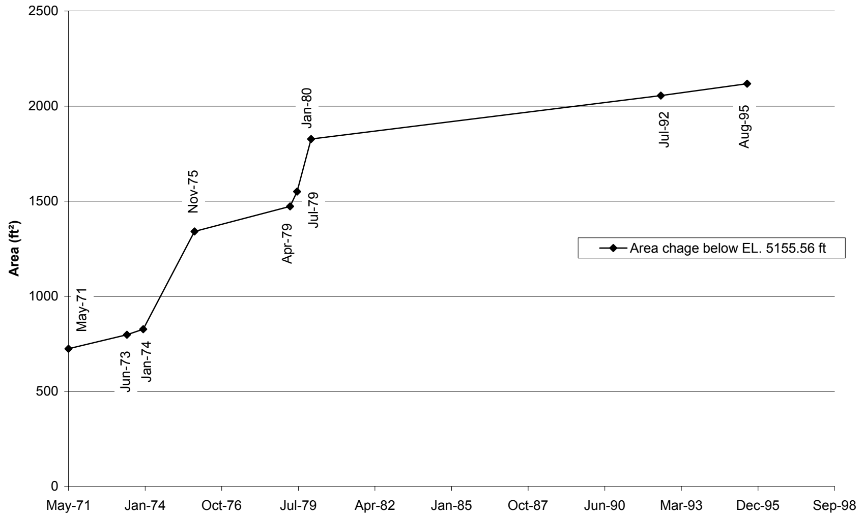
Fig. E-38. Change in cross section area with time at cross section CO-11.
