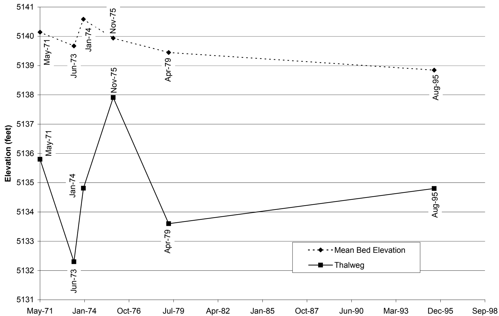
Fig. E-11. Change in thalweg elevation and mean bed elevation with time at cross section CO-13.
