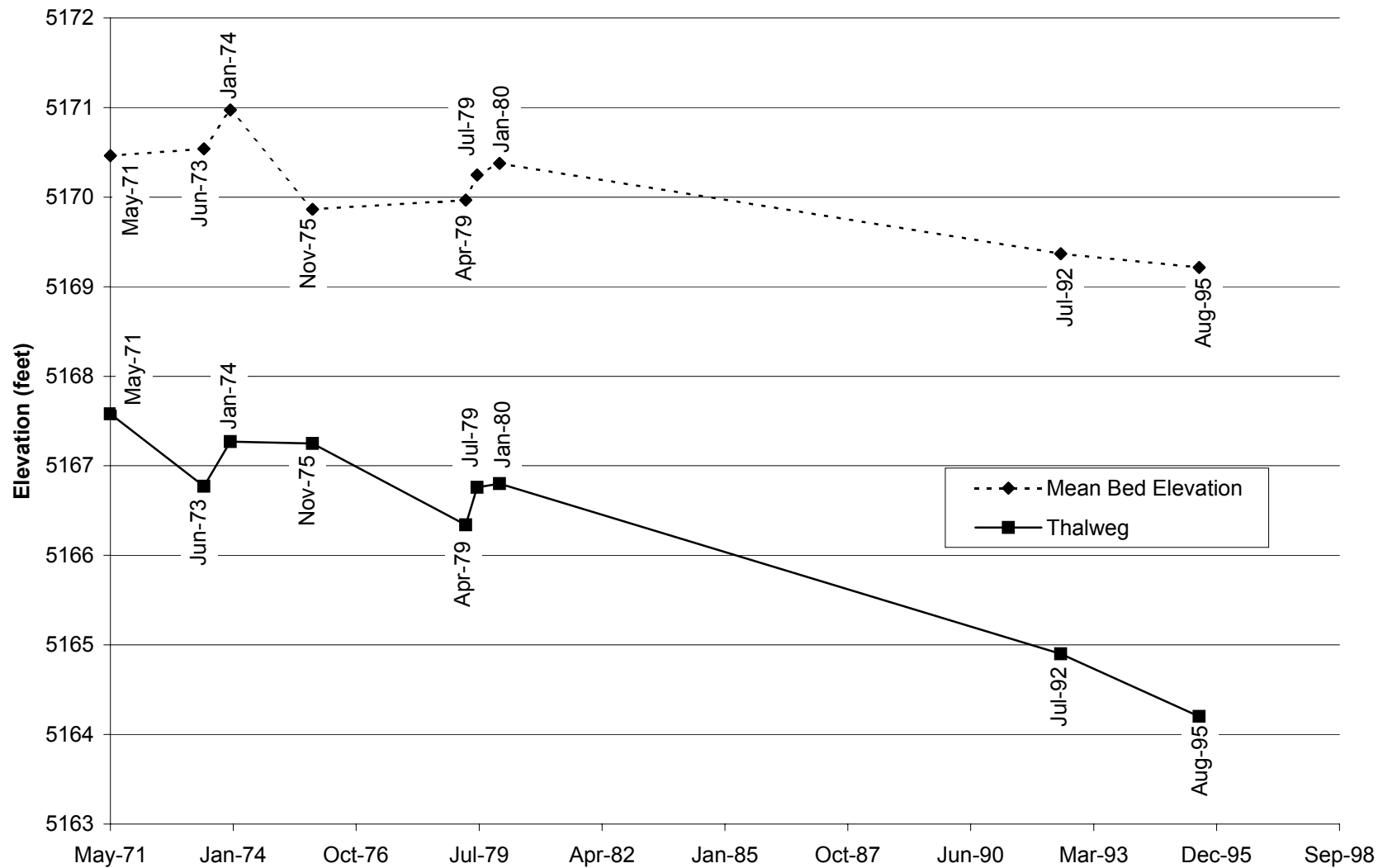
Fig. E-7. Change in thalweg elevation and mean bed elevation with time at cross section CO-8.
