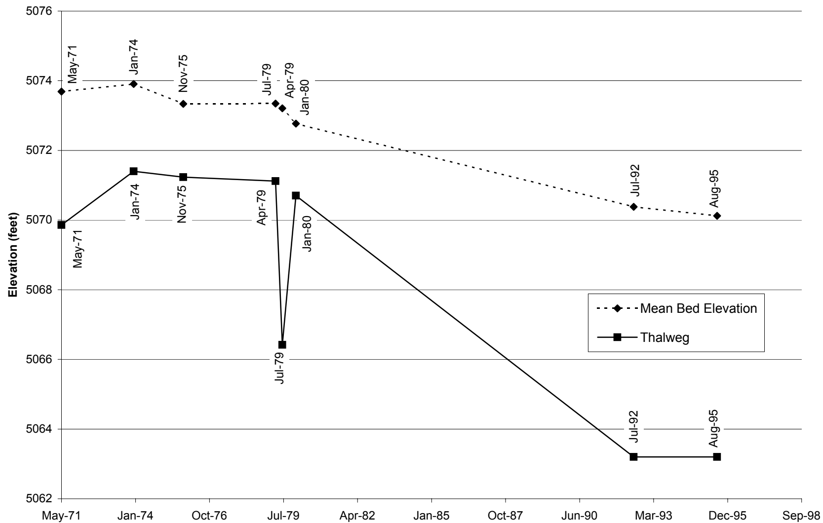
Fig. E-23. Change in thalweg elevation and mean bed elevation with time at cross section CO-25.
