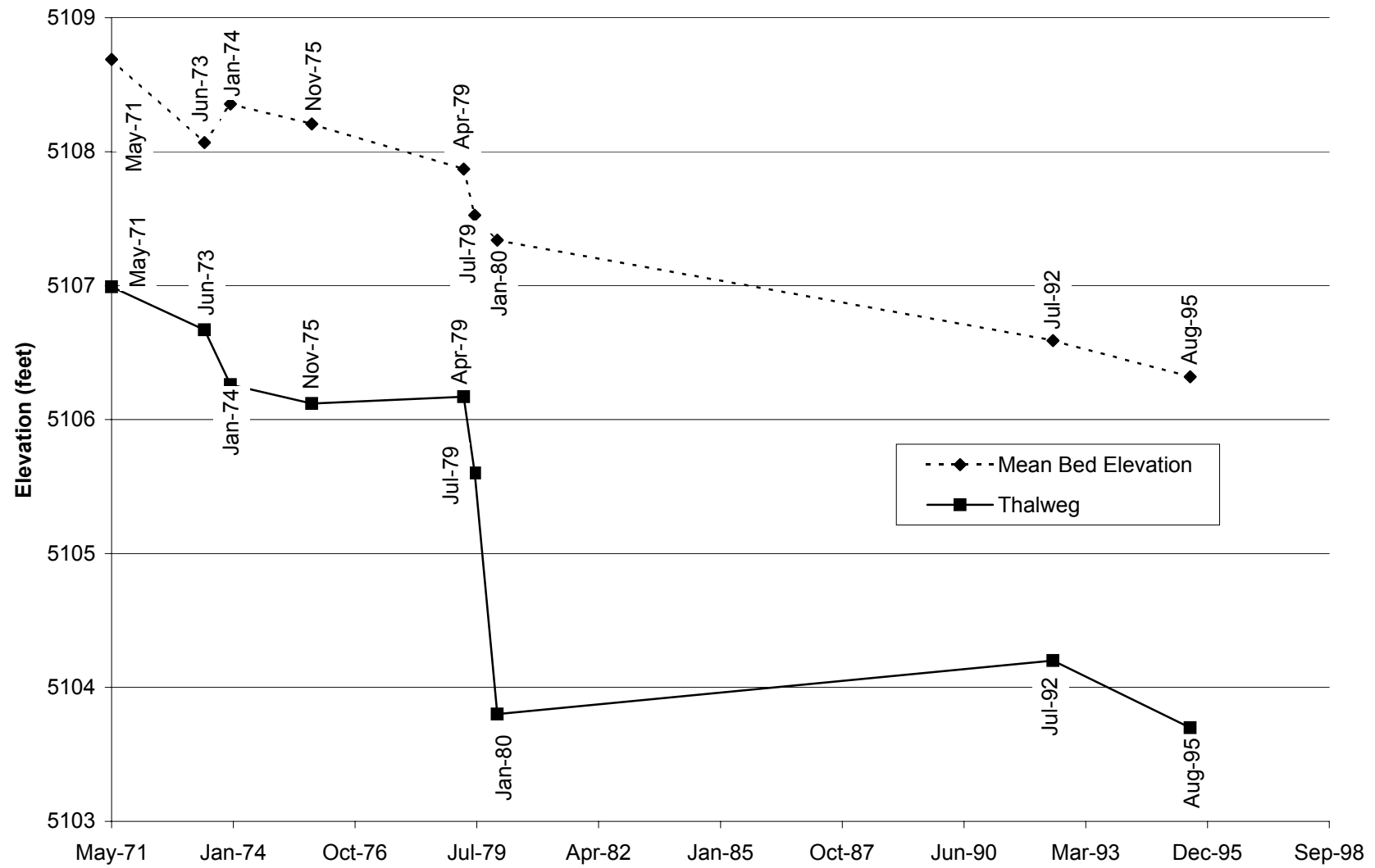
Fig. E-16. Change in thalweg elevation and mean bed elevation with time at cross section CO-18.
