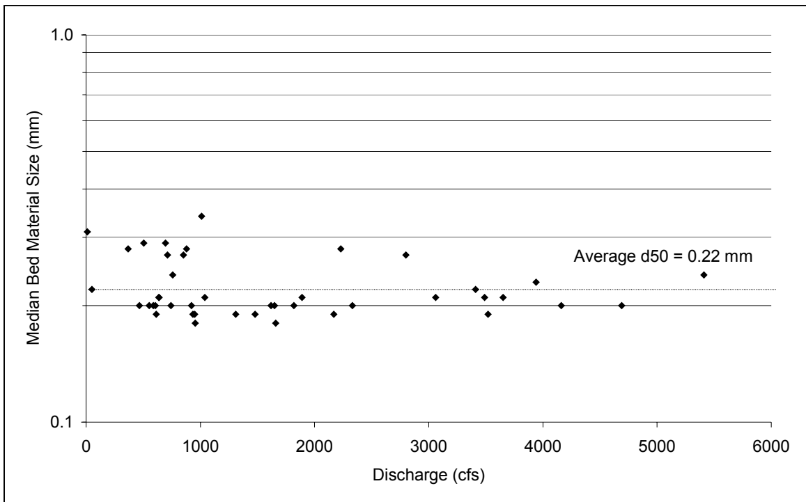
Fig. 3.24. Median bed material size versus discharge at Rio Grande near Bernalillo station from 1961 to 1969.
