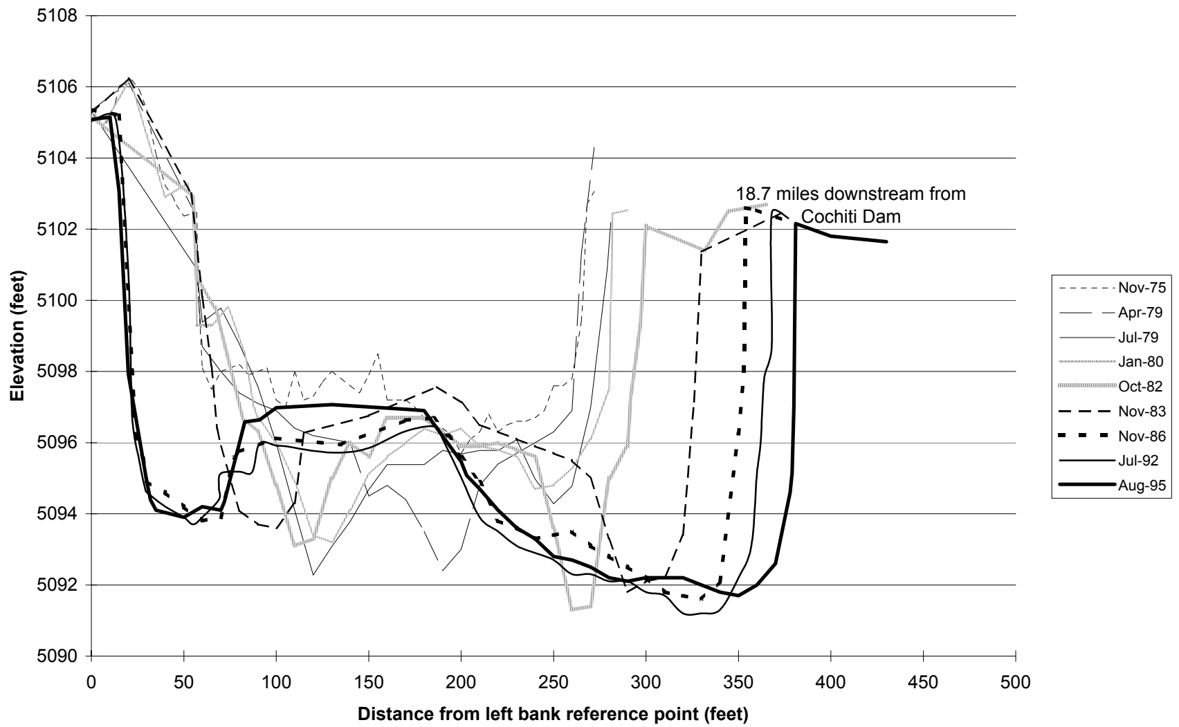
Fig.D-12. Cross Section CO-20
