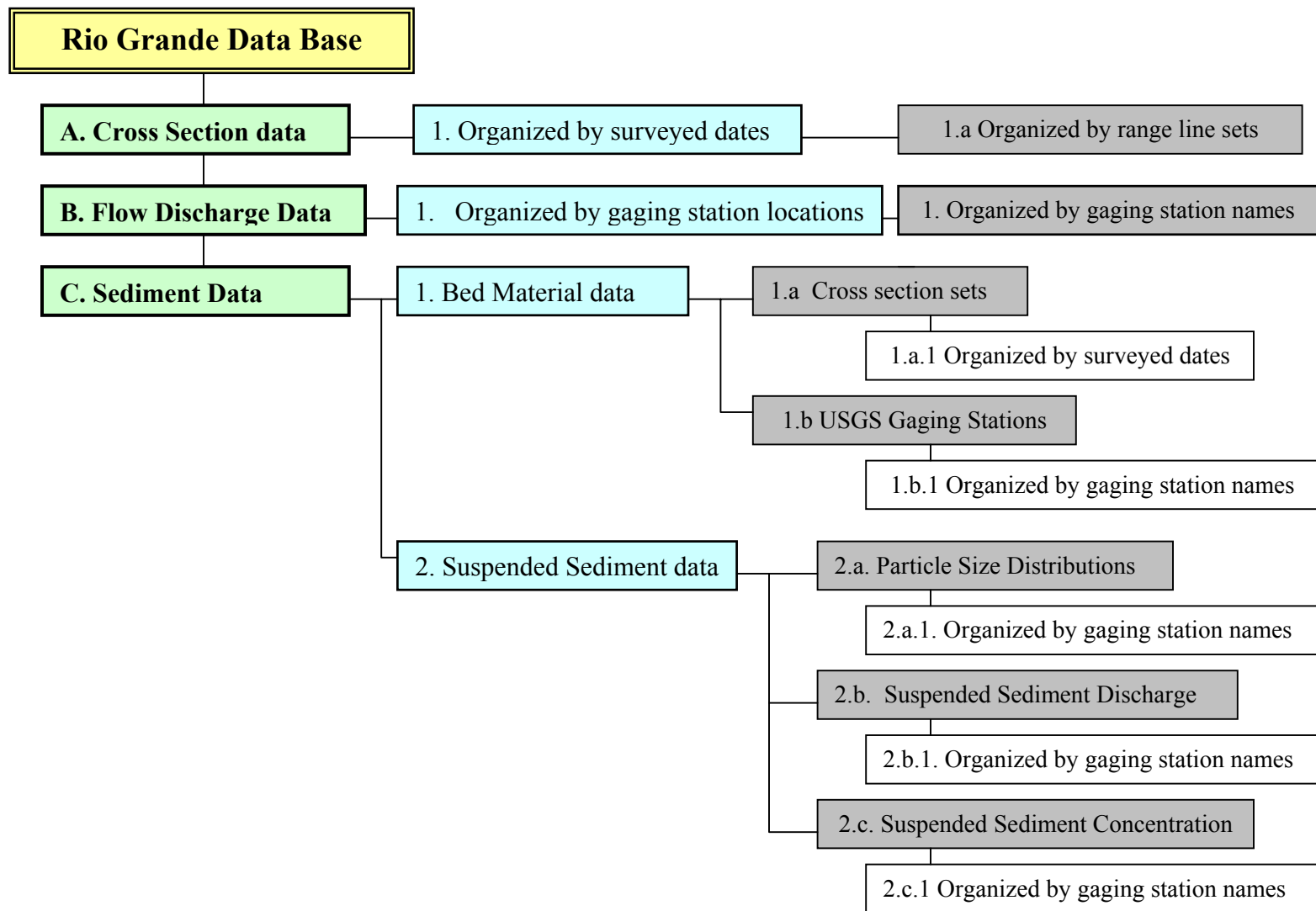
Fig. 3.1. Diagram of the computer data base.
