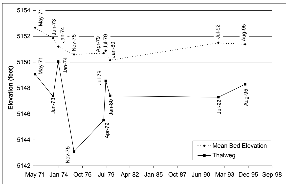
Fig. 4.1. Change in thalweg and mean bed elevation with time at cross section CO-11.
