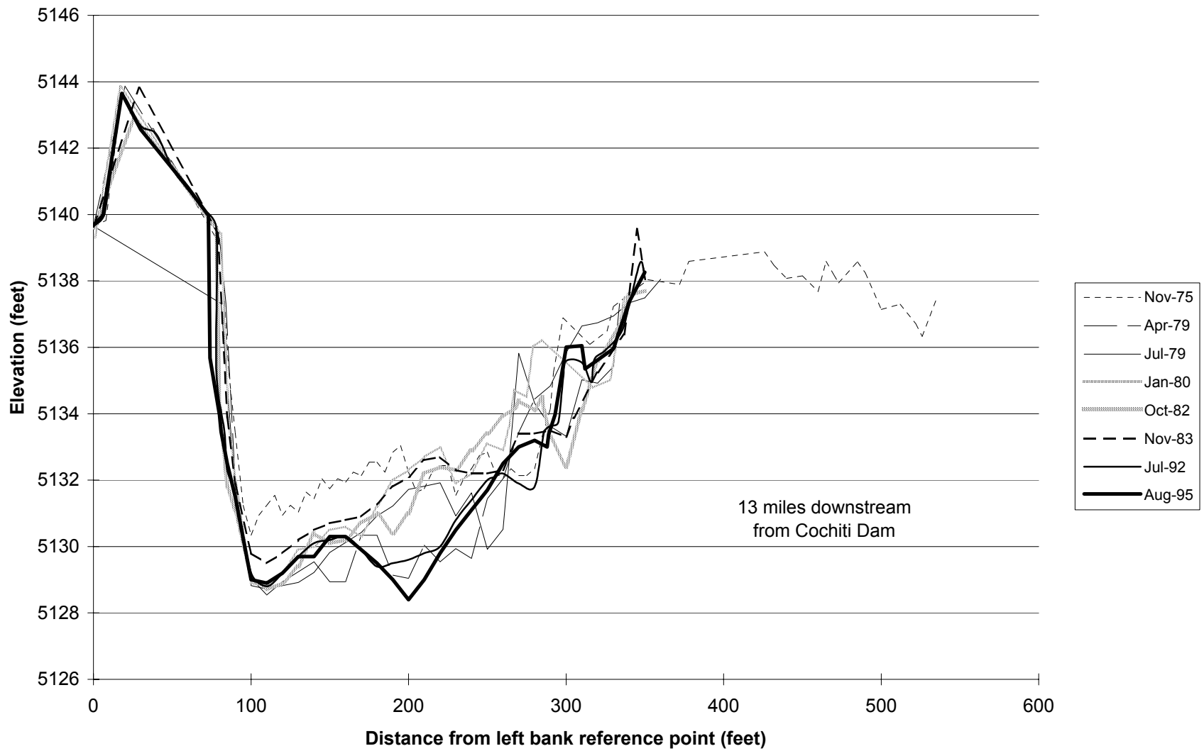
Fig.D-9. Cross Section CO-14.
