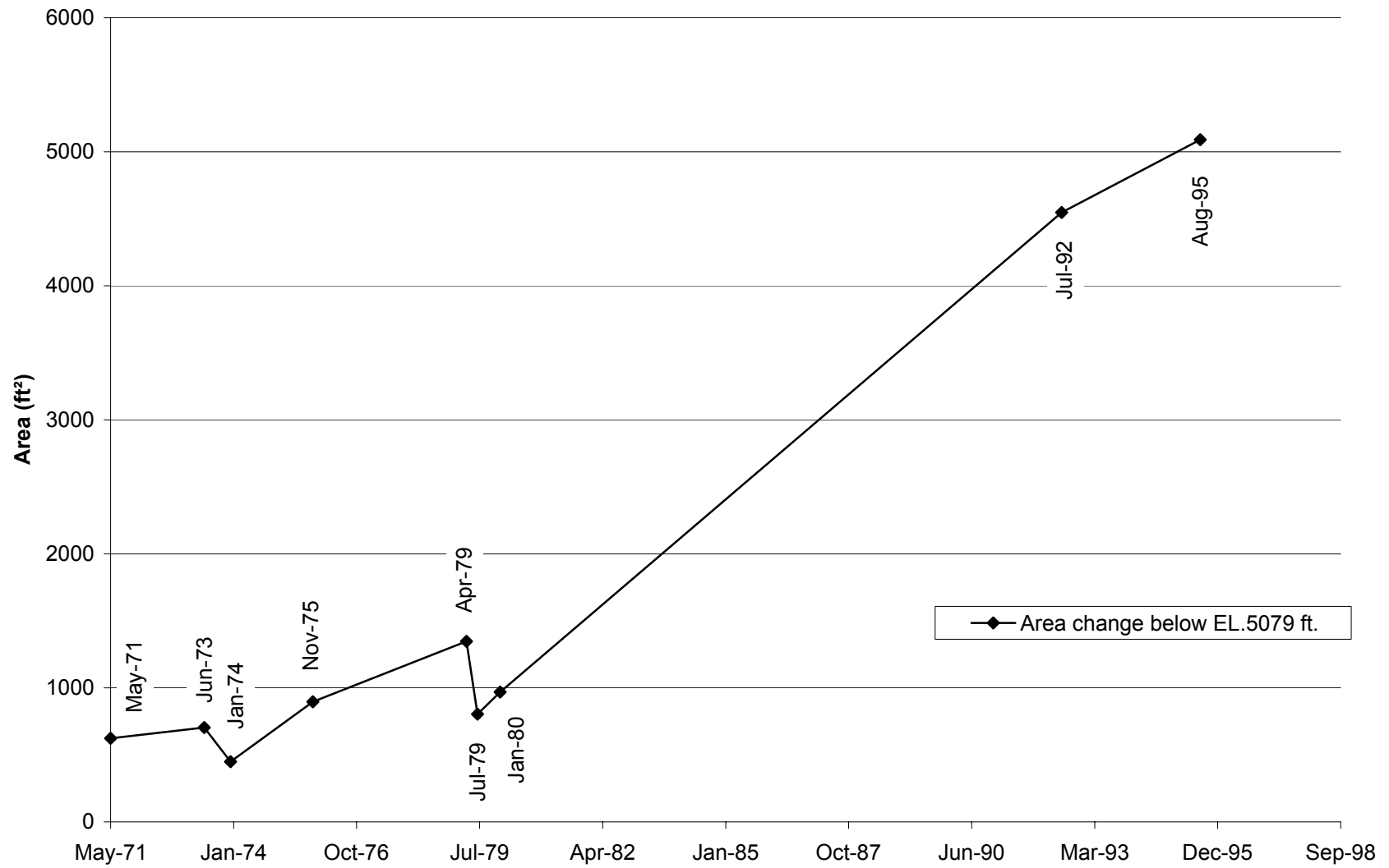
Fig. E-51. Change in cross section area with time at cross section CO-24.
