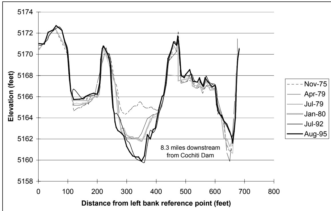
Fig. 4.4. Cross section CO-9.
