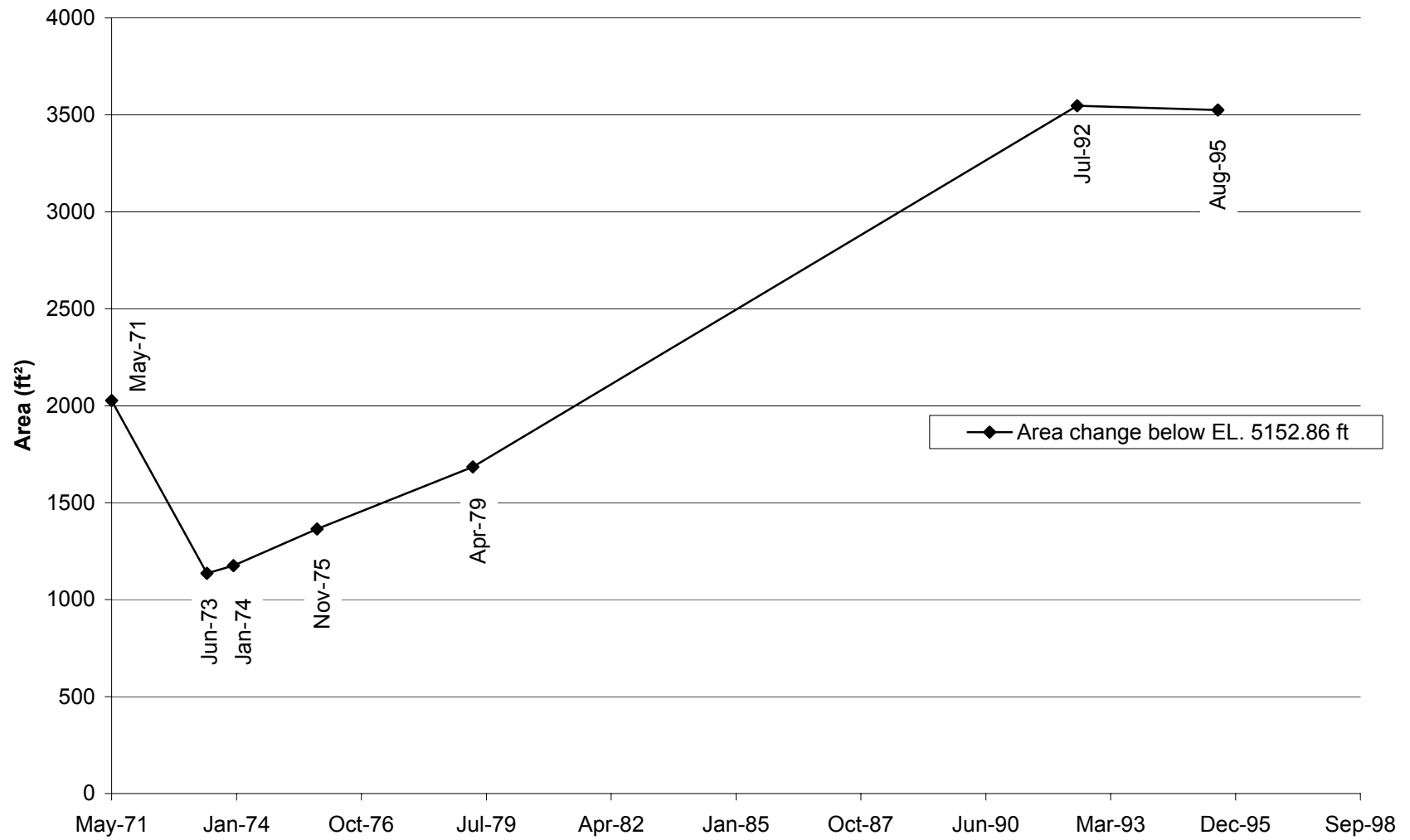
Fig. E-39. Change in cross section area with time at cross section CO-12.
