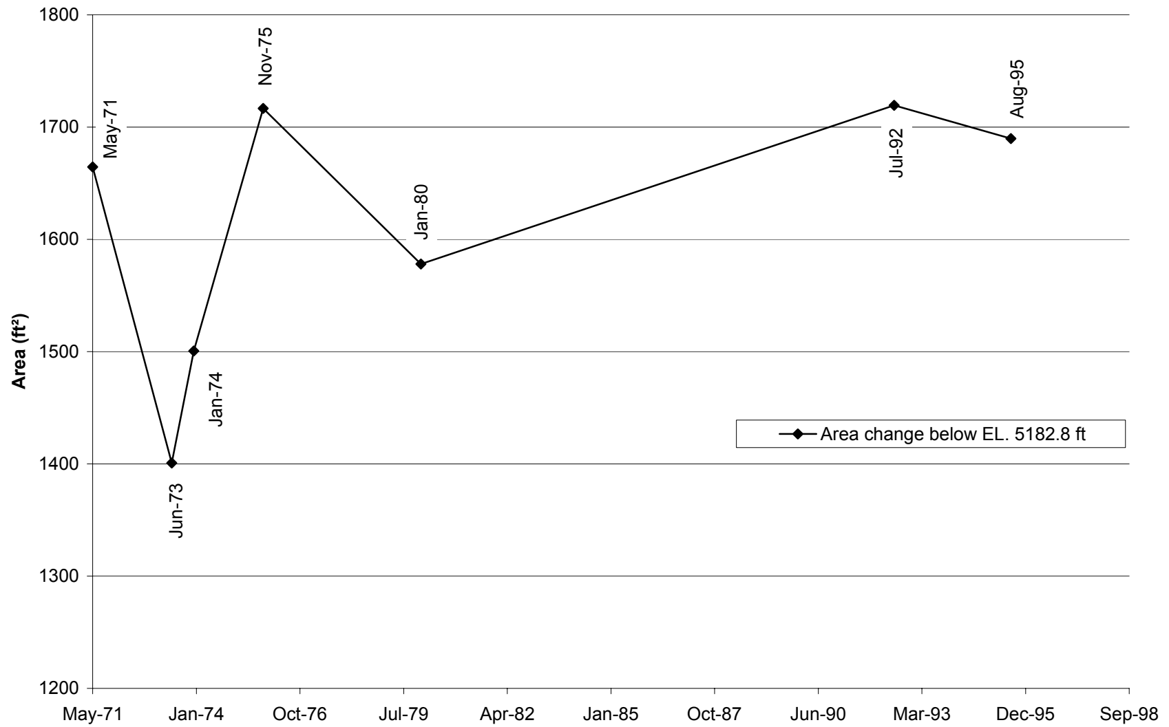
Fig. E-34. Change in cross section area with time at cross section CO-7.
