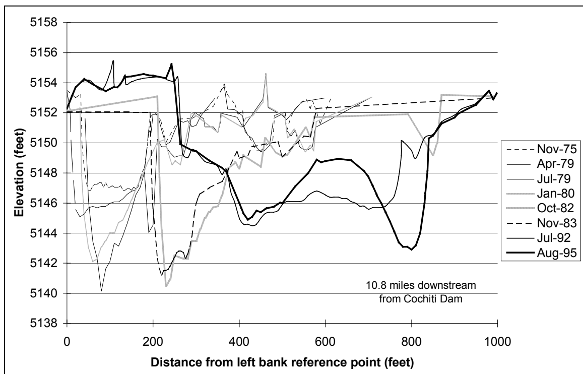
Fig. 4.5. Cross section CO-12.
