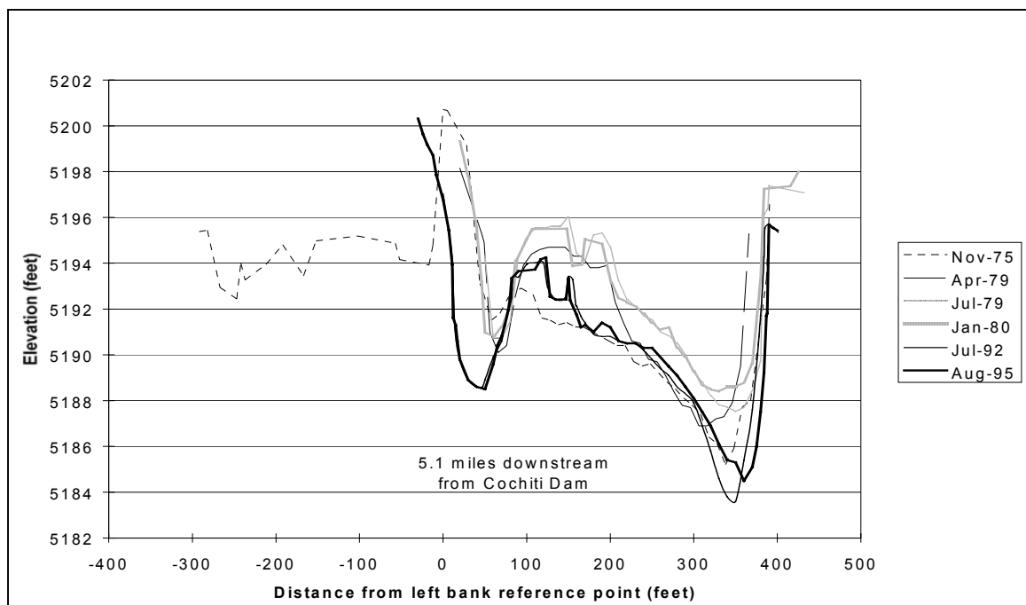
Fig. 4.3. Cross section CO-5.
