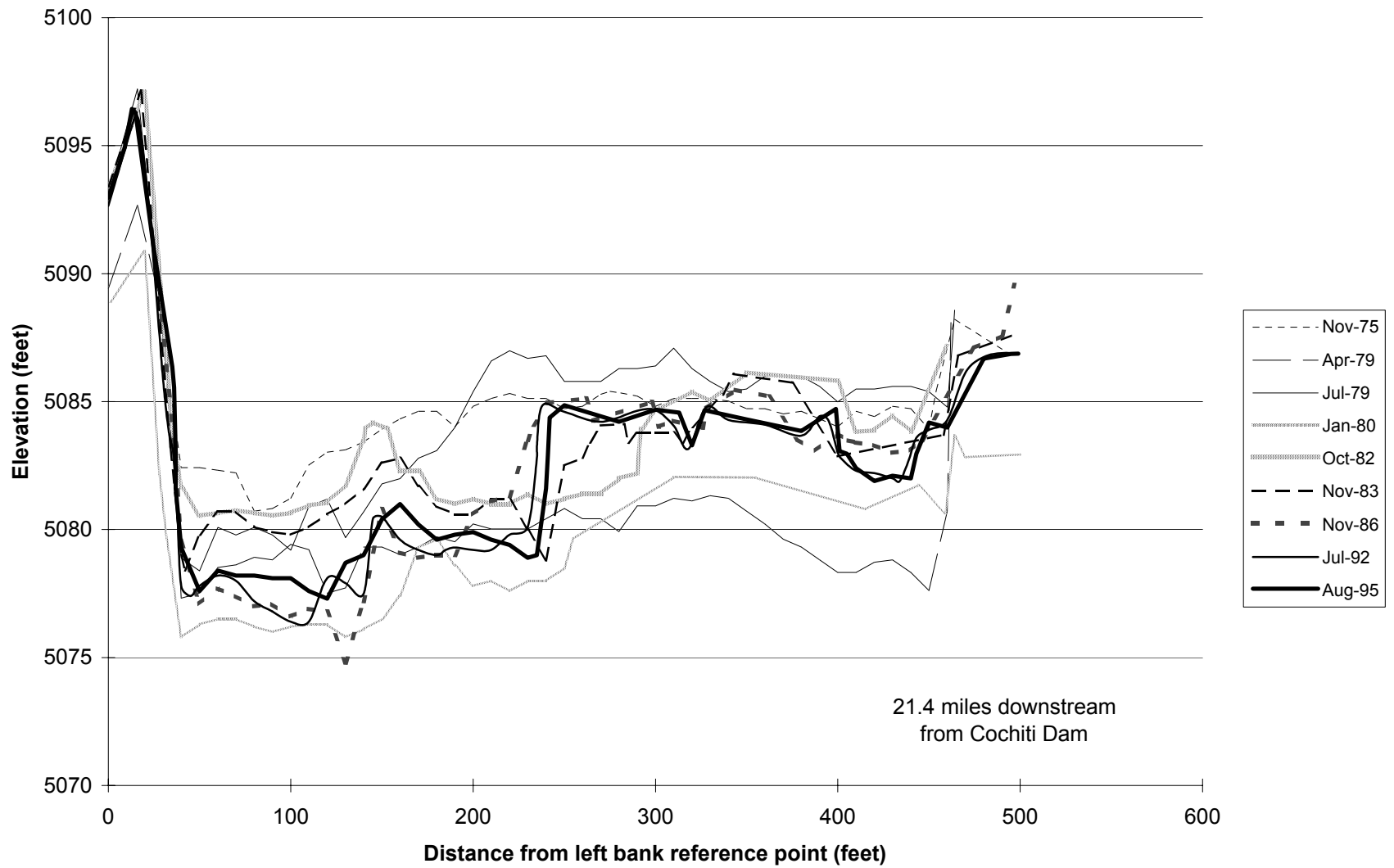
Fig.D-14. Cross Section CO-23.
