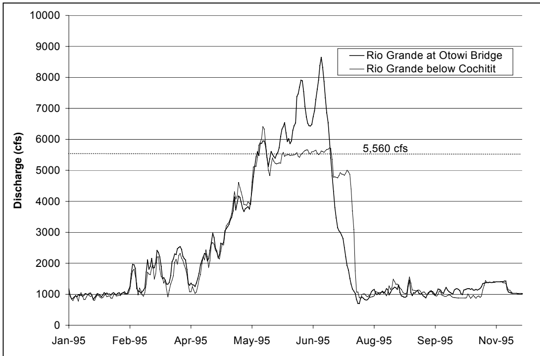
Fig. 3.5. 1995 flow hydrograph of Rio Grande at Otowi Bridge and Rio Grande below Cochiti Dam gaging stations.
