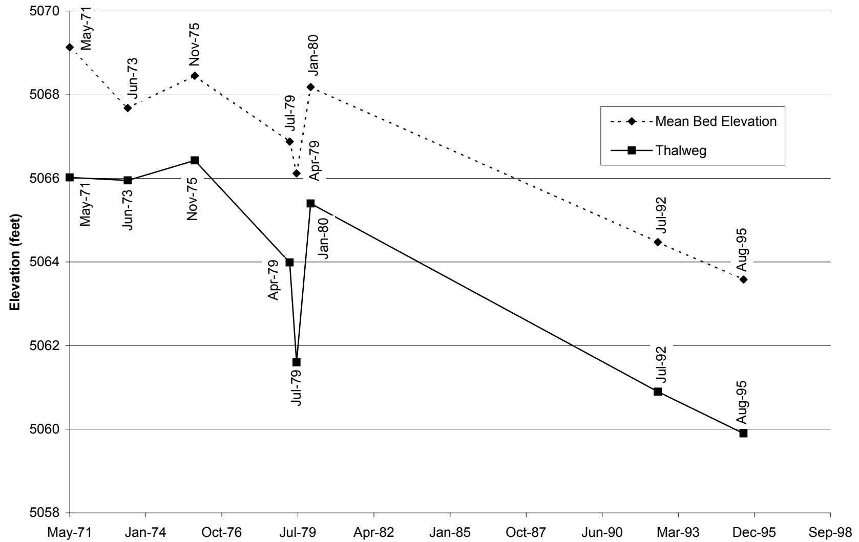
Fig. E-24. Change in thalweg elevation and mean bed elevation with time at cross section CO-26.
