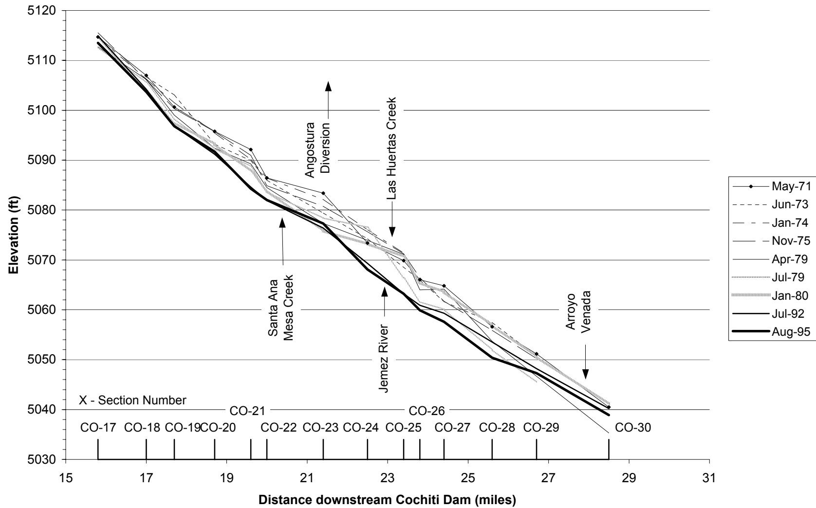
Fig. 3.11. Thalweg profile from cross section CO-17 to cross section CO-30.
