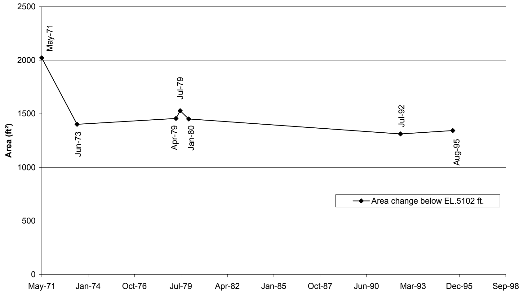
Fig. E-31. Change in cross section area with time at cross section CO-4.
