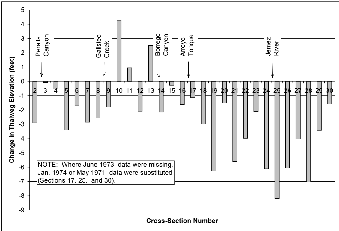
Fig. 3.12. Change in thalweg elevation between June 1973 and August 1995.
