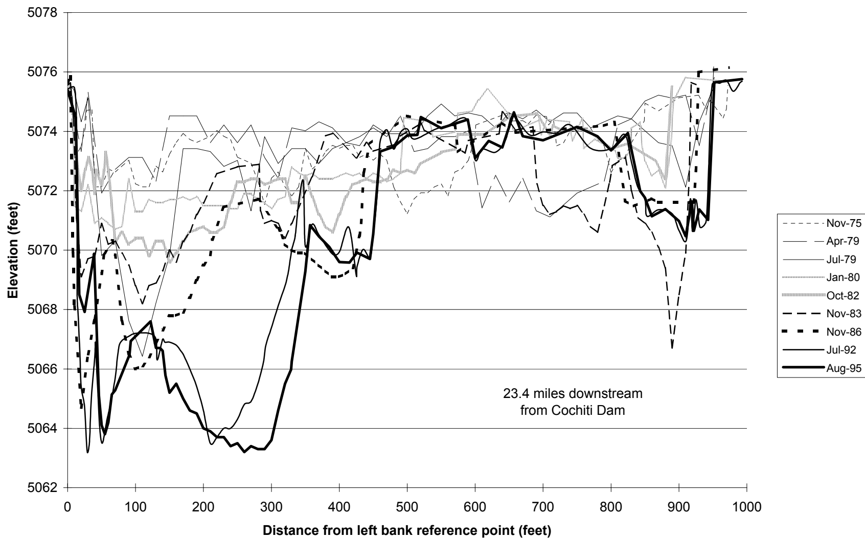
Fig.D-15. Cross Section CO-25.
