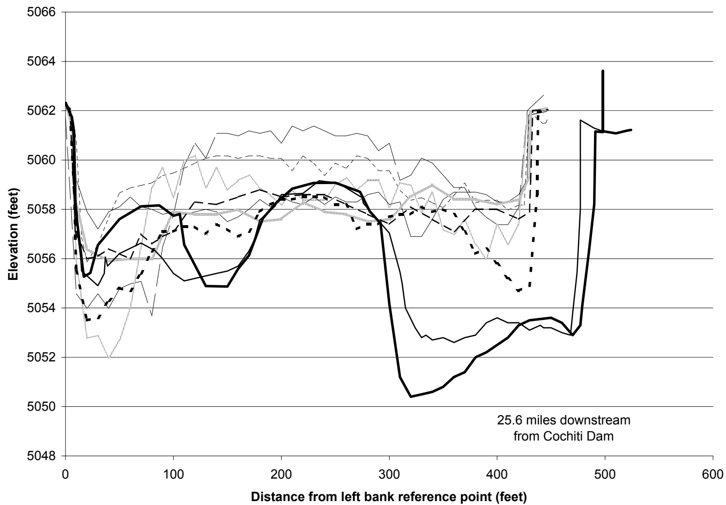
Fig.D-18. Cross Section CO-28.
