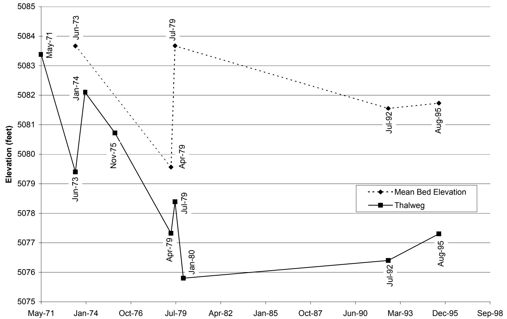
Fig. E-21. Change in thalweg elevation and mean bed elevation with time at cross section CO-23.
