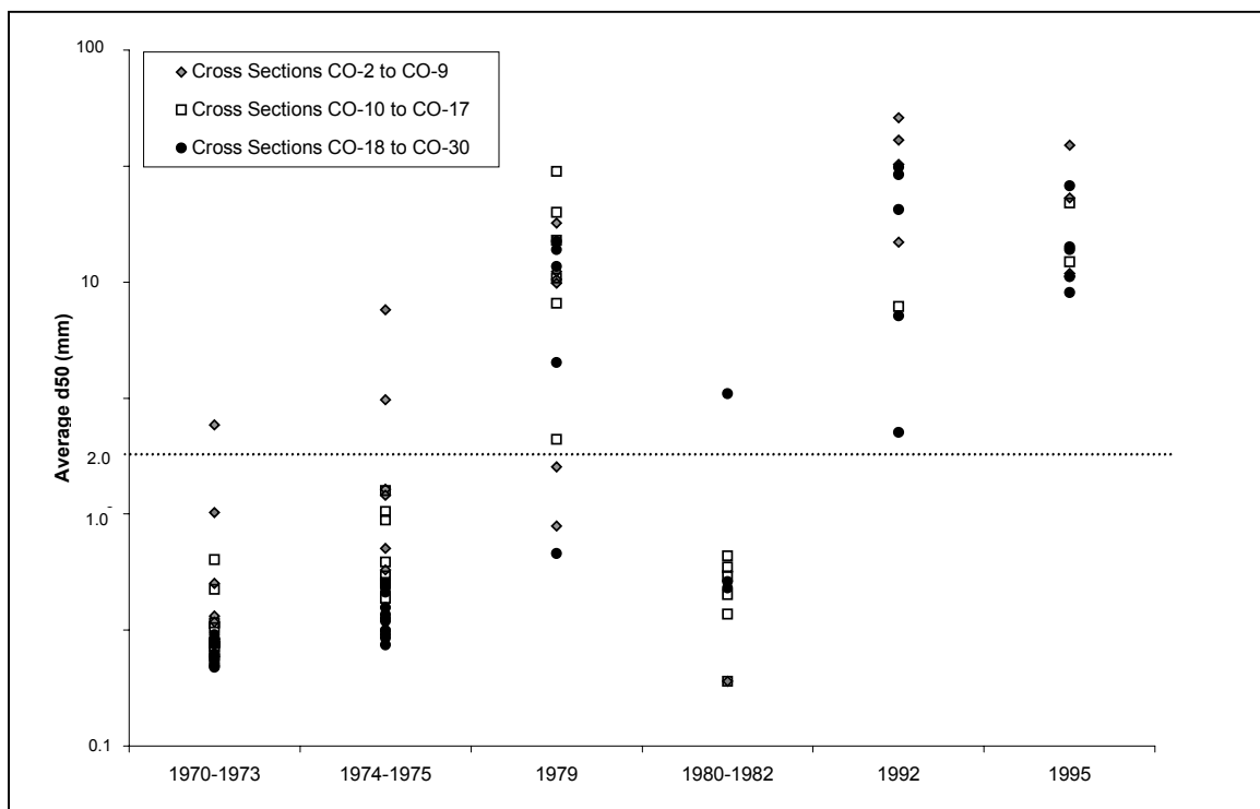
Fig. 3.17. Change in median bed material size with time.
