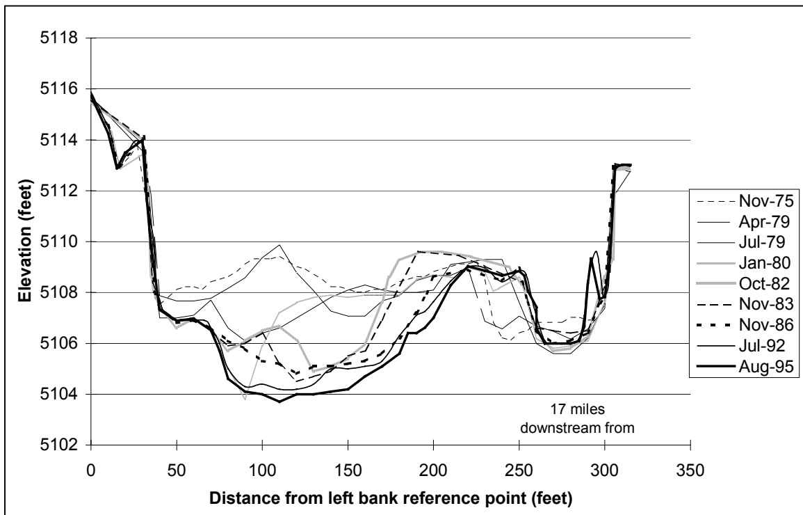
Fig. 4.8. Cross section CO-18.
