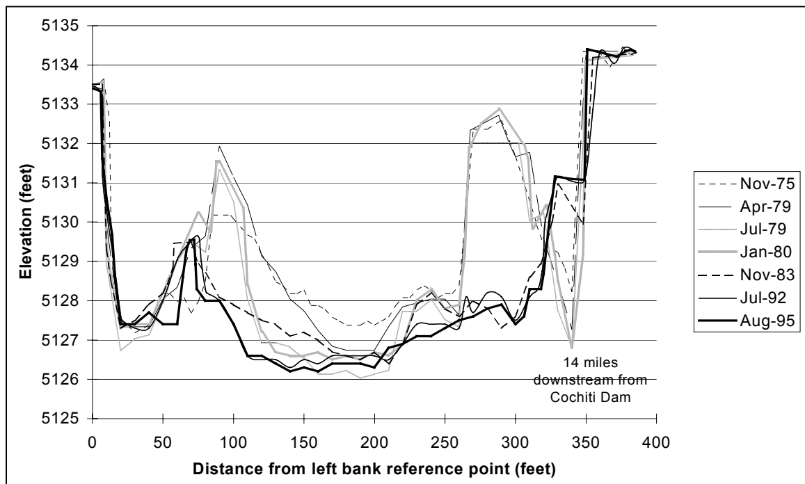
Fig. 4.6. Cross section CO-15.
