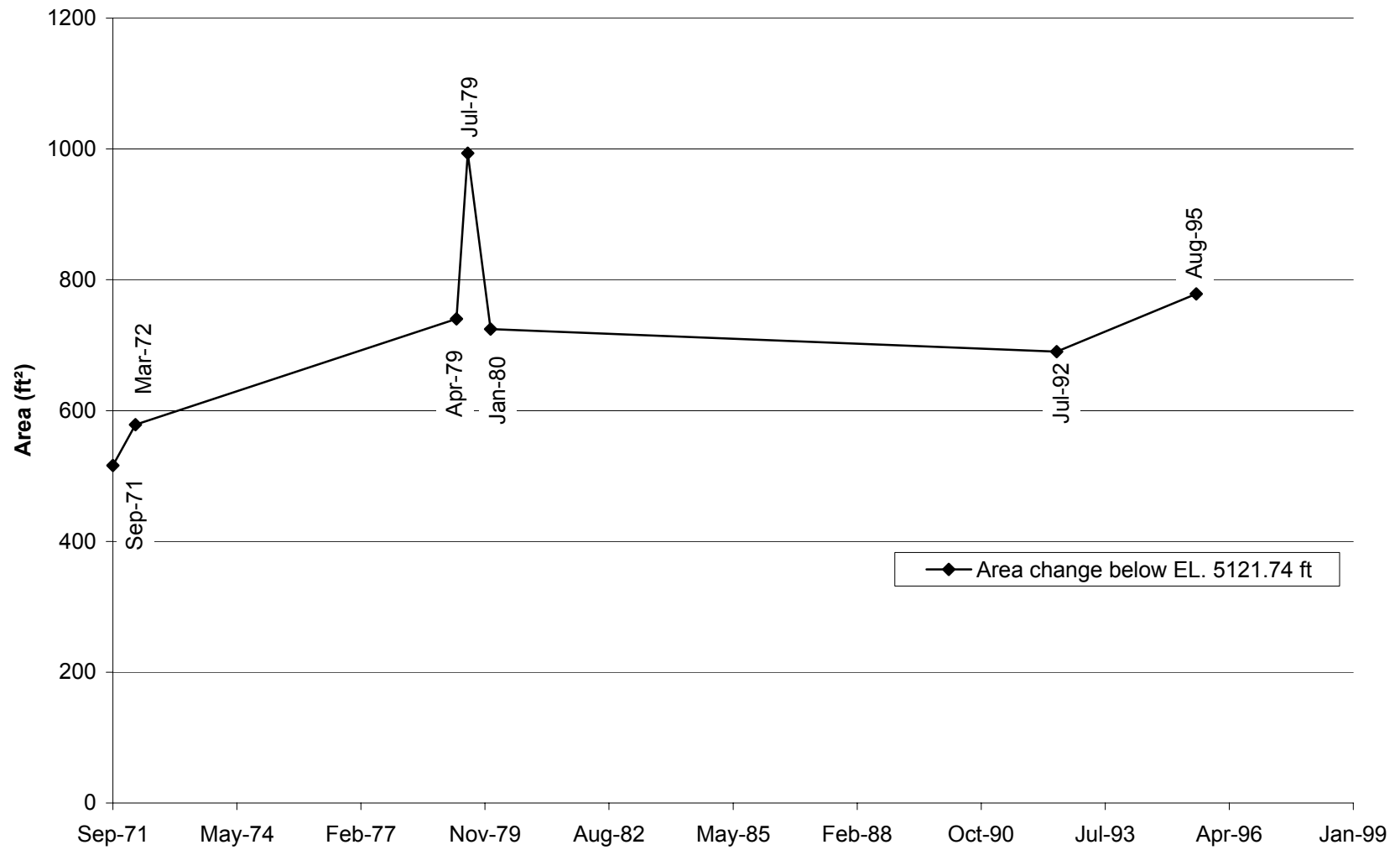
Fig. E-44. Change in cross section area with time at cross section CO-17.
