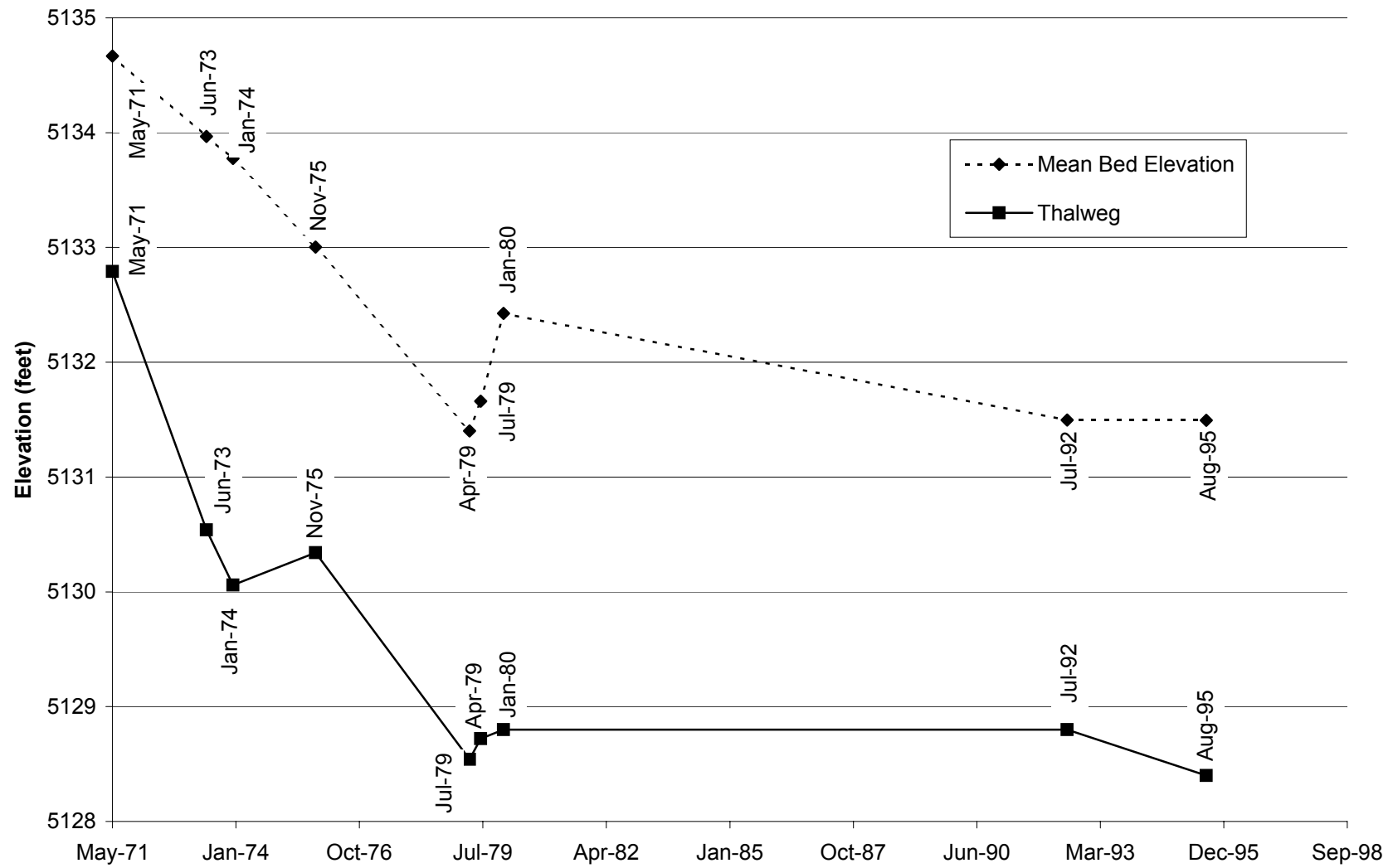
Fig. E-12. Change in thalweg elevation and mean bed elevation with time at cross section CO-14.
