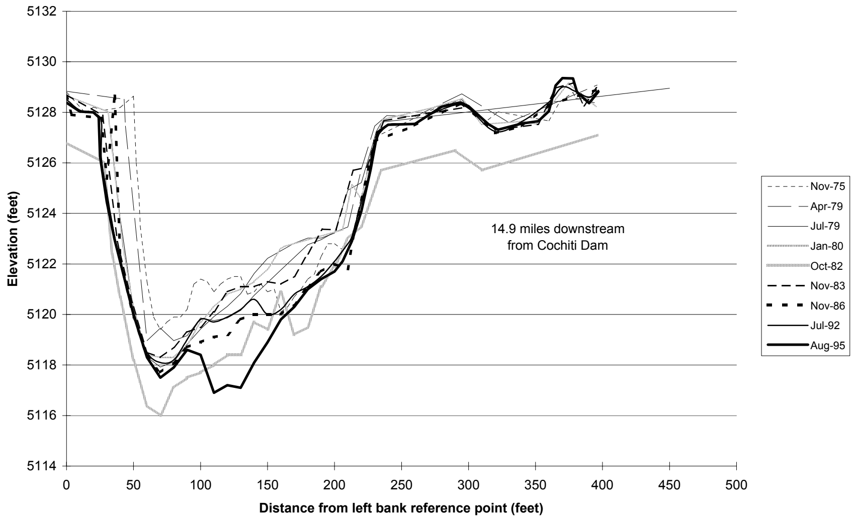
Fig.D-10. Cross Section CO-16.
