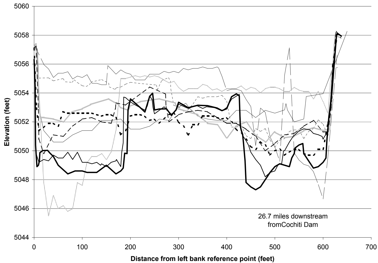
Fig.D-19. Cross Section CO-29
