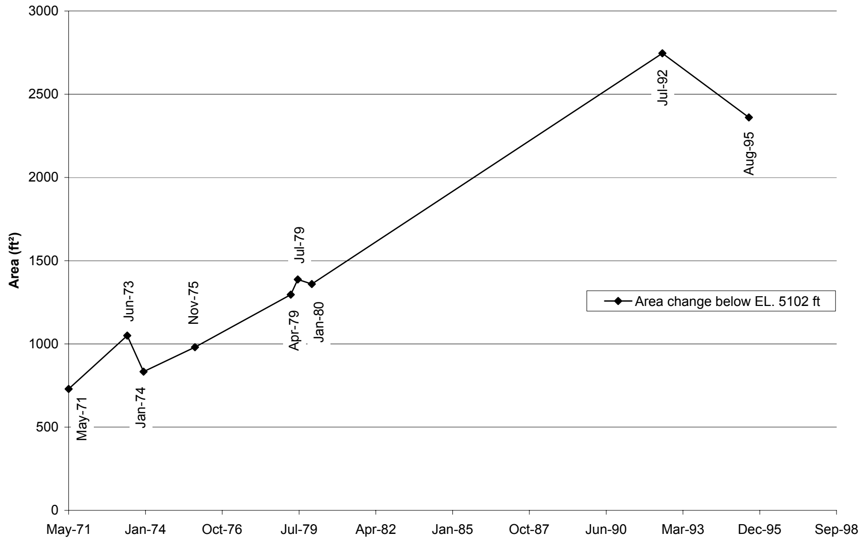
Fig. E-47. Change in cross section area with time at cross section CO-20.
