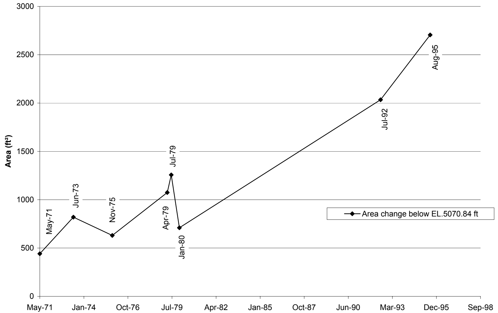
Fig. E-53. Change in cross section area with time at cross section CO-26.
