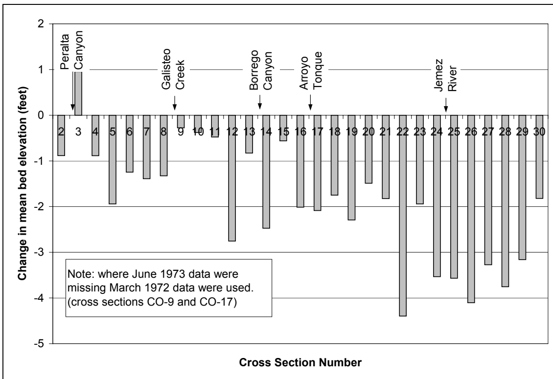
Fig. 3.13. Change in mean bed elevation between June 1973 and August 1995.
