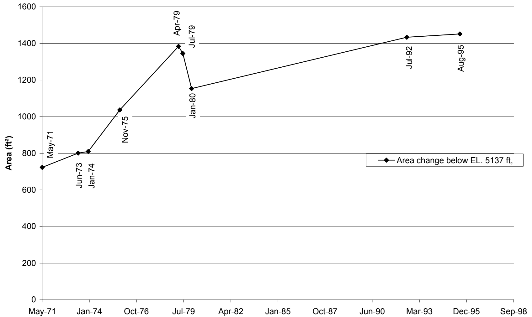
Fig. E-41. Change in cross section area with time at cross section CO-14.
