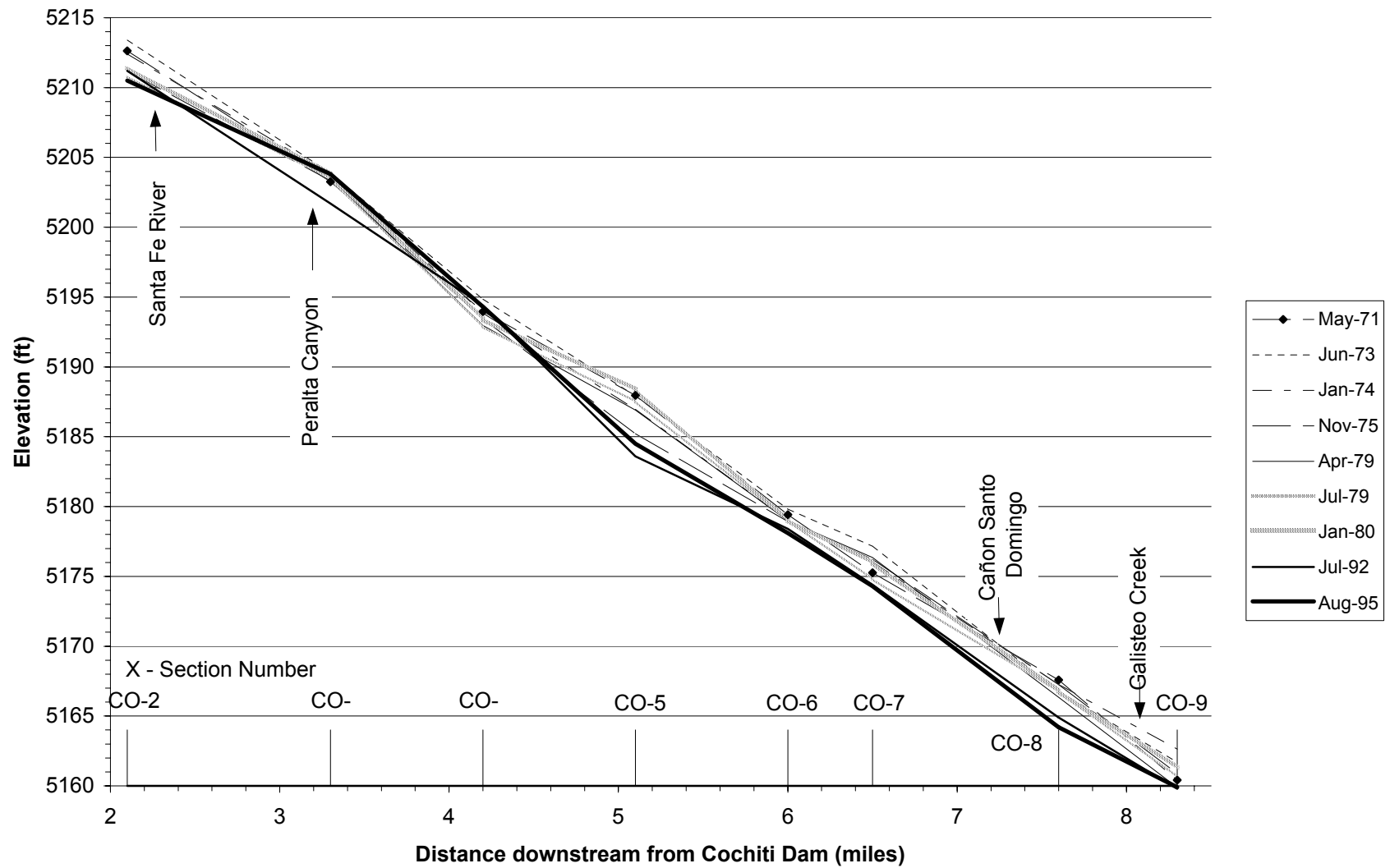
Fig. 3.9. Thalweg profile from cross section CO-2 to cross section CO-9
