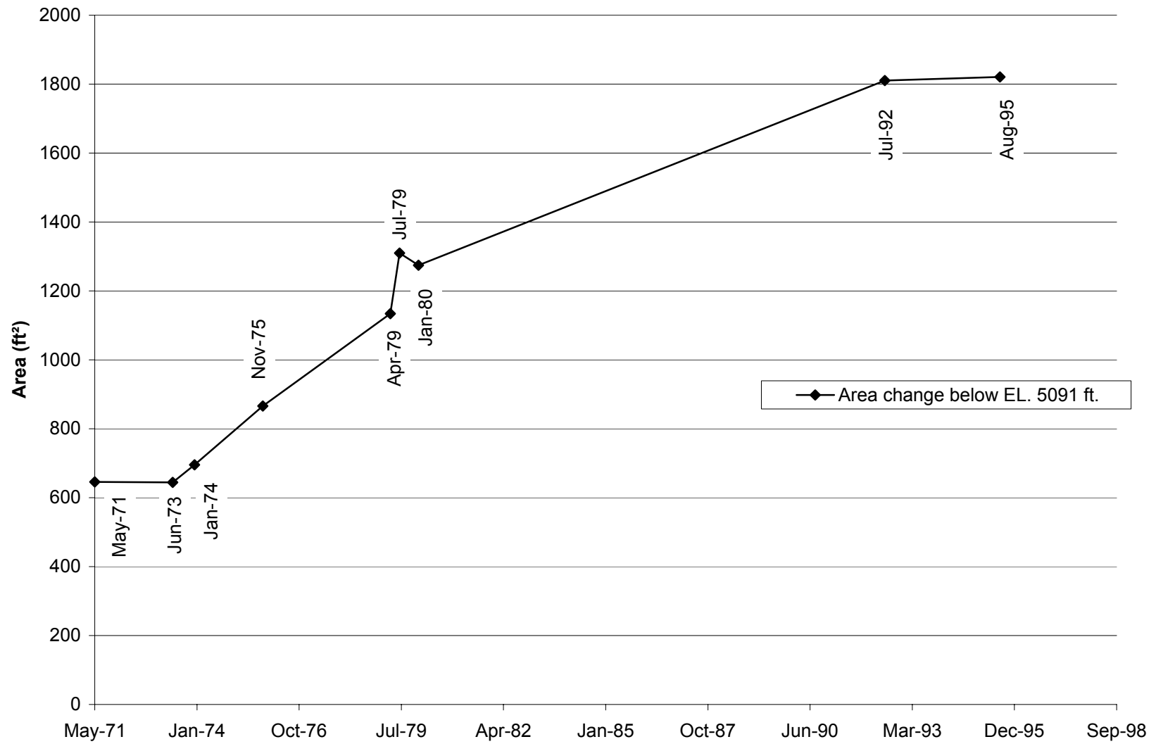
Fig. E-49. Change in cross section area with time at cross section CO-22.
