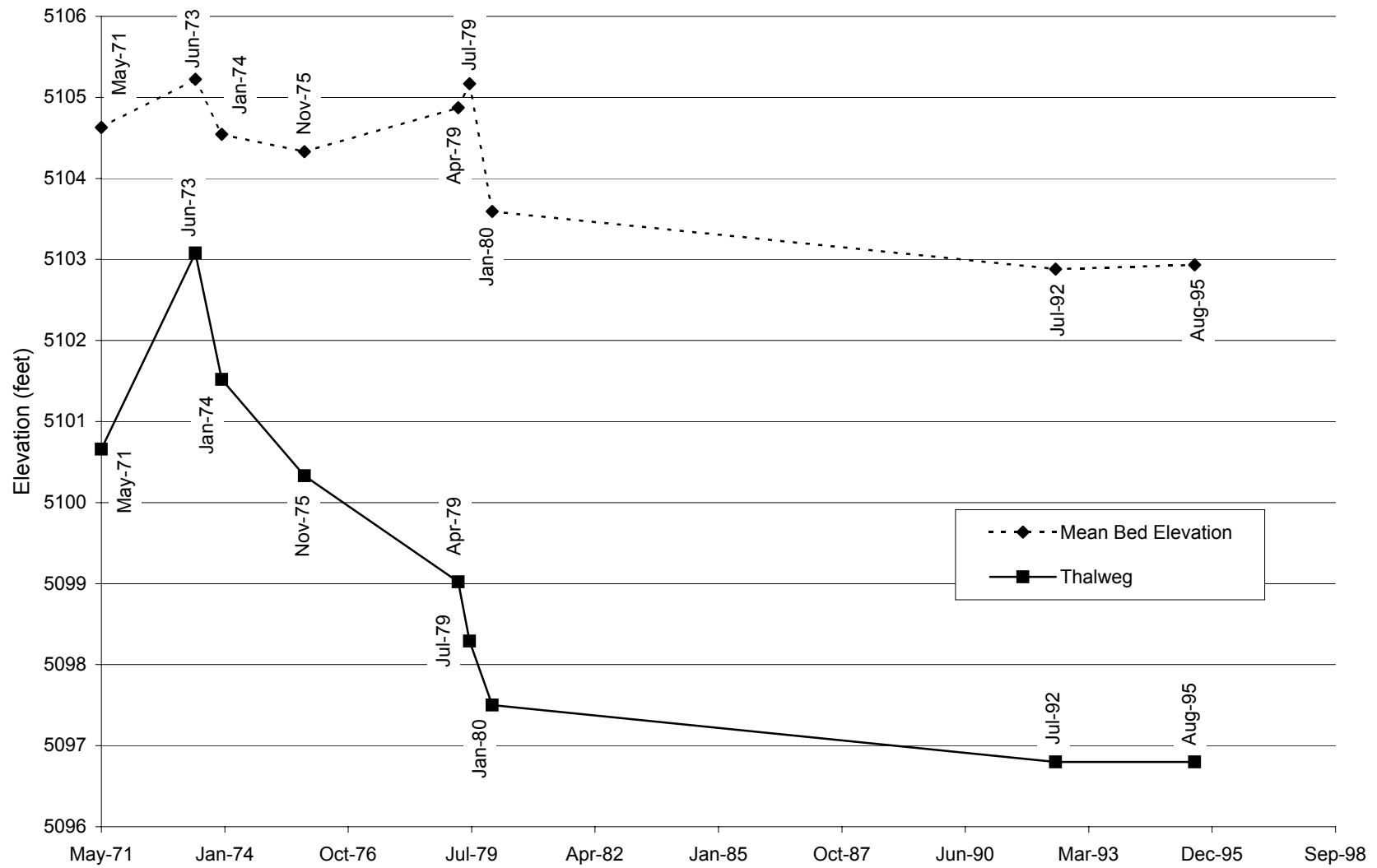
Fig. E-17. Change in thalweg elevation and mean bed elevation with time at cross section CO-19.
