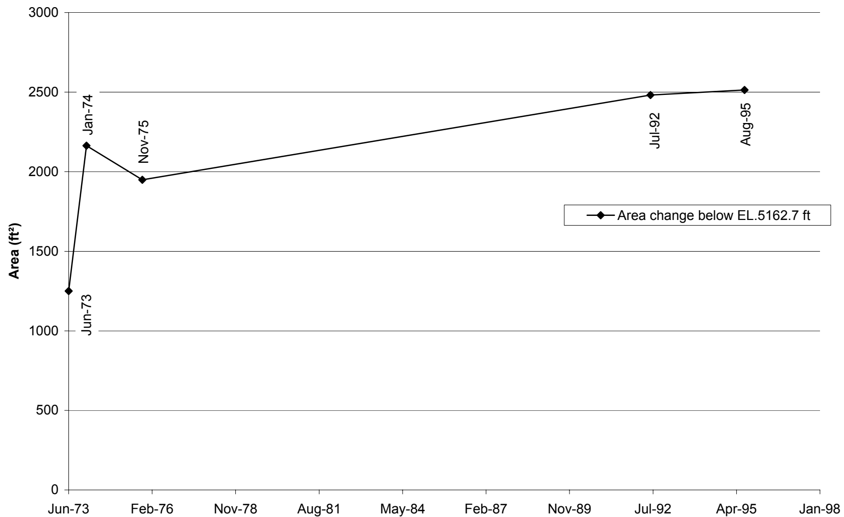
Fig. E-37. Change in cross section area with time at cross section CO-10.
