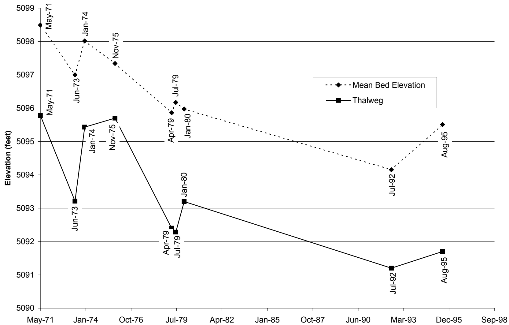
Fig. E-18. Change in thalweg elevation and mean bed elevation with time at cross section CO-20.
