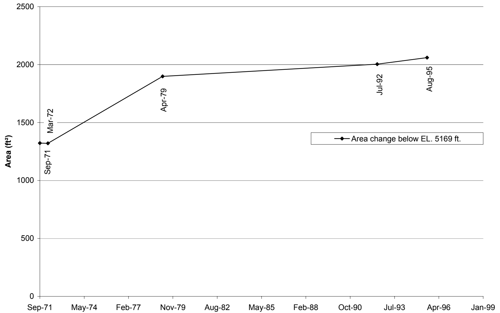
Fig. E-36. Change in cross section area with time at cross section CO-9.
