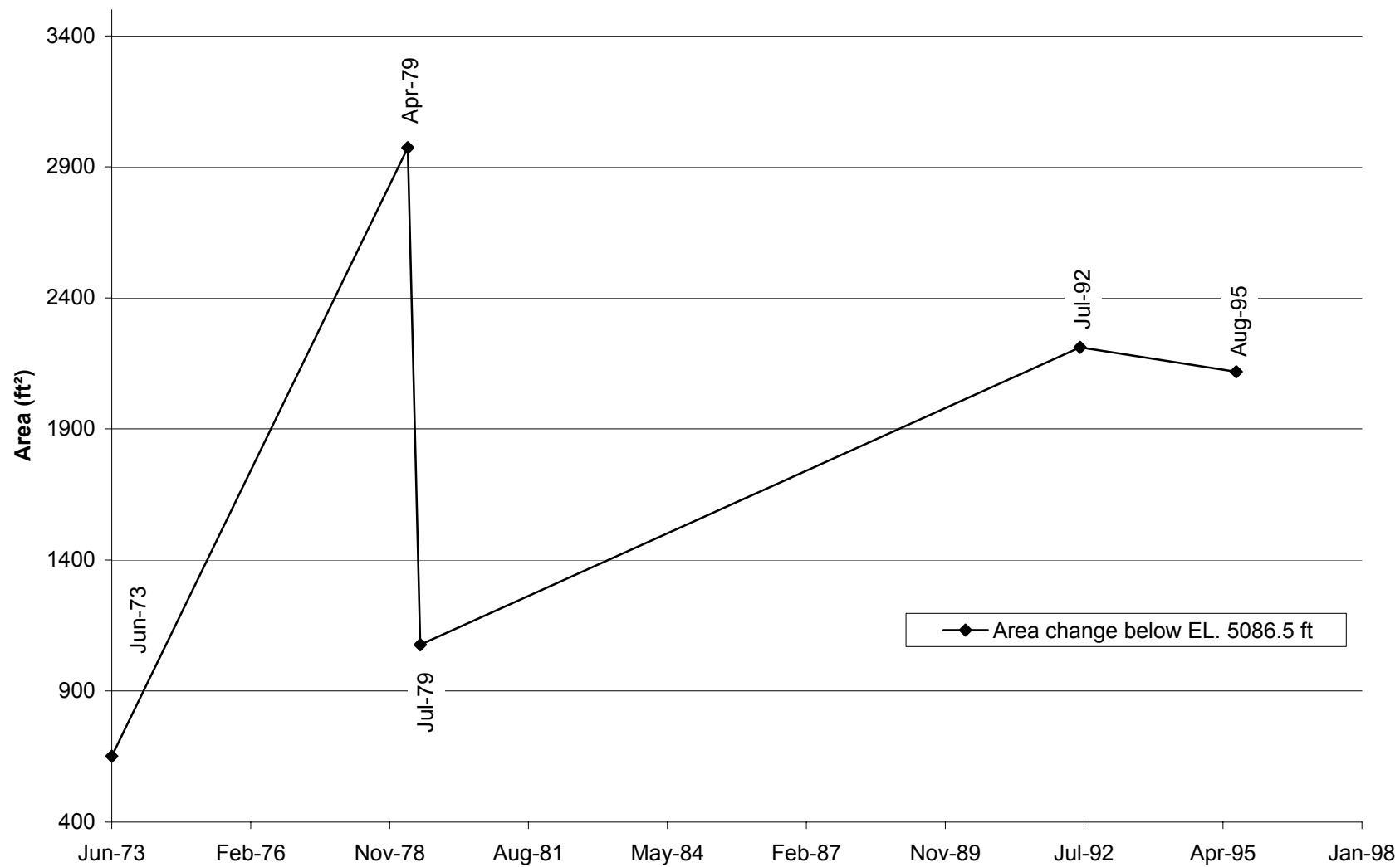
Fig. E-50. Change in cross section area with time at cross section CO-23.
