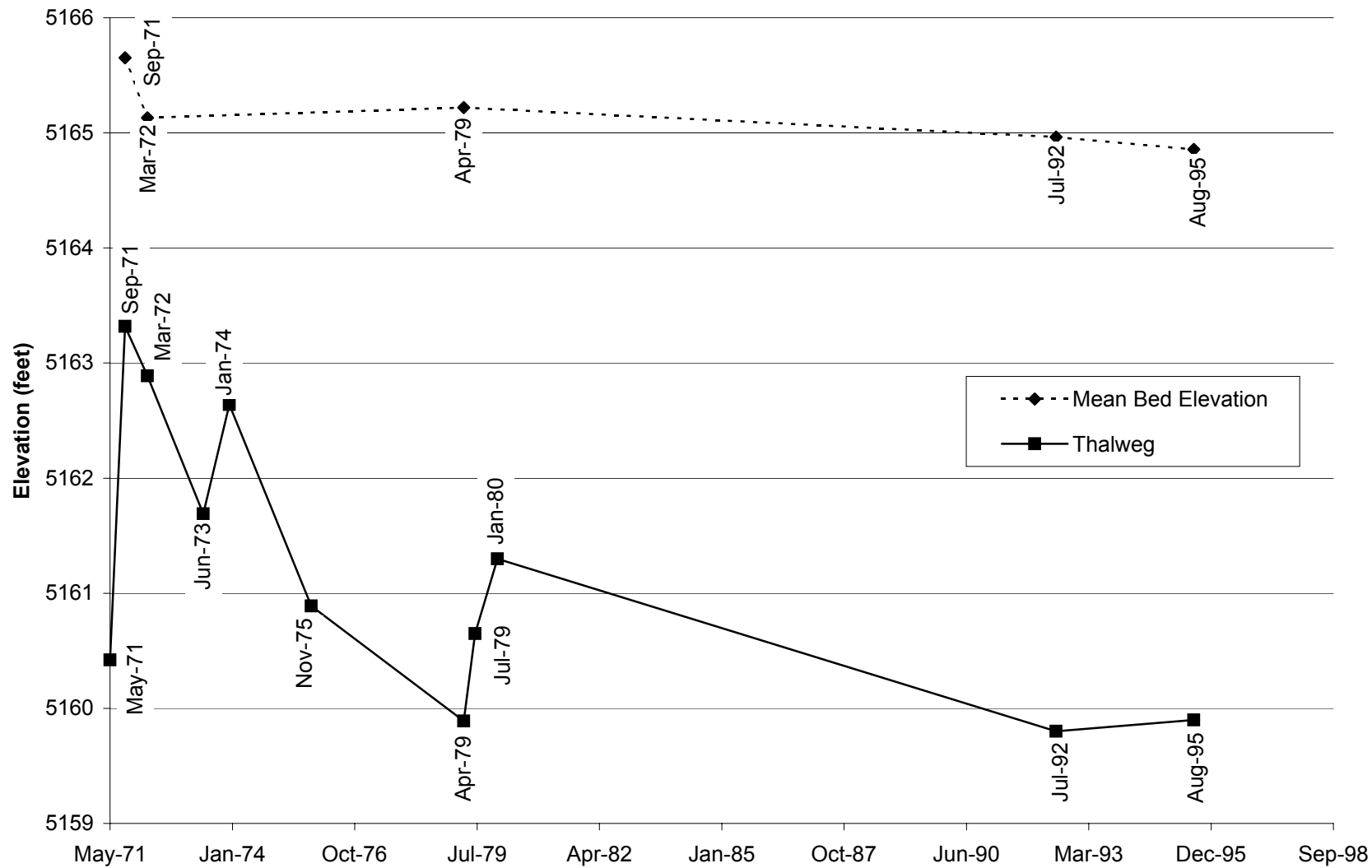
Fig. E-8. Change in thalweg elevation and mean bed elevation with time at cross section CO-9.
