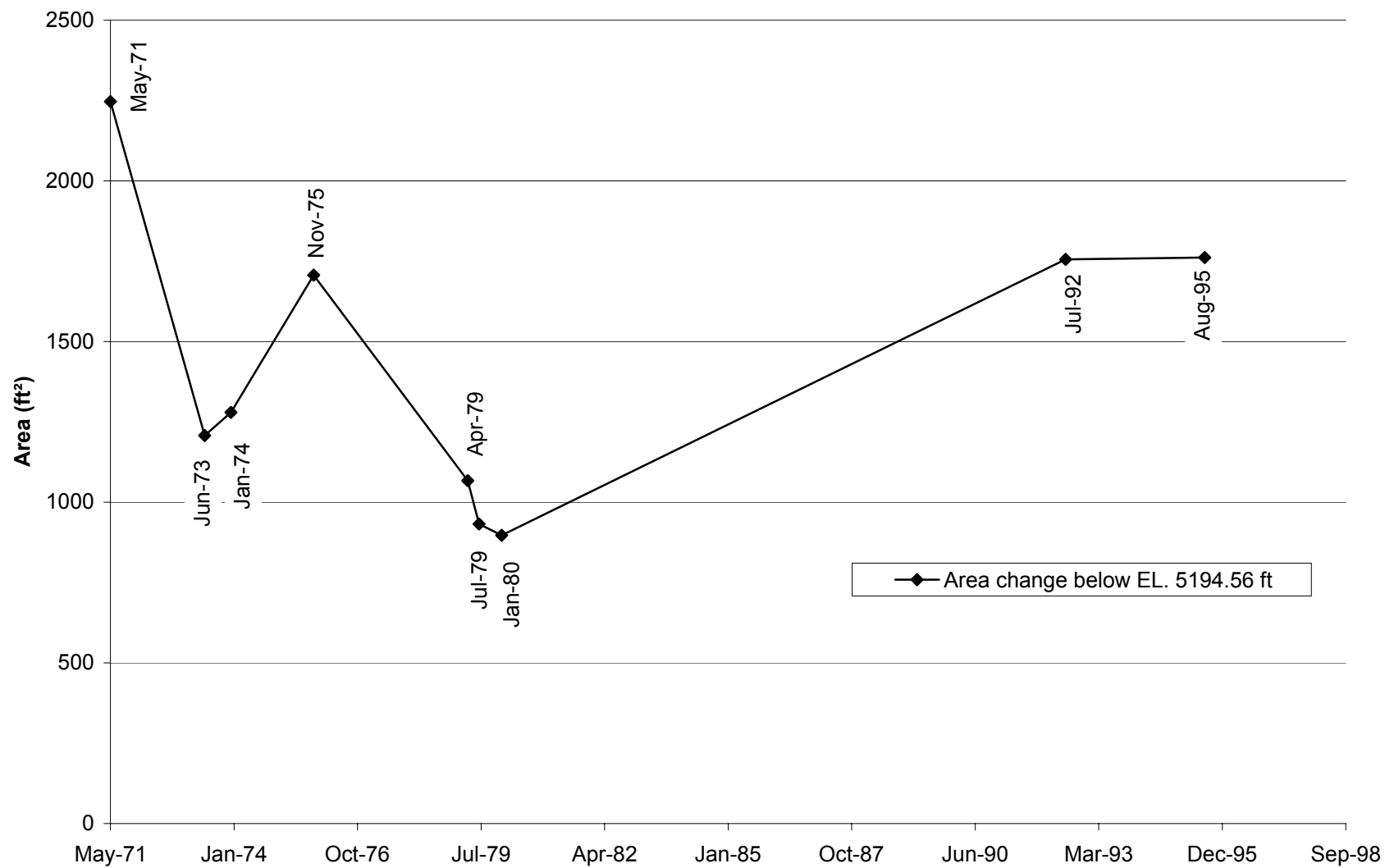
Fig. E-32. Change in cross section area with time at cross section CO-5.
