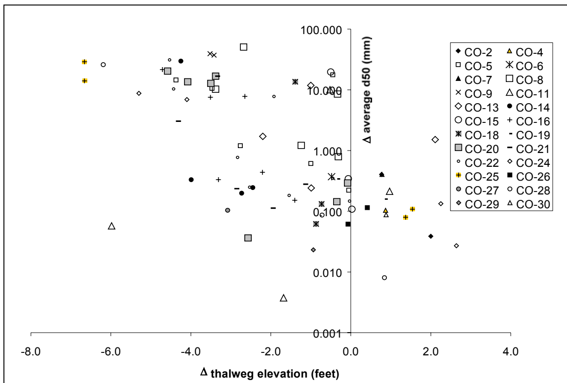
Fig. 3.18. Change in thalweg elevation versus change in median bed material size with respect to the 1971 data.
