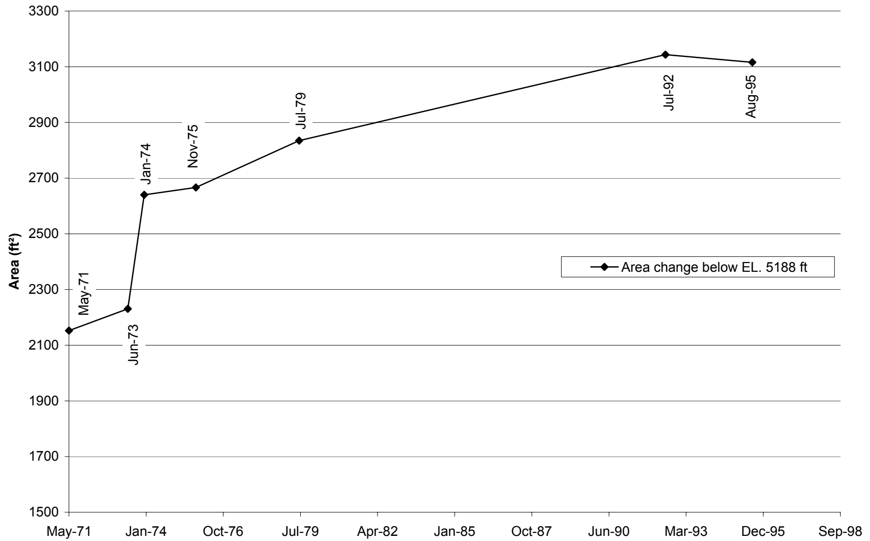
Fig. E-33. Change in cross section area with time at cross section CO-6.
