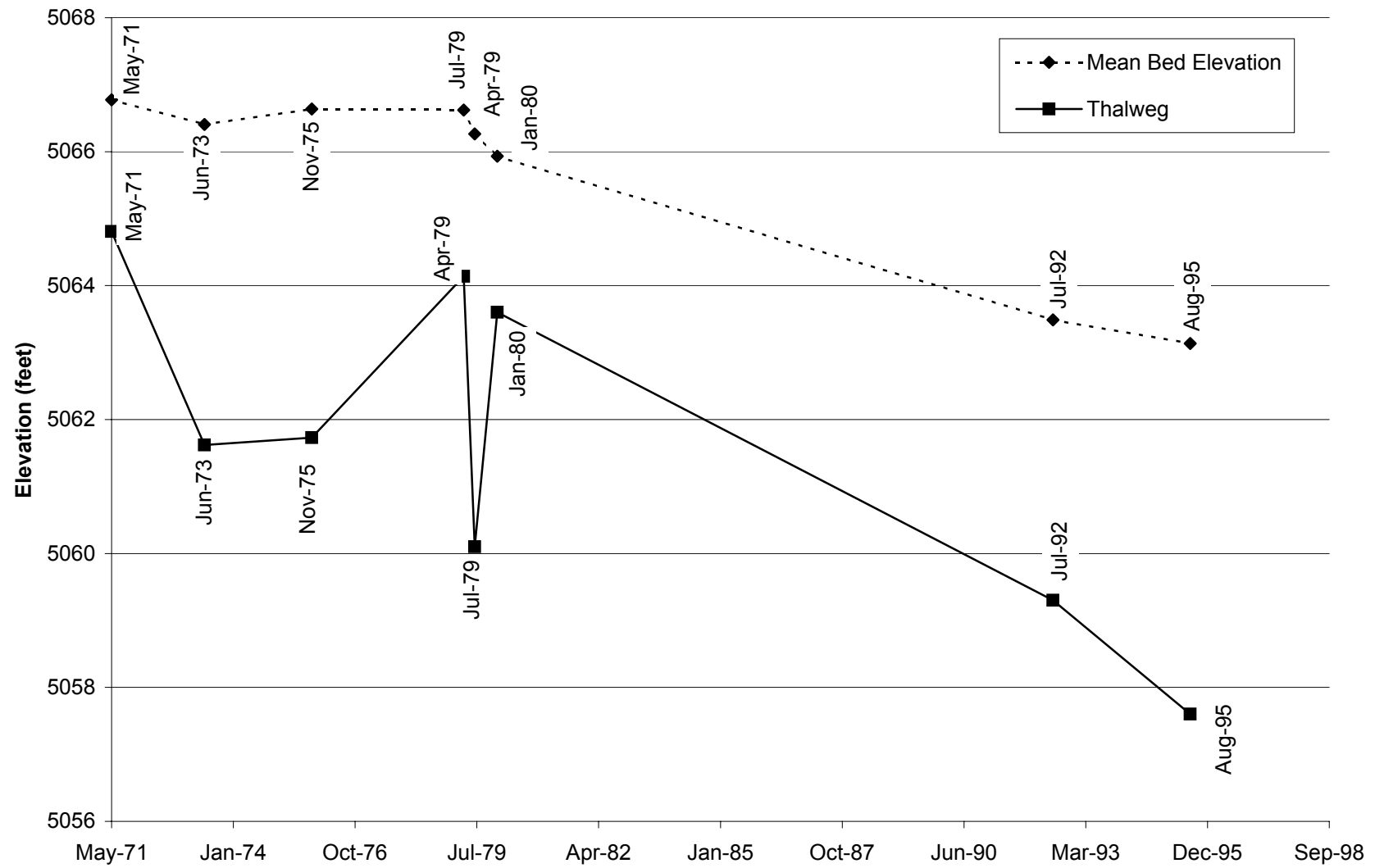
Fig. E-25. Change in thalweg elevation and mean bed elevation with time at cross section CO-27.
