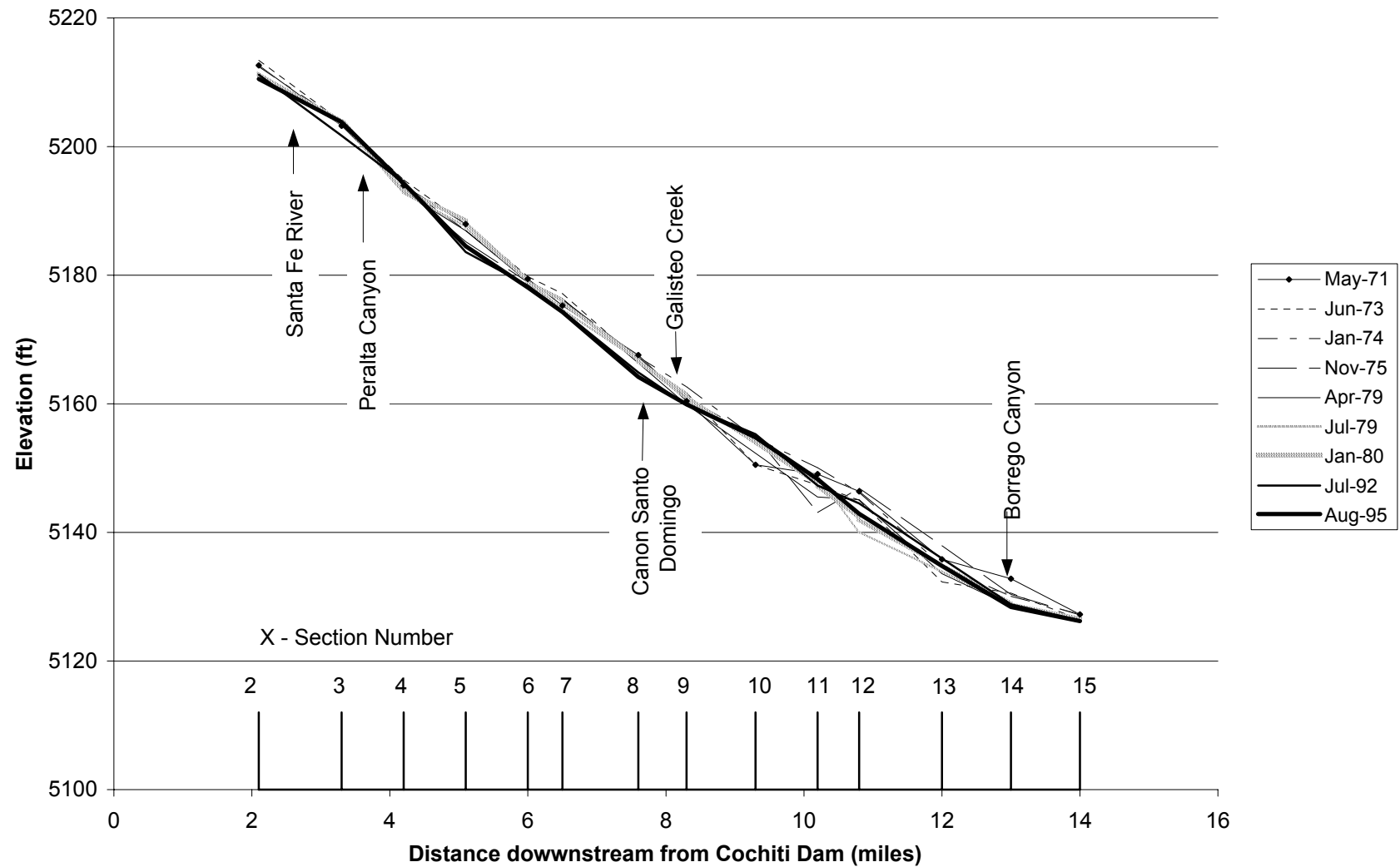
Fig. 3.7. Thalweg profile from cross section CO-2 to cross section CO-15.
