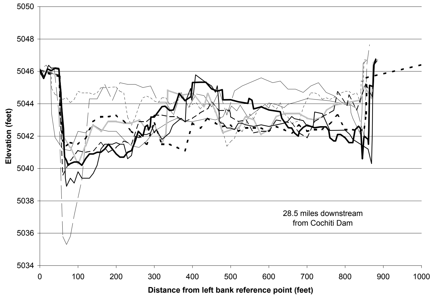
Fig.D-20. Cross Section CO-30.
