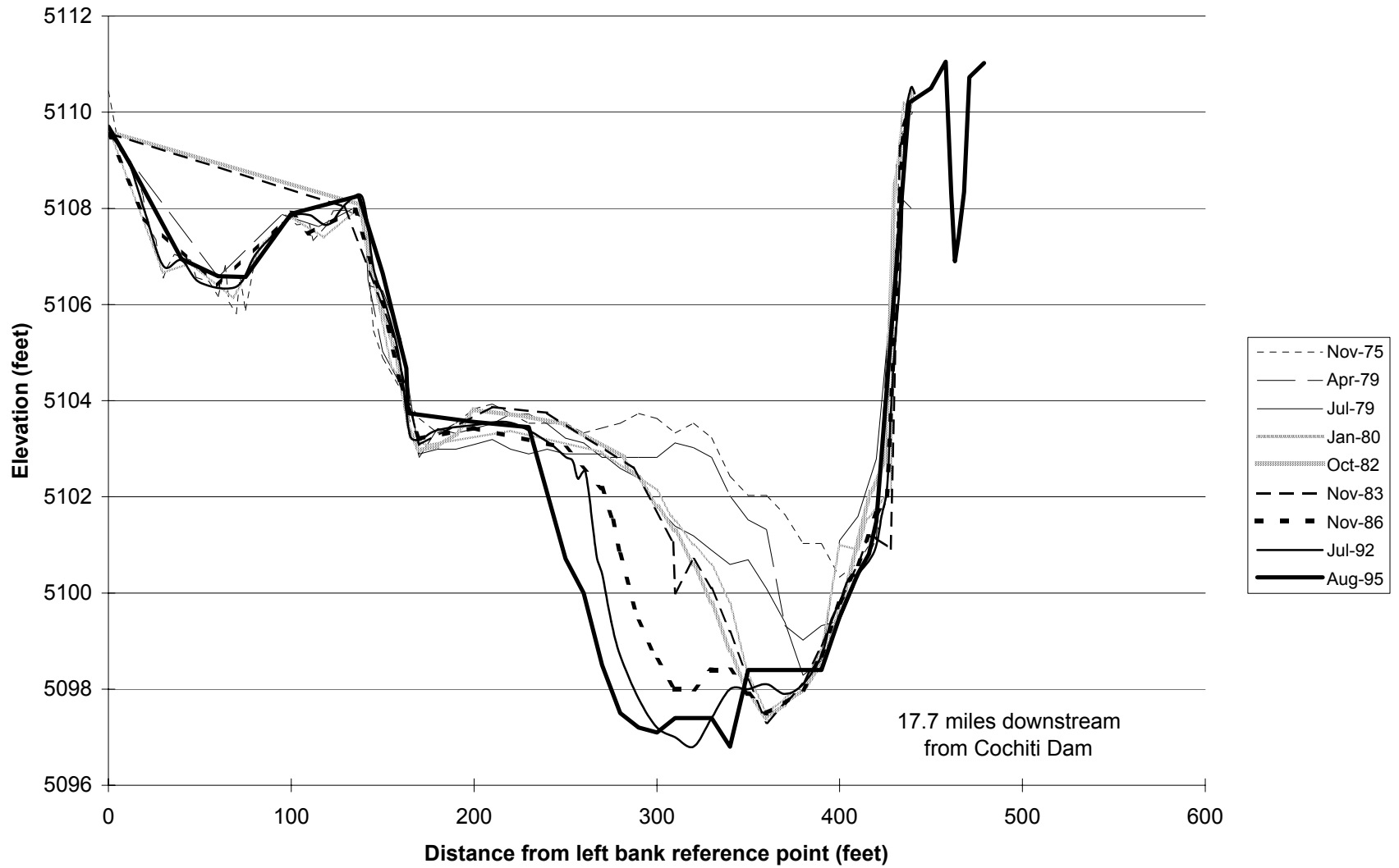
Fig.D-11. Cross Section CO-19
