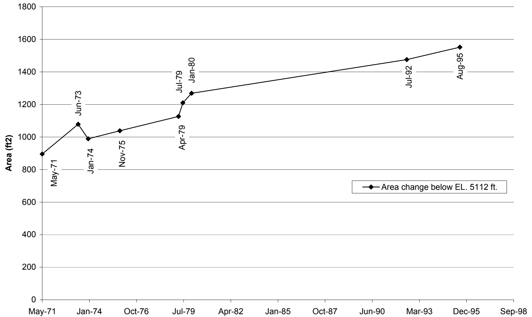
Fig. E-45. Change in cross section area with time at cross section CO-18.
