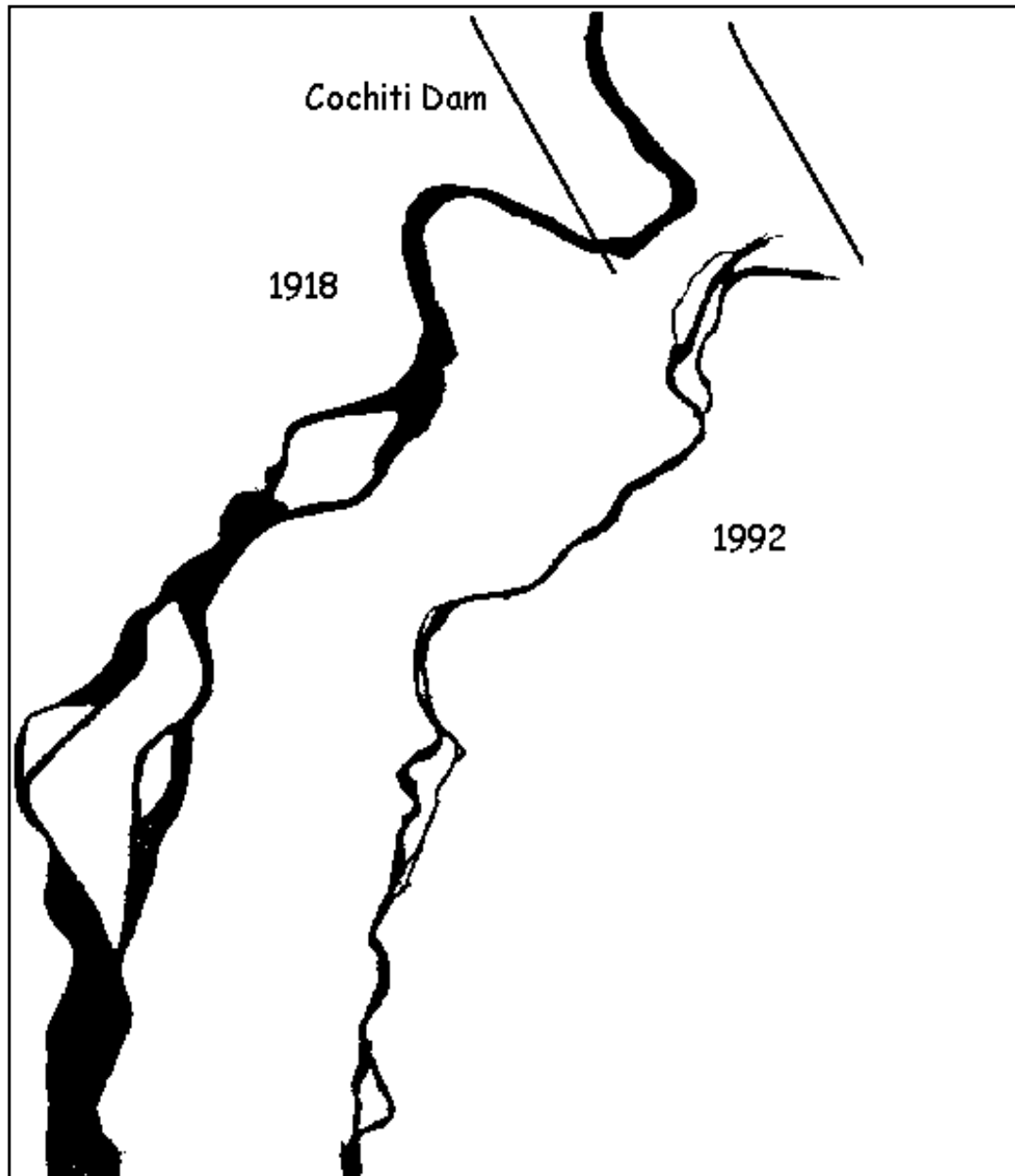
Fig. 2.2. Planform comparison below Cochiti Dam from 1918 to 1992.
