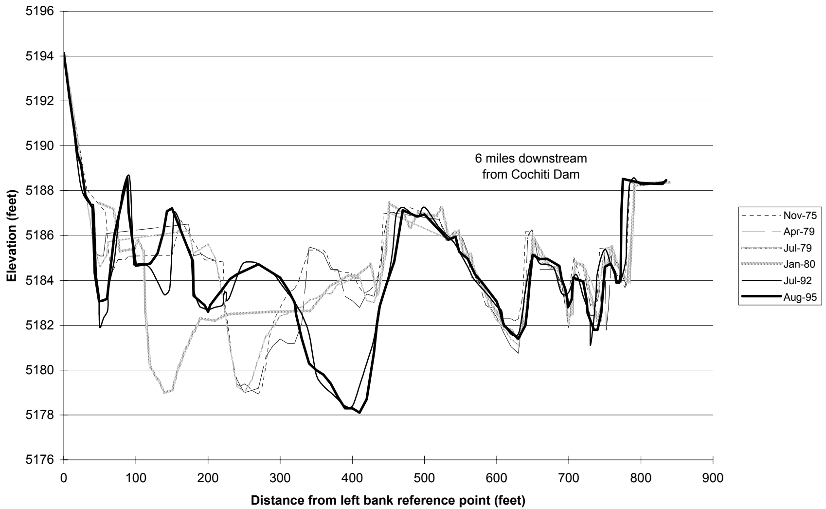
Fig.D-3. Cross Section CO-6.
