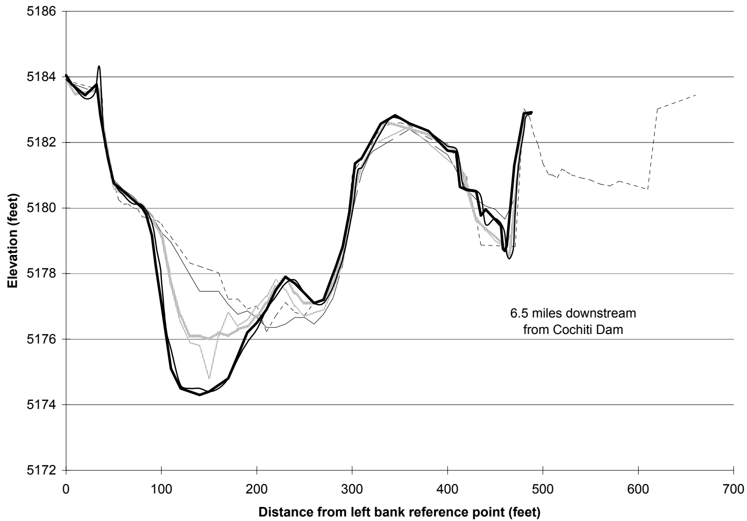
Fig.D-4. Cross Section CO-7.
