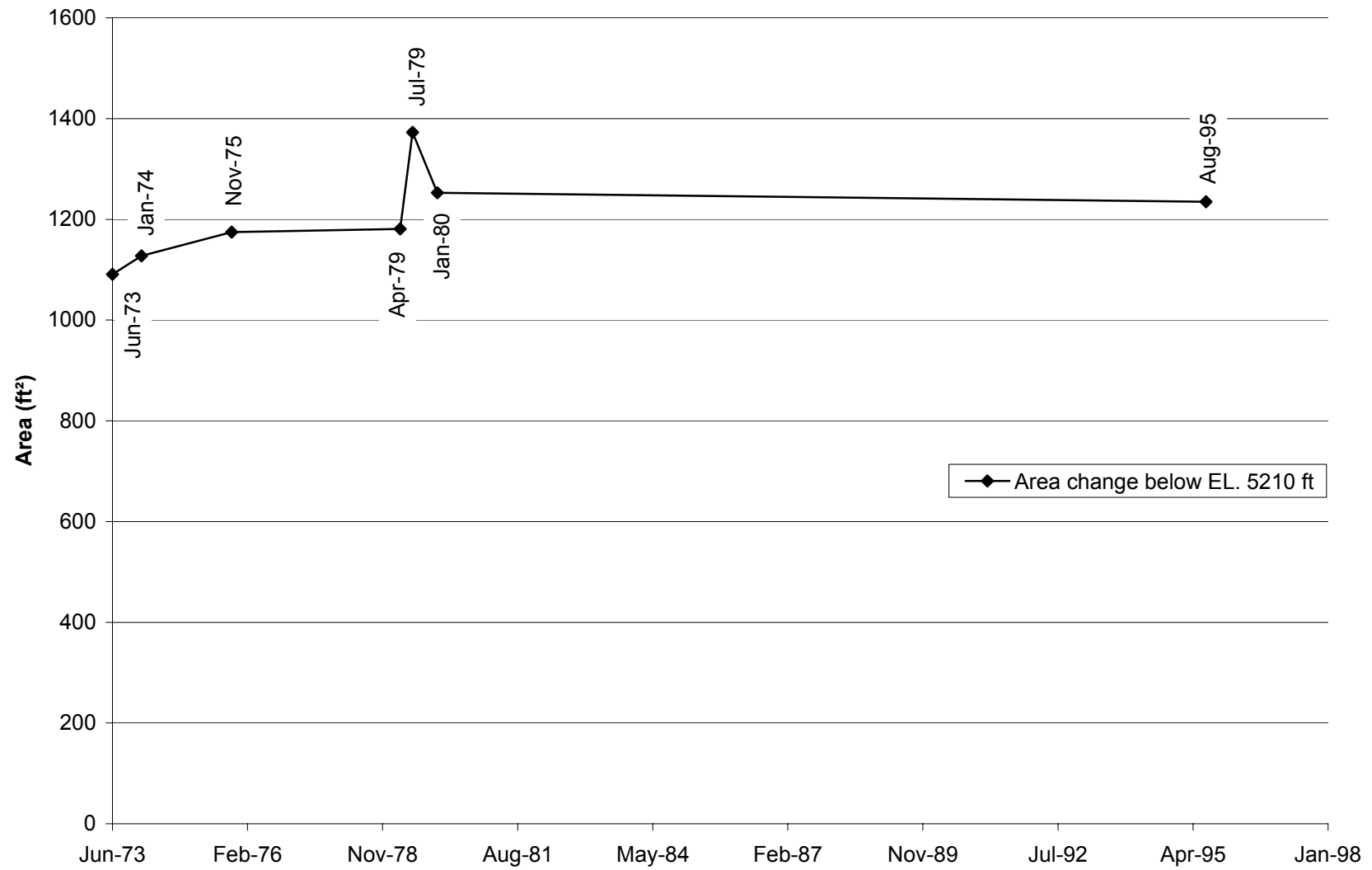
Fig. E-30. Change in cross section area with time at cross section CO-3.
