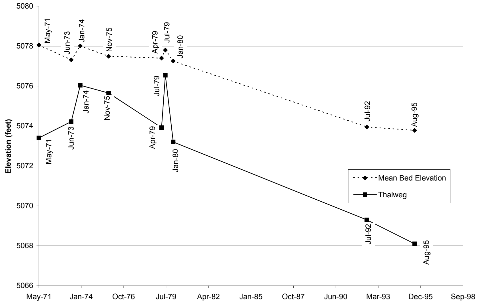
Fig. E-22. Change in thalweg elevation and mean bed elevation with time at cross section CO-24.
