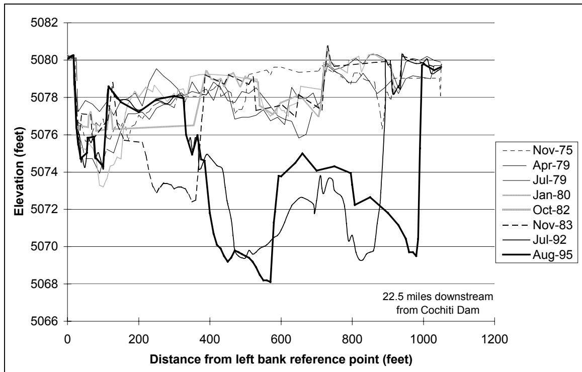
Fig. 4.10. Cross section CO-24.
