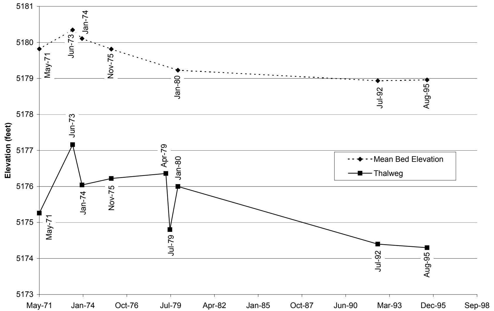
Fig. E-6. Change in thalweg elevation and mean bed elevation with time at cross section CO-7.
