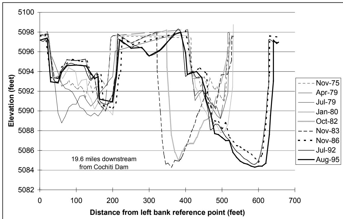
Fig. 4.9. Cross section CO-21.
