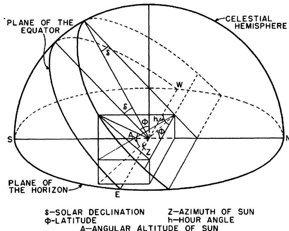
FIGURE 3.—Diagram of celestial hemisphere.
