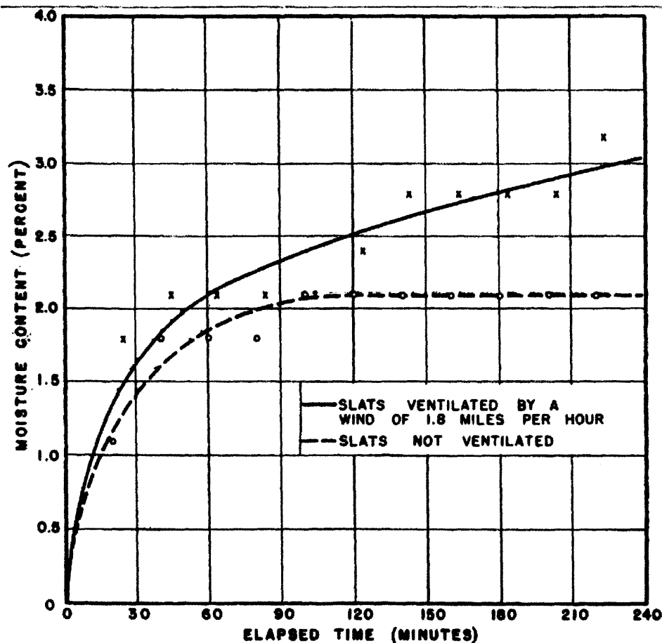
FIGURE 10.—Curves showing effect of wind on rate of gain of moisture by wood slats initially oven-dry and exposed to a radiation of 1.76 calories per square centimeter per minute. Relative humidity during test, 62 percent; air temperature, 82° F
