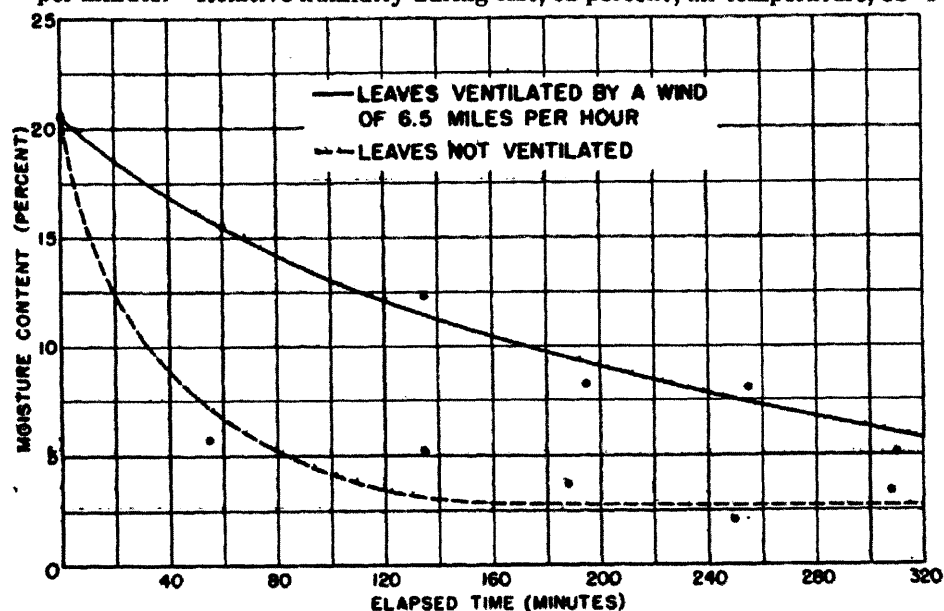
FIGURE 11.—Curves showing effect of wind on equilibrium moisture content of hardwood leaf litter exposed to a radiation of 1.76 calories per square centimeter per minute. Relative humidity during test, 51 percent; air temperature, 84° F.
