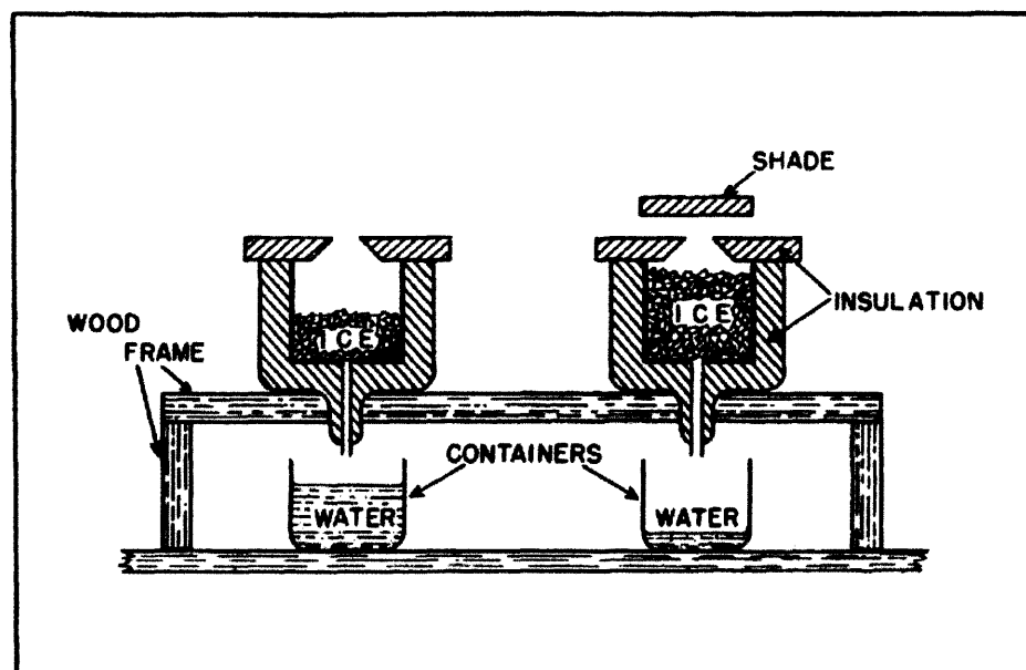
FIGURE 2.—Ice calorimeters used to measure intensity of radiation.
