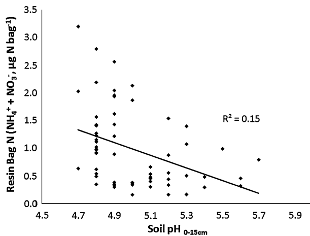
Figure 4. Total resin-sorbed N ( \text{NH}_4^+ + \text{NO}_3^- ) versus soil pH (0–15 cm) among all stands.
