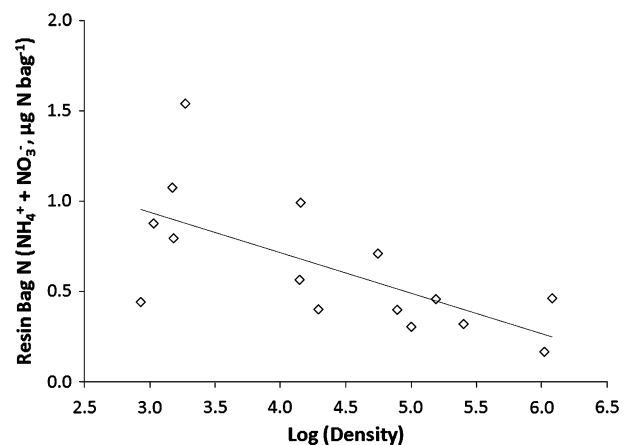
Figure 3. Total resin-sorbed N ( \text{NH}_4^+ + \text{NO}_3^- ) versus stem density among young stands younger than 20 years.
