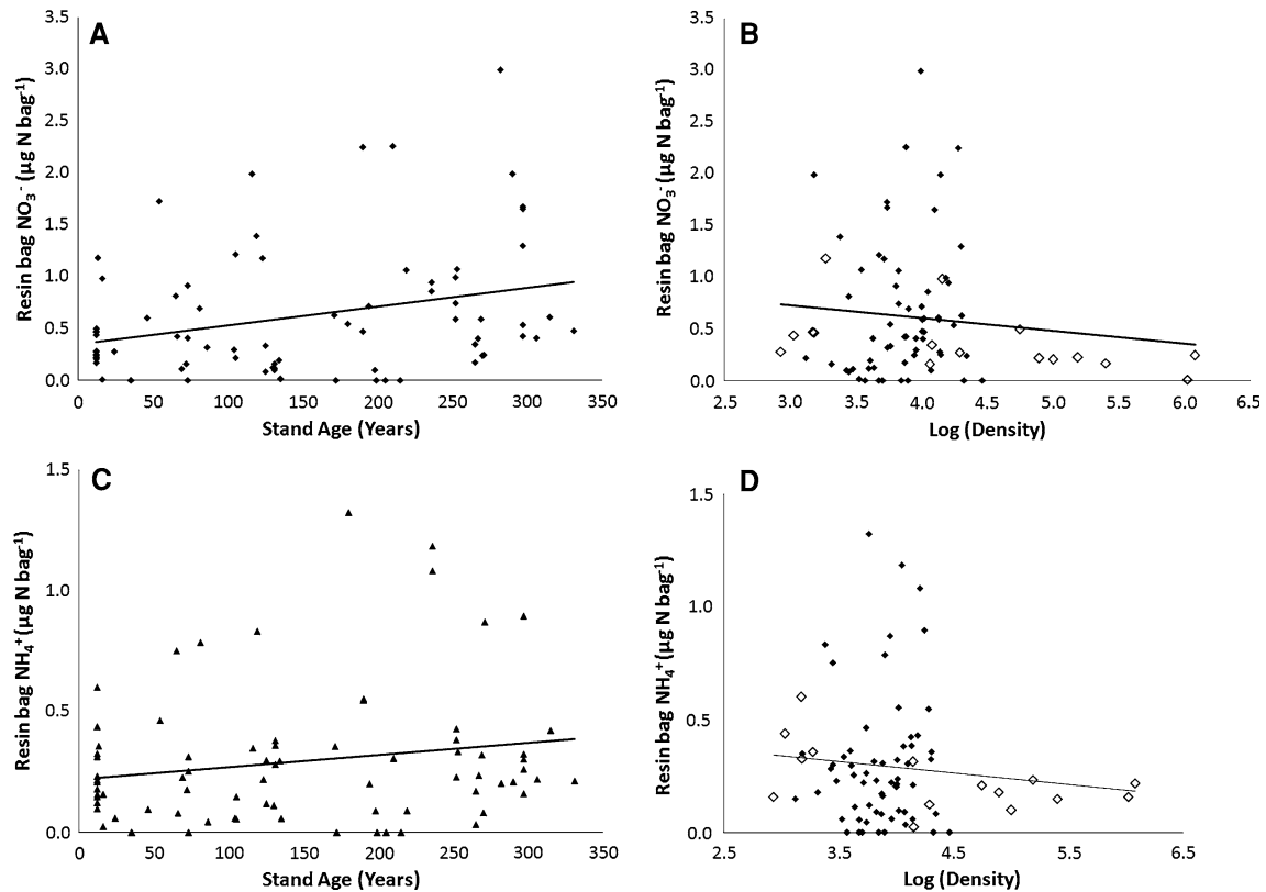
Figure 2. Relationship between resin-sorbed nitrogen and stand age and stem density in the Greater Yellowstone Eco-system: A resin-sorbed nitrate ( \text{NO}_3^- ) versus stand age, B resin-sorbed \text{NO}_3^- versus stem density, C resin-sorbed ammonium ( \text{NH}_4^+ ) versus stand age, D resin-sorbed \text{NH}_4^+ versus stem density. For density figures, trendline represents best fit across all stands; closed symbols = stands older than 20 years; open symbols = stands younger than 20 years.
