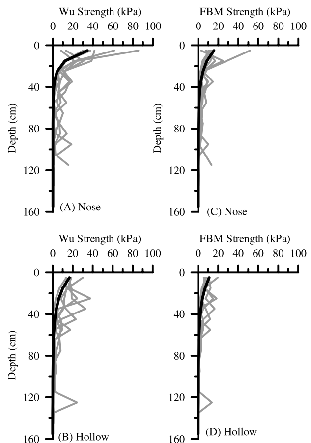
Figure 6. Distribution of root cohesive strength as a function of depth for (a and c) nose and (b and d) hollow locations using the Wu method (Figures 6a and 6b) [Wu et al. , 1979] and fiber bundle model method (Figures 6c and 6d) [Pollen and Simon, 2005]. Individual gray lines correspond to pits, while the dark line corresponds to the modeled mean across pits (equation (5c)).
