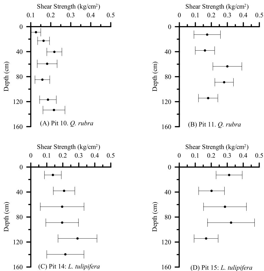
Figure 2. Depth distribution of shear strength measured using a vane shear in Q. rubra and L. tulipifera pits in both (a and c) hollow and (b and d) nose locations. Points represent the mean of five measurements and the bars are standard deviations.
