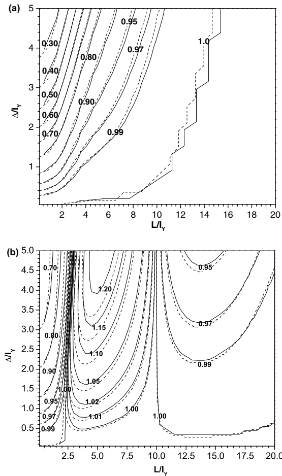
Fig. 10. Contour plots of R_C at \mathbf{x} = (10I_Y, 0) for (a) t = 10I_Y/U and (b) t = 15I_Y/U . First-order solutions obtained with Pe_T = 1000 , and R_{Pe} = 10 (solid lines) are compared with those obtained in the absence of PSD ( Pe \rightarrow \infty , dashed lines). In all cases \sigma_Y^2 = 0.2 .
