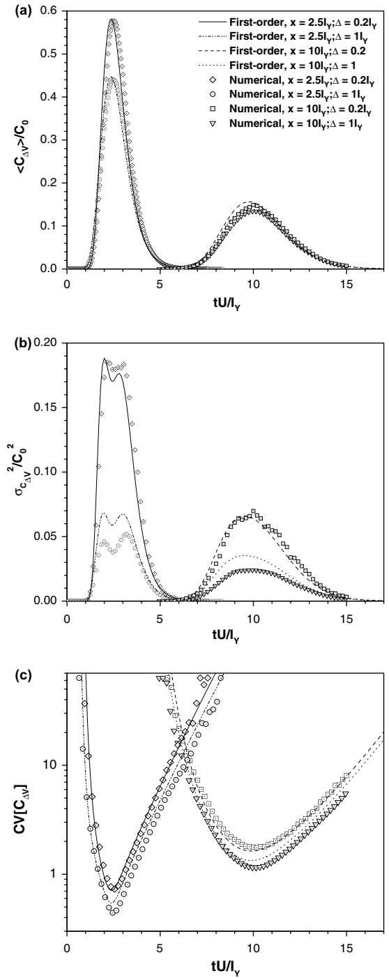
Fig. 4. First-order solutions of (a) \langle C_{\Delta V} \rangle (Eq. (A.1)), (b) \sigma_{C_{\Delta V}}^2 (Eq. (9)), and (c) CV(C_{\Delta V}) (Eq. (8)) are compared with numerical simulations (symbols) at \mathbf{x} = (2.5I_Y, 0) and \mathbf{x} = (10I_Y, 0) for several sampling volumes. In all cases, the source area is a square with side L = 1I_Y , \sigma_Y^2 = 0.2 , Pe_T = 1000 , and R_{Pe} = 1 .
