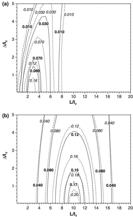
Fig. 8. Contour plot of \sigma^2_{C_{\Delta V}} as a function of source and sampling volumes at \mathbf{x} = (10I_Y, 0) for (a) t = 10 I_Y/U and (b) t = 15 I_Y/U , with \sigma_Y^2 = 0.2 . First-order solutions obtained with Pe_T = 1000 , and R_{Pe} = 10 (solid lines) are compared with those obtained in the absence of PSD ( Pe \rightarrow \infty , dashed lines).
