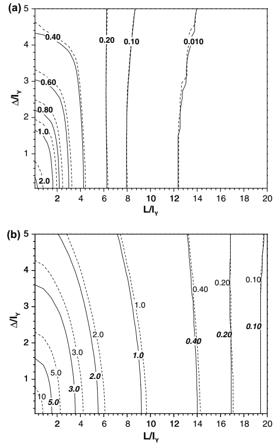
Fig. 9. Contour plots of CV(C_{\Delta V}) as a function of source and sampling volumes at \mathbf{x} = (10I_Y, 0) for (a) t = 10 I_Y/U and (b) t = 15 I_Y/U , with \sigma_Y^2 = 0.2 . First-order solutions obtained with Pe_T = 1000 , and R_{Pe} = 10 (solid lines) are compared with those obtained in the absence of PSD ( Pe \rightarrow \infty , dashed lines).
