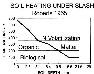
Fig. 3. Soil heating under slash piles (Adapted from Roberts, 1965).
