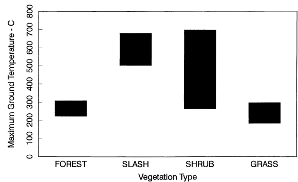
Fig. 2. Maximum ground temperatures during fires in forest, shrubland, and grassland ecosystems (Adapted from Rundel, 1983).
