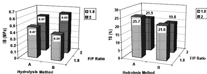
Figure 2 Effects of interaction between hydrolysis method and F/P ratio on internal bonding strength (IB) and percent thickness swell (TS) of southern pine fiberboard.
