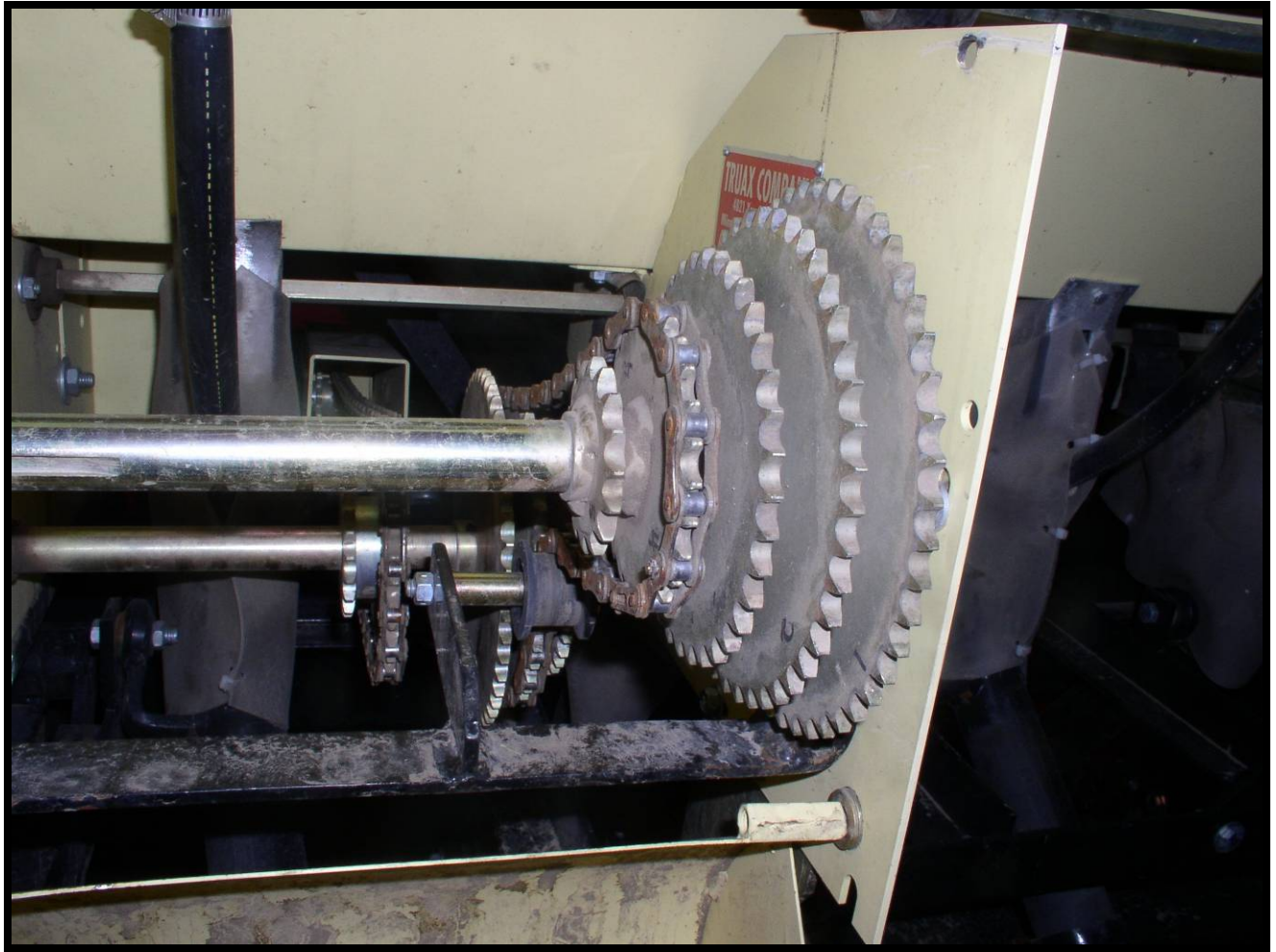
Figure 7. Derailleur controls for fluffy seed box. Moving the chain to the left increases seed output and moving the chain to the right decreases seed output.
