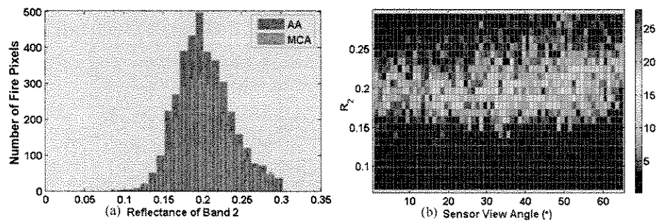
Fig. 3. The distribution of R_2 . (a) The histogram of R_2 . The distribution of fire pixels detected by the MODIS contextual algorithms is in brown (MCA). Blue is for fire pixels that only can be detected by the adjusted algorithm (AA). (b) The density distribution of all fire pixels (Group AA and MCA) with R_2 and the sensor view angle.
