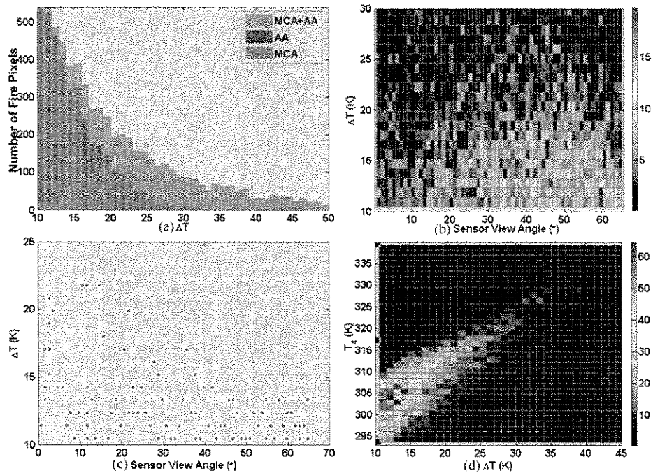
Fig. 5. The distribution of \Delta T . (a) The histogram of \Delta T . The distribution of fire pixels detected by the MODIS contextual algorithms (MCA) is in brown. Blue is for fire pixels that only can be detected by the adjusted algorithm (AA). All fire pixels from both groups are in grey. (b) The density distribution of all fire pixels with \Delta T and the sensor view angle. (c) The distribution of \Delta T for maximum fire density at all sensor view angles. (d) The density distribution of all fire pixels with \Delta T and T_1 .
