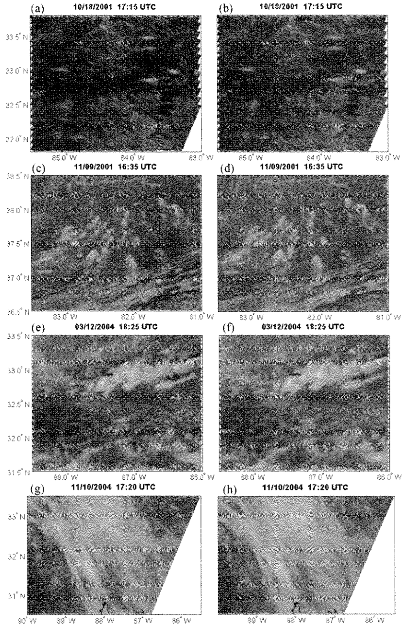
Fig. 2. Small fires detected by the adjusted algorithm and the MODIS contextual algorithm. Fires in left panels are detected by the adjusted algorithm, and fires in right panels are detected by the MODIS contextual algorithm.
