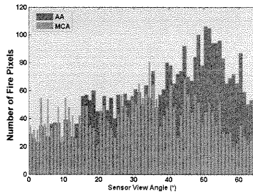
Fig. 6. The histogram of sensor view angles for fire pixels. The distribution of fire pixels detected by the MODIS contextual algorithms (MCA) is in brown. Blue is for fire pixels that only can be detected by the adjusted algorithm (AA).
