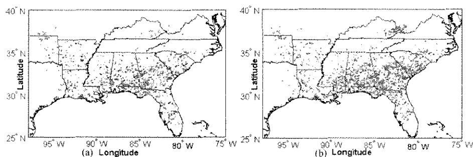
Fig. 1. Spatial distribution of the fire pixels. (a) Fire pixels detected by the MODIS contextual algorithm; (b) Fire pixels omitted by the MODIS contextual algorithm.
