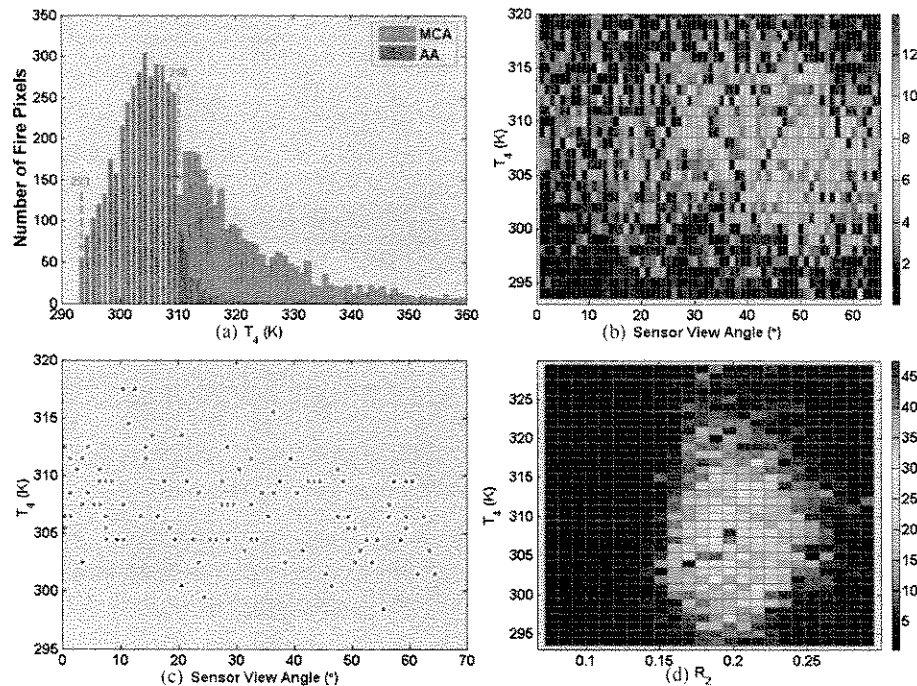
Fig. 4. The distribution of brightness temperature T_4 . (a) The histogram of T_4 . The distribution of the fire group MCA is in brown. Blue is for the fire group AA. (b) The density distribution of all fire pixels (Group AA and MCA) with T_4 and the sensor view angle. (c) The distribution of T_4 for maximum fire density at all sensor view angles. (d) The density distribution of all fire pixels with R_2 and T_4 .
