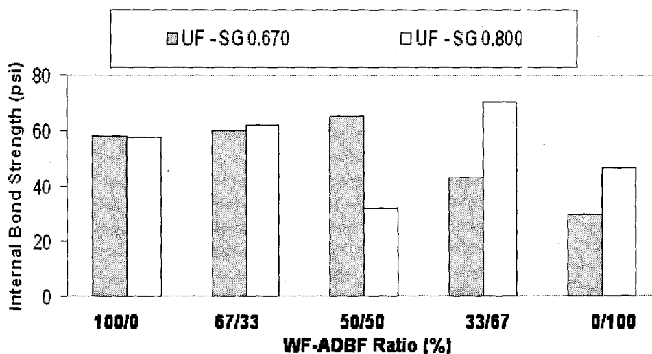
Figure 4. Effects of various WF and ADBF fiber mixtures and fiberboard density on internal bond strength (IB)
