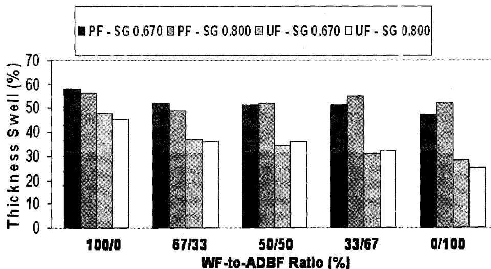
Figure 5. Effects of various WF and ADBF fiber mixtures and fiberboard density on thickness swell (TS) after 24-hr soak
