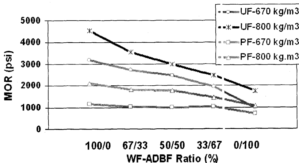
Figure 3. Effects of various WF and ADBF fiber mixtures and fiberboard density on Modulus of Rupture (MOR)
