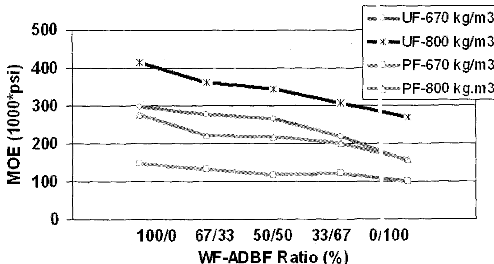
Figure 2. Effects of various WF and ADBF fiber mixtures and fiberboard density on Modulus of Elasticity (MOE)
