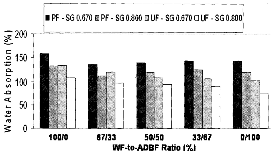
Figure 6. Effects of various WF and ADBF fiber mixtures and fiberboard density on water absorption (WA) after 24-hr soak
