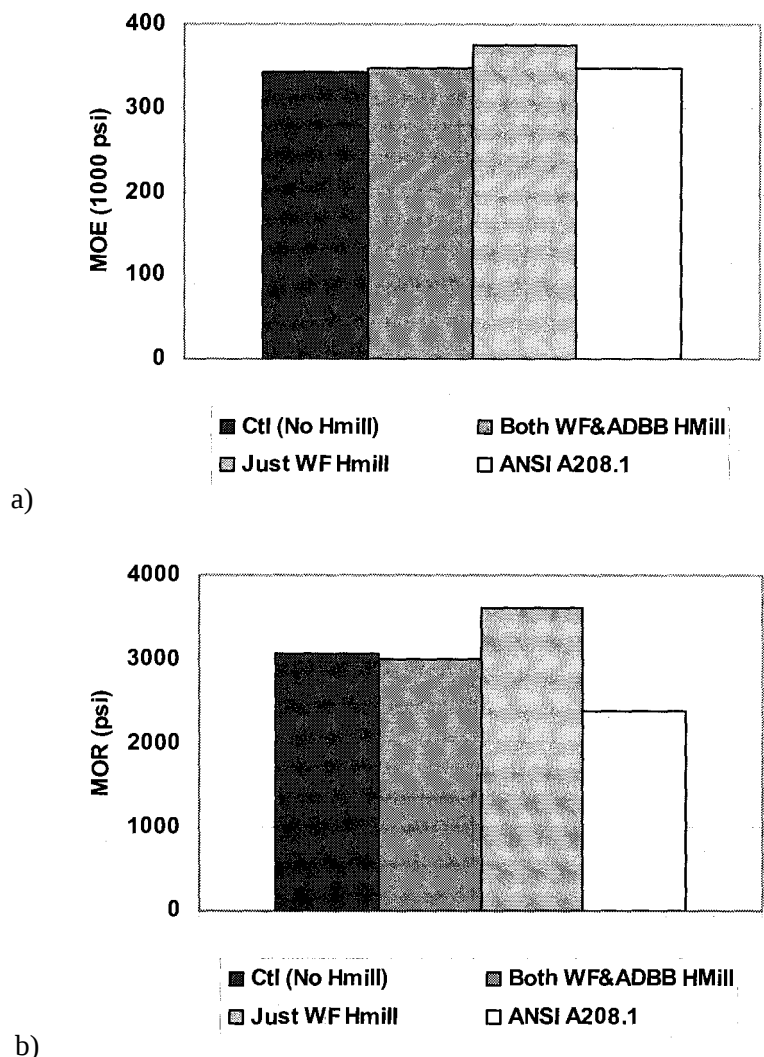
Figure 1. Effects of pre-process hammermilling of fiber on a) Modulus of Elasticity (MOE) and b) bending strength (MOR) of 50/50% hybrid wood-ADBF dry-formed fiberboard compared to commercial H-1 grade particleboard requirements.
