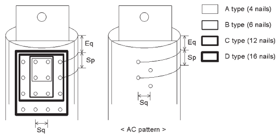
Figure 2. Nail patterns for power-driven nail connection.
