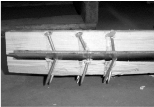
Figure 6. Mode III nail bending failure.
