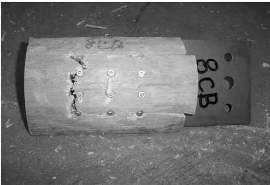
Figure 7. Block shear failures.
